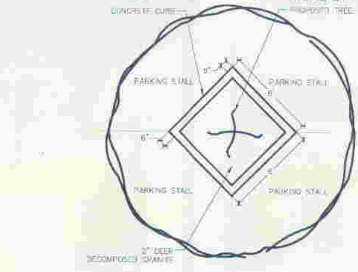
A DETAIL AT PLANTER NO SCALE
