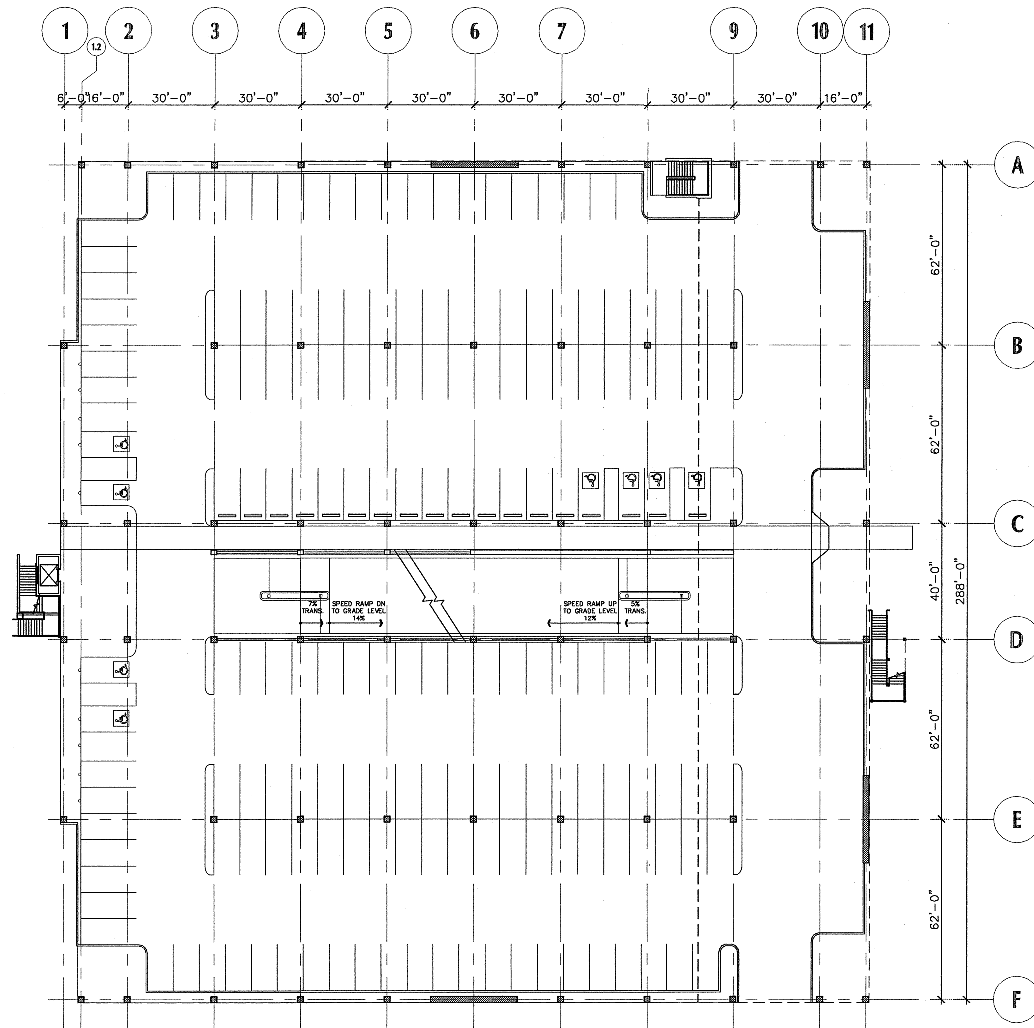
GRADE LEVEL 179 PARKING SPACES 80,658 SF
