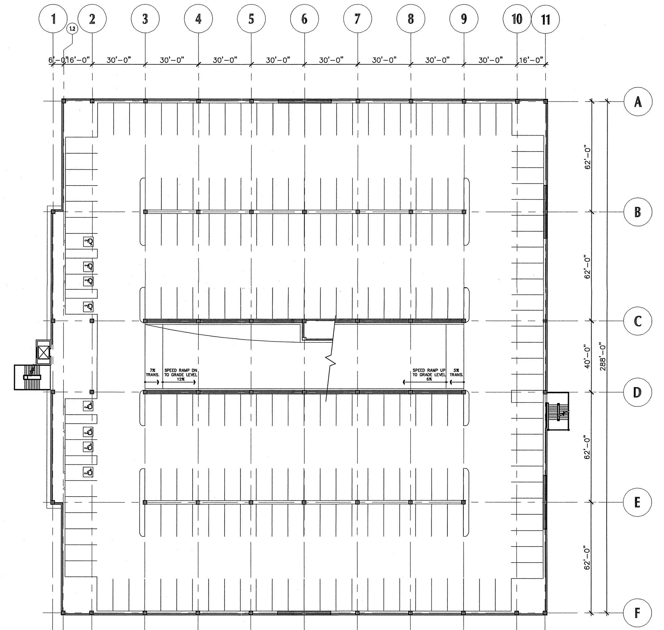
SECOND LEVEL 219 PARKING SPACES 80,646 SF
