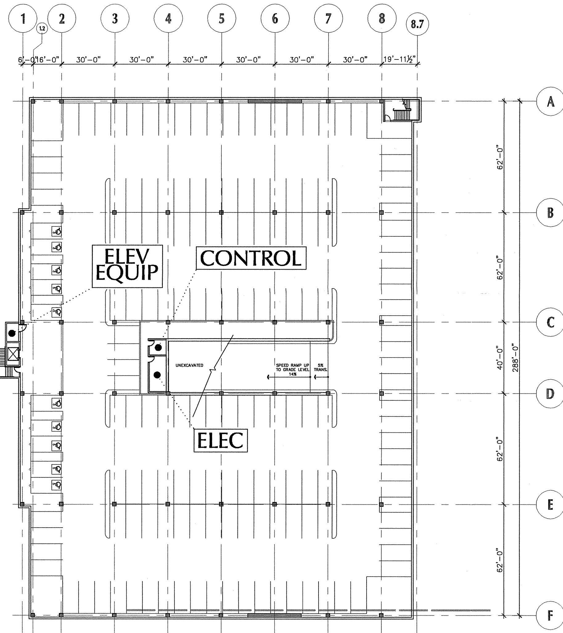
BASEMENT LEVEL 168 PARKING SPACES 64,206 SF
