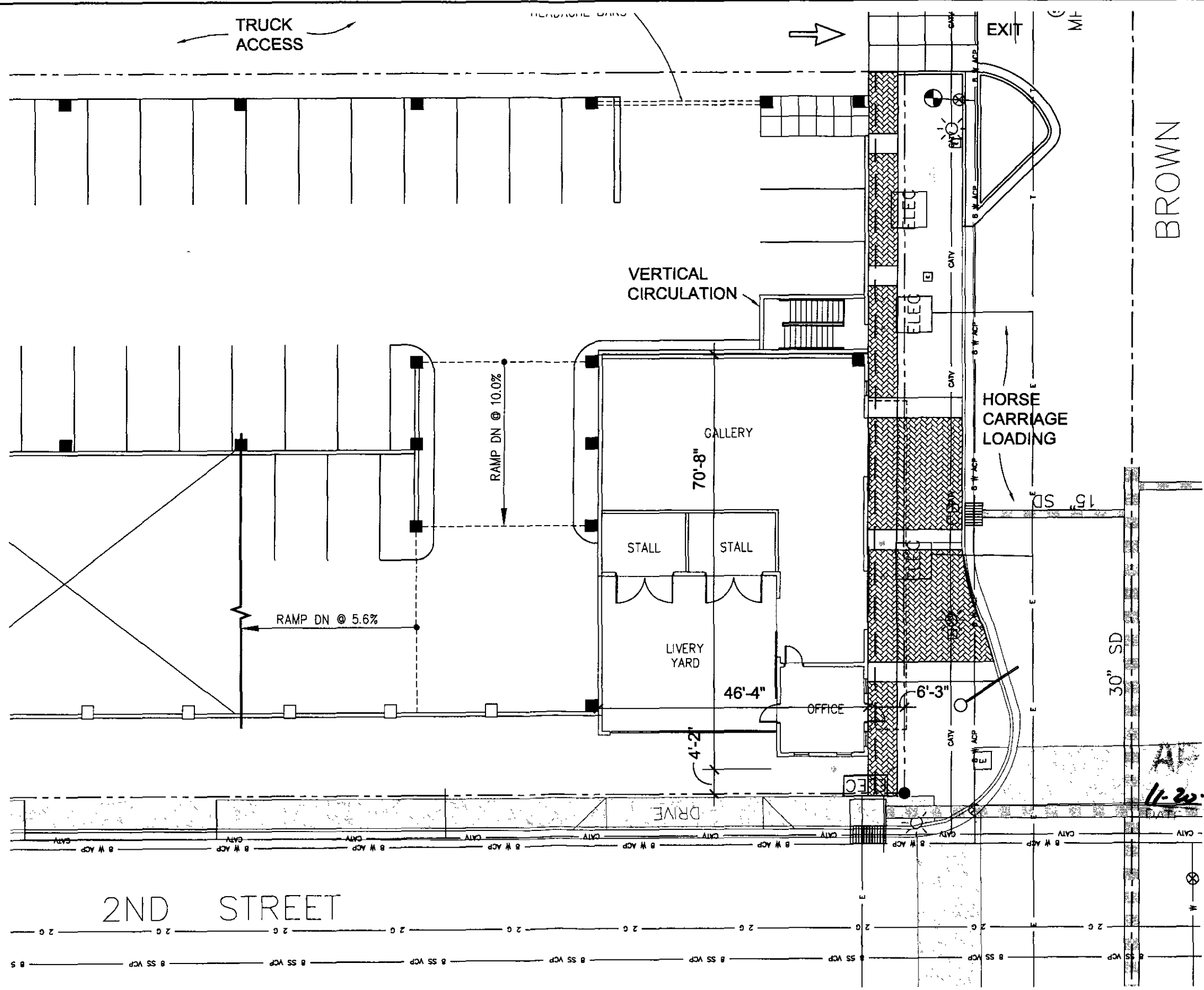
A SITE PLAN - LIVERY 1/8" = 1'-0"
