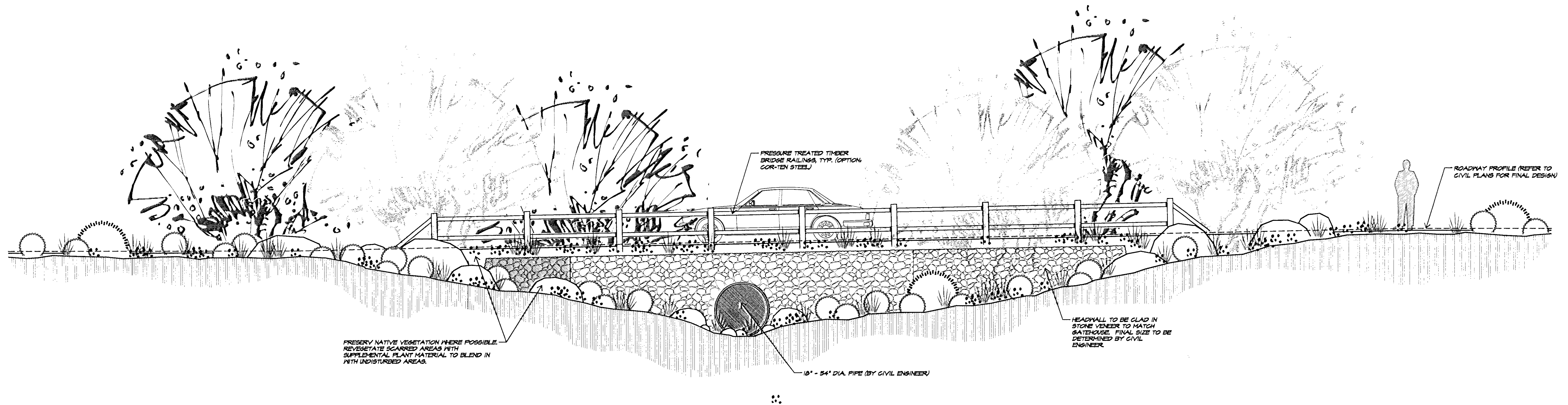
WASH CROSSING / HEADWALL TREATMENT
