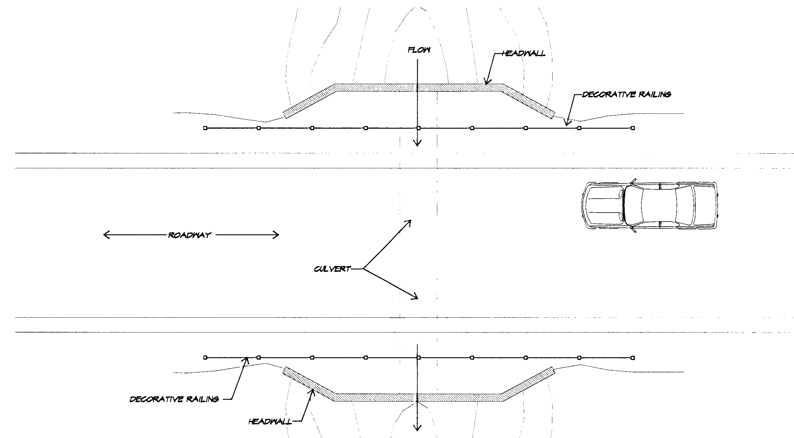
WASH CROSSING / HEADWALL TREATMENT (PLAN VIEW)
