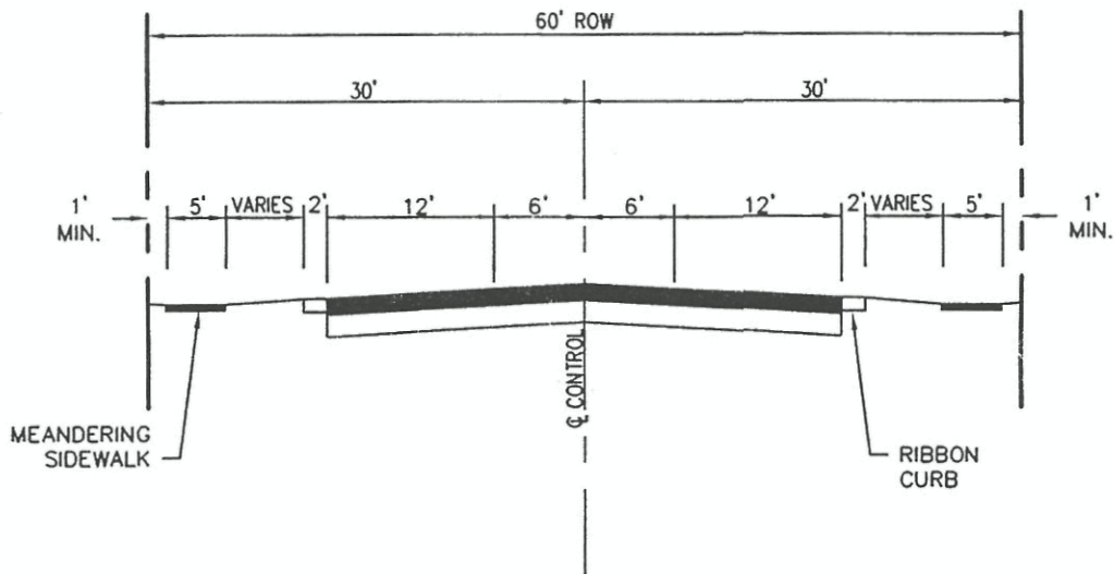
PUBLIC ROADWAY - MINOR COLLECTOR ULTIMATE ROADWAY CROSS-SECTION
