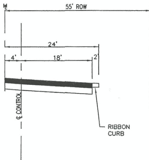
PROPOSED 128th STREET - MINOR COLLECTOR INTERIM ROADWAY CROSS-SECTION
