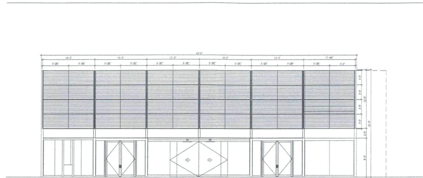
WEST - CANOPY ELEVATION SCALE: 1/4" = 1'-0"
