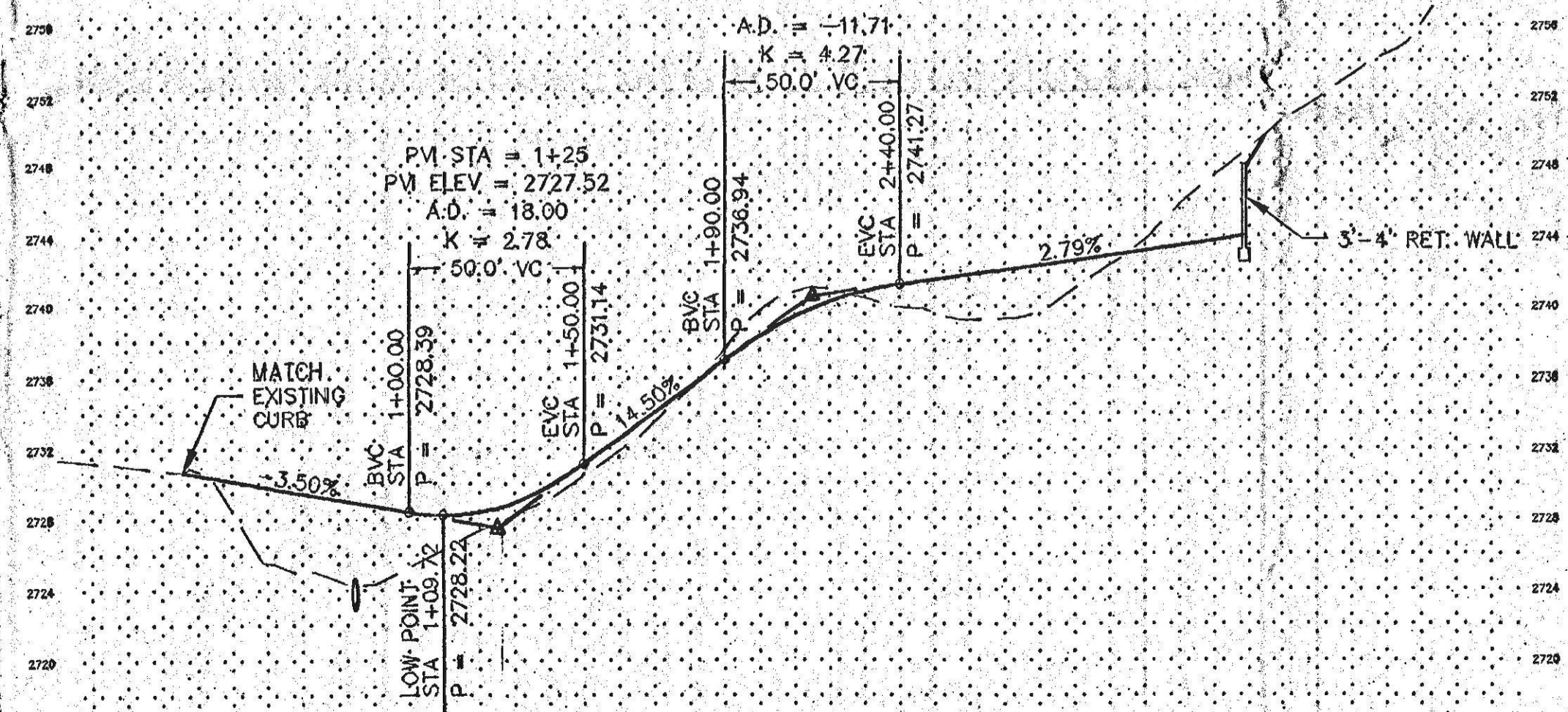
DRIVEWAY PROFILE
