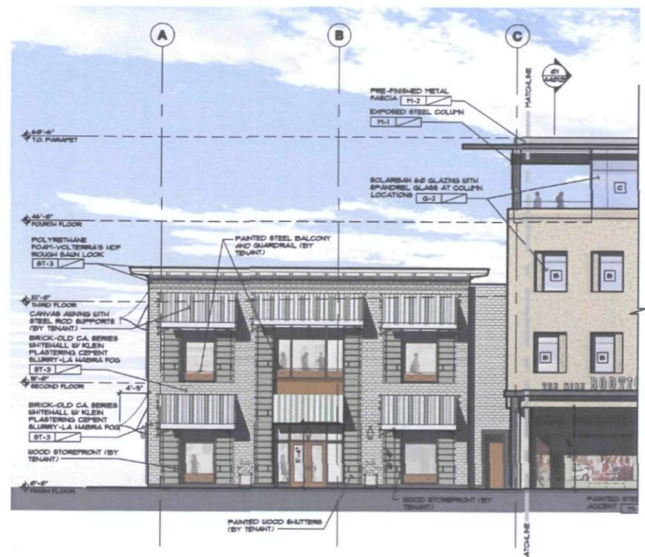
BUILDING B PARTIAL WEST ELEVATION - 01 SCALE: 3/32" = 1'-0" REF:
