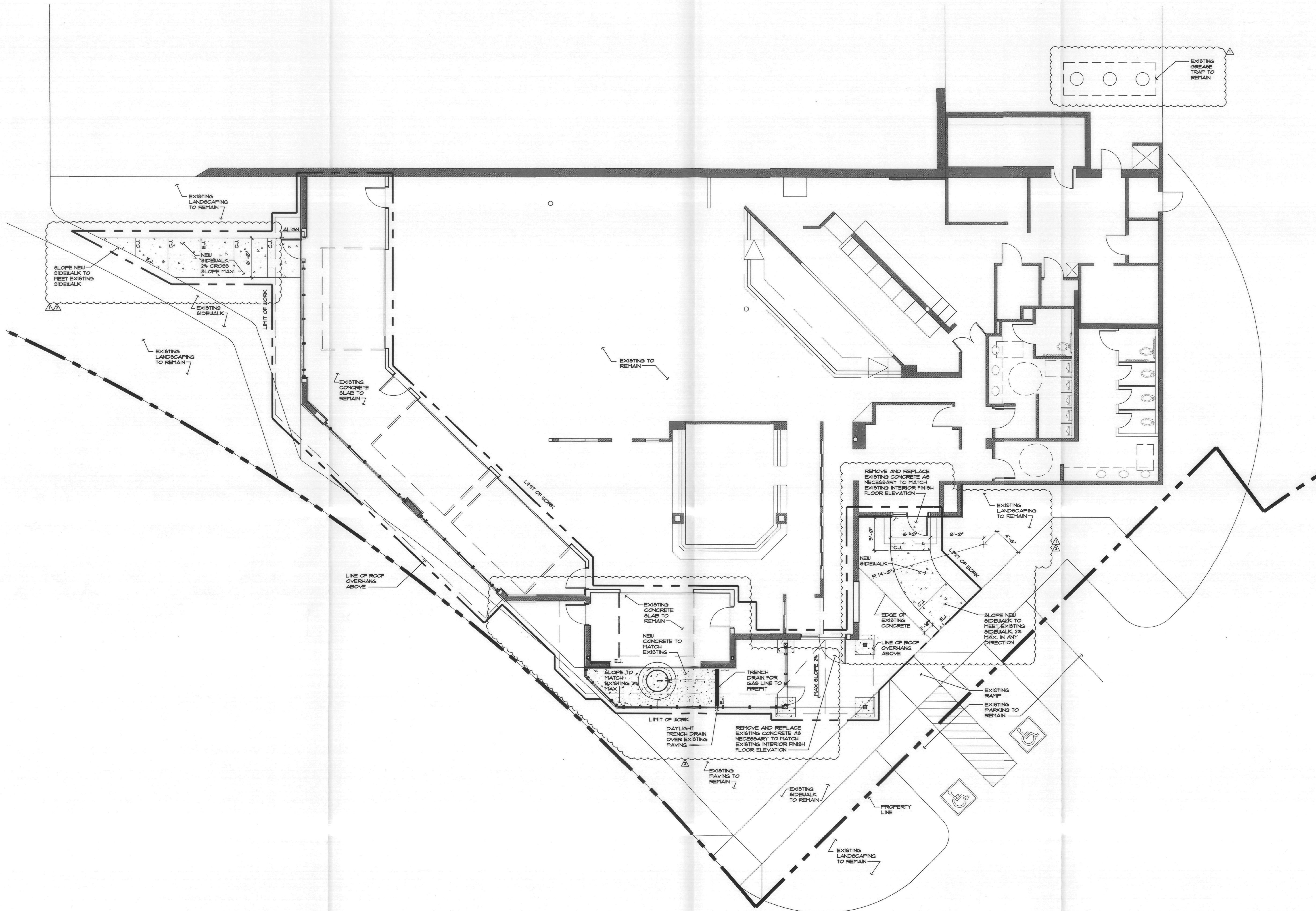
01 SITE PLAN SCALE: 3/16" = 1'-0"
