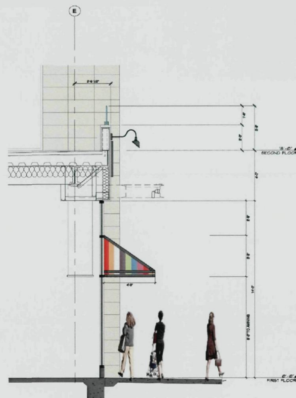
STOREFRONT/ CANOPY SECTION SCALE: 1'-0" = 3/8"
