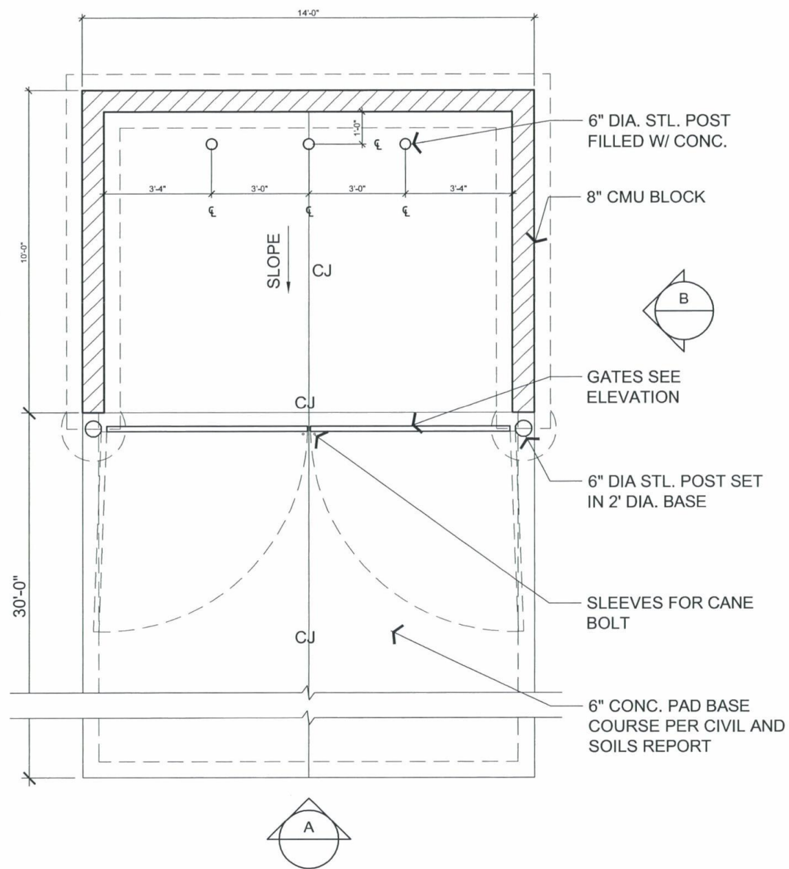
REFUSE ENCLOSURE TYPICAL PLAN SCALE: 1/4" = 1'-0"
