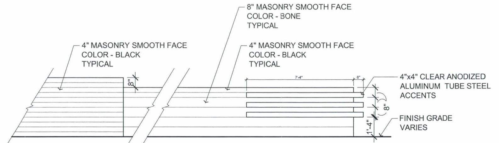
TYPICAL RETAINING WALL ELEVATION SCALE: 1/4" = 1'-0"
