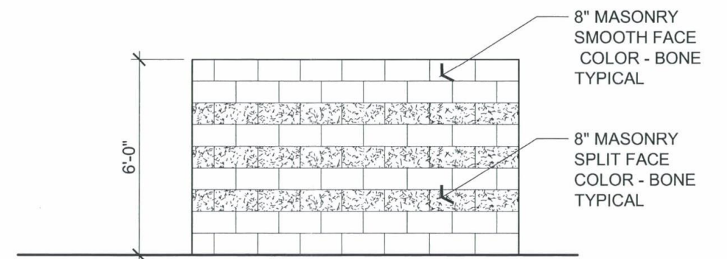
REFUSE ENCLOSURE ELEVATION B SCALE: 1/4" = 1'-0"
