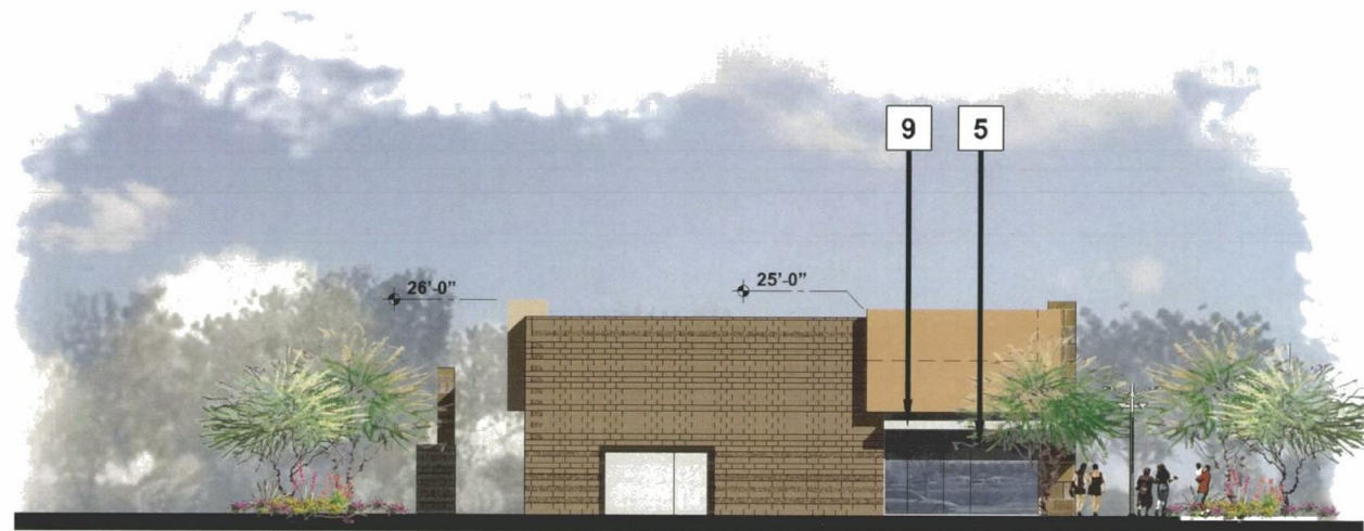
South Elevation
