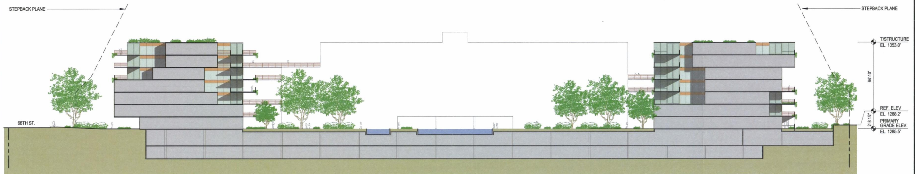
EAST - WEST SECTION
