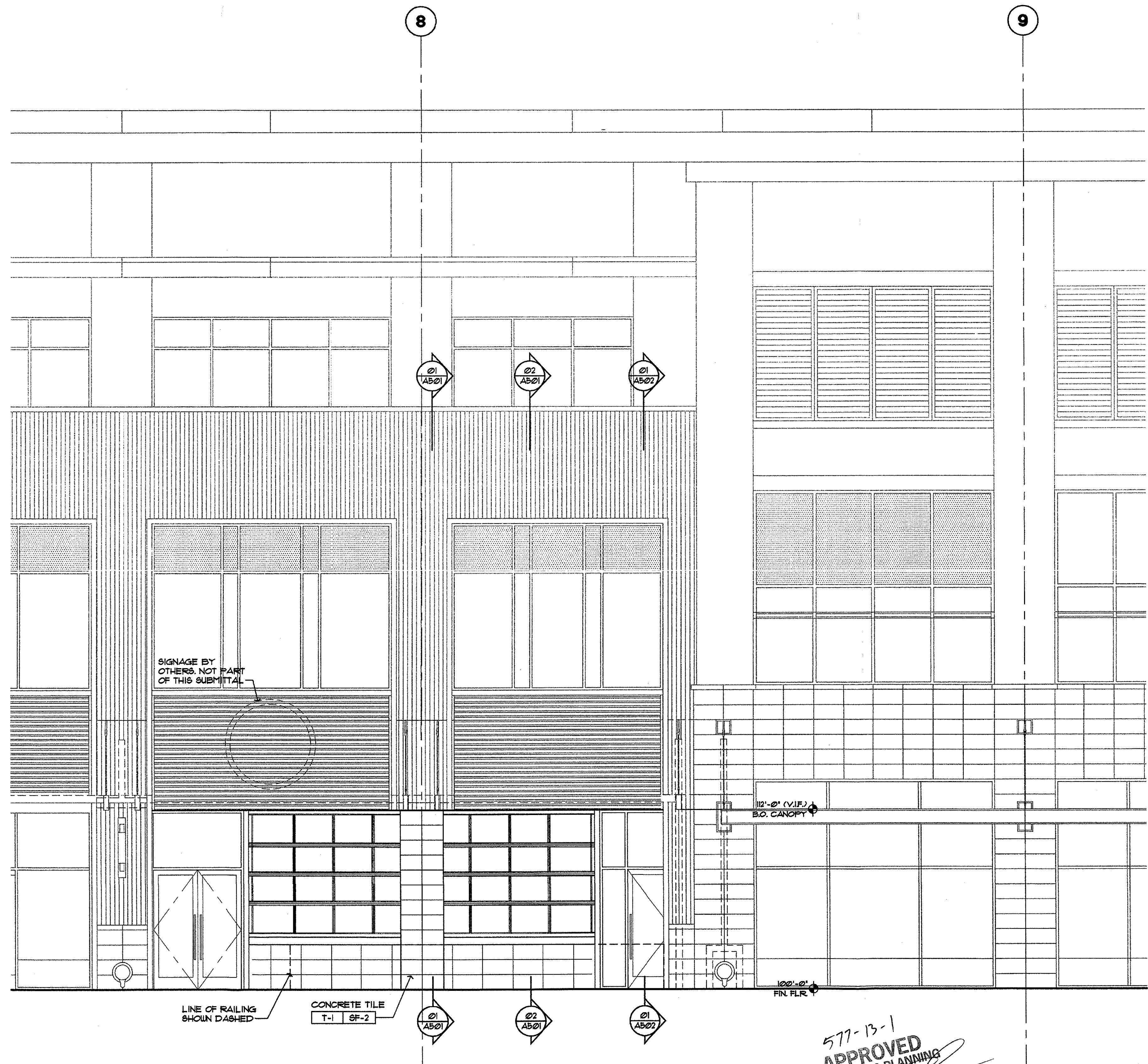
01 BUILDING ELEVATION SCALE: 1/4"=1'-0" REF: 01/A201
