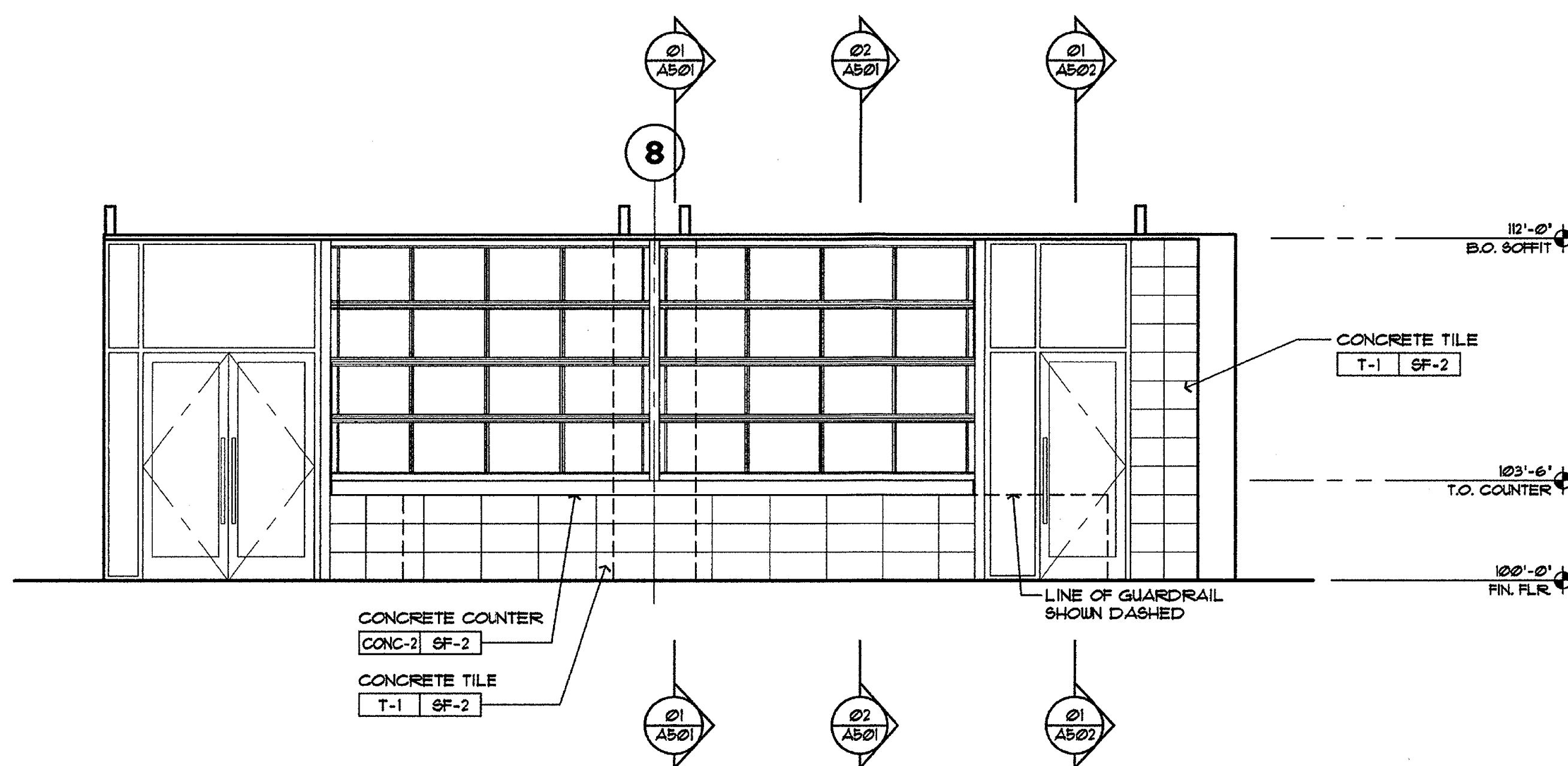
04 PATIO ELEVATION SCALE: 1/4"=1'-0" REF: 01/A201
