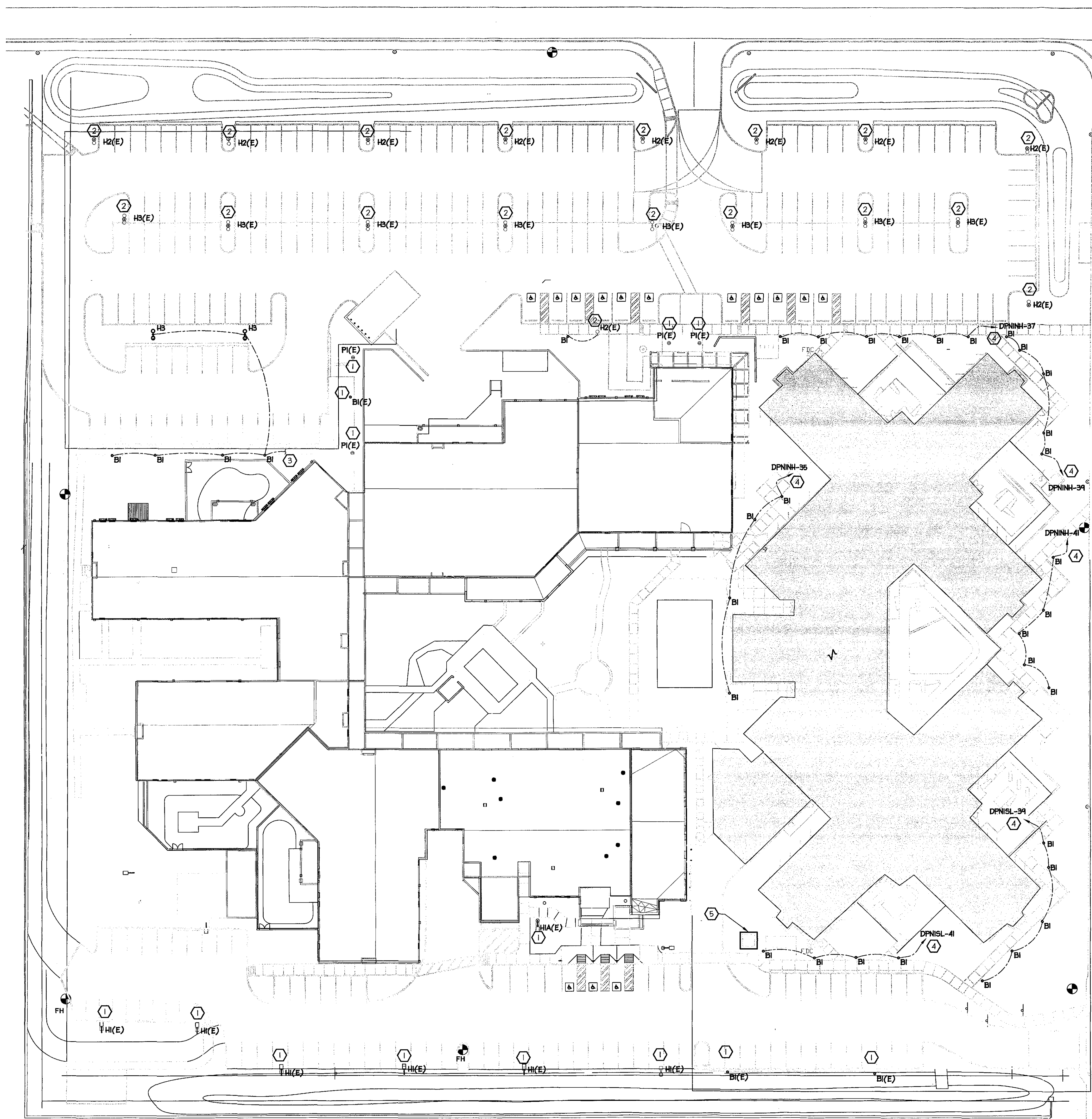
NORTH SITE LIGHTING PLAN SCALE: 1" = 30'-0"
