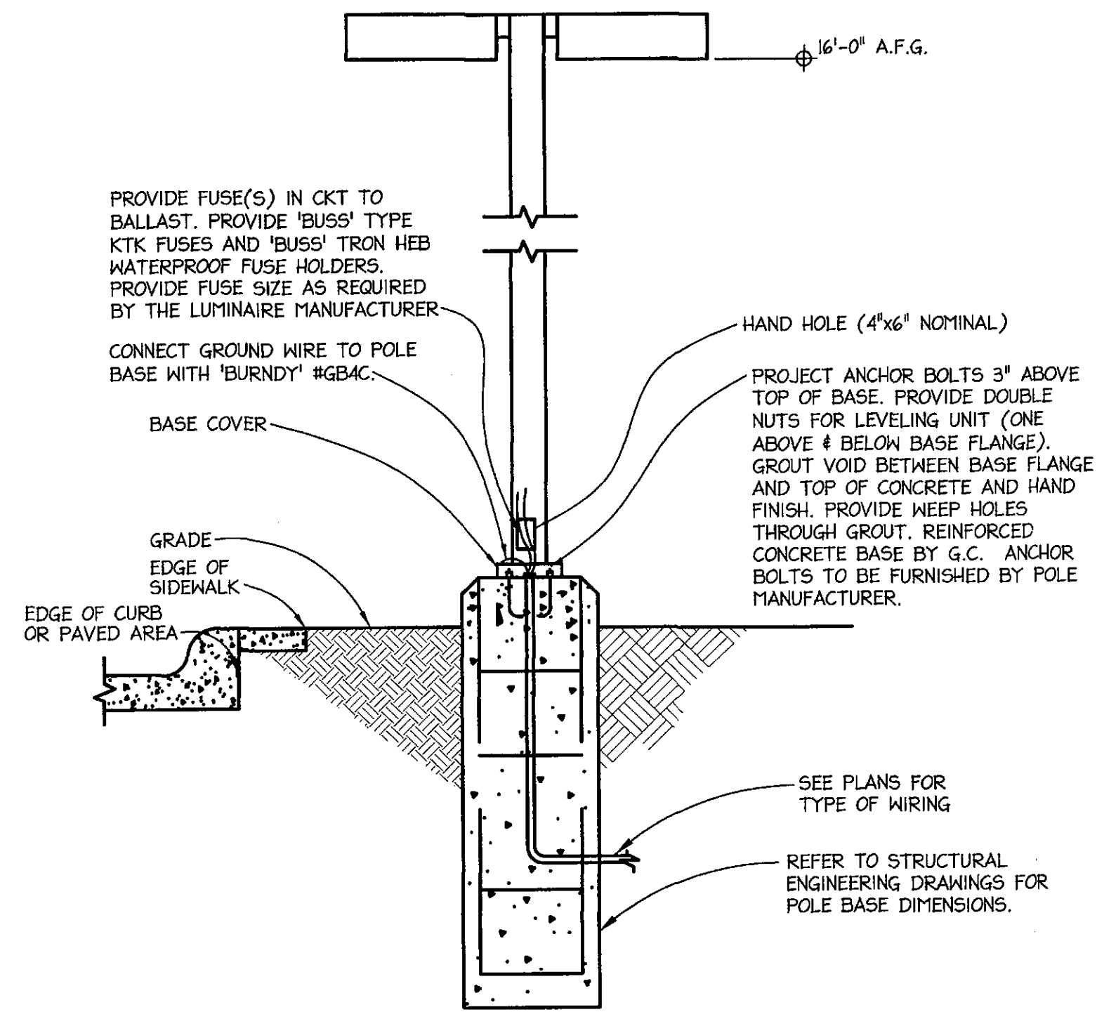
POLE BASE DETAIL NOT TO SCALE
