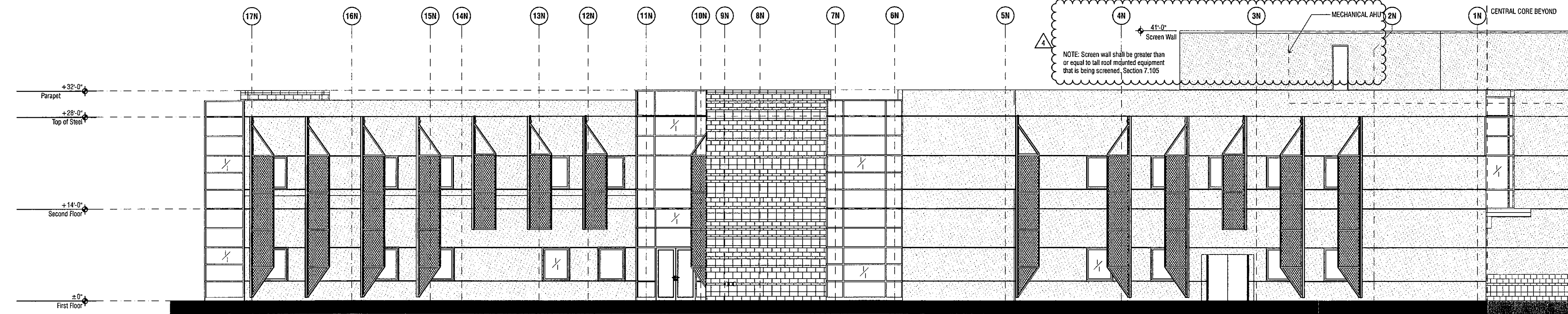
7B BLDG N NORTHWEST ELEVATION SCALE: 1/8" = 1'-0" 0 4 8 16'
