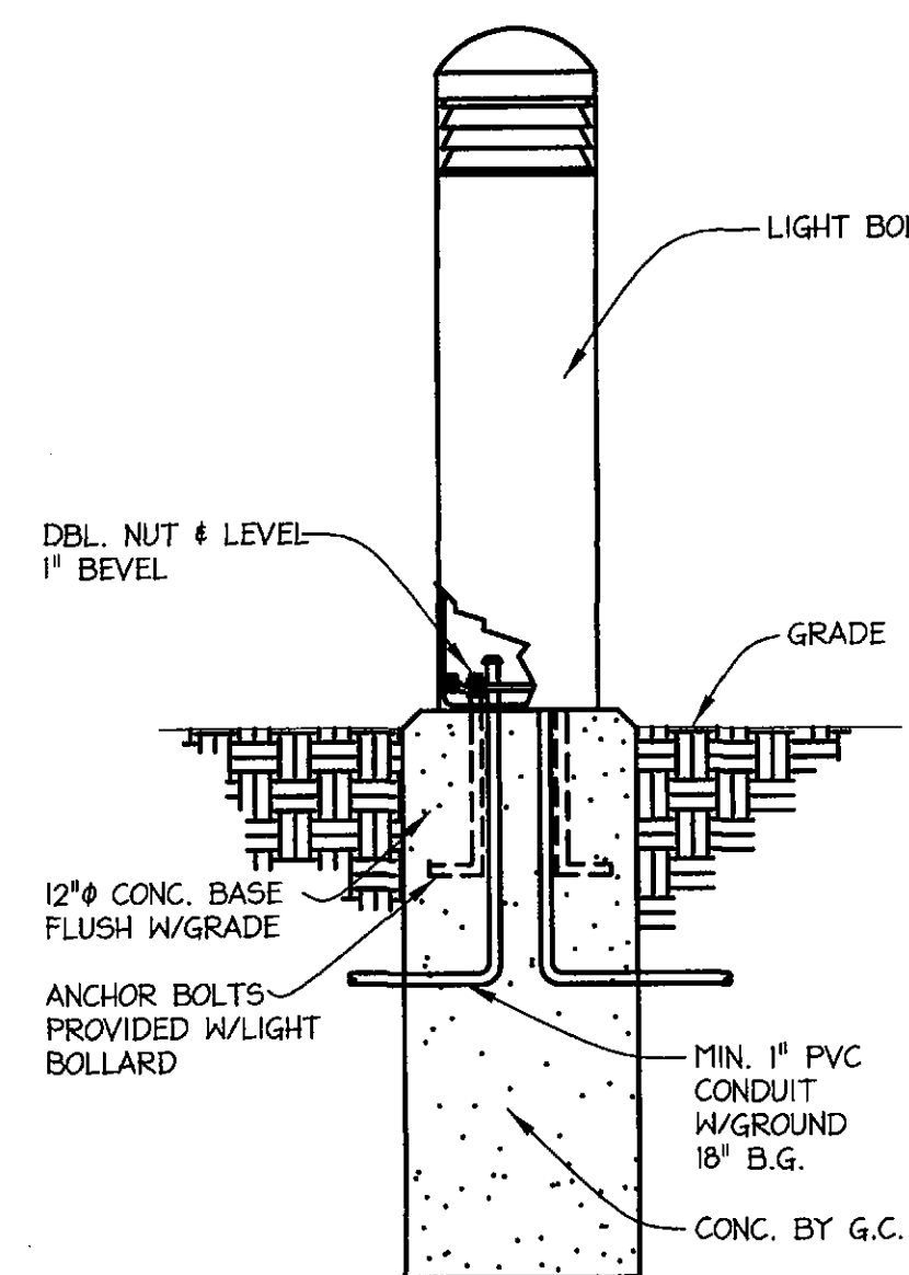
LIGHT BOLLARD BASE DETAIL NOT TO SCALE
