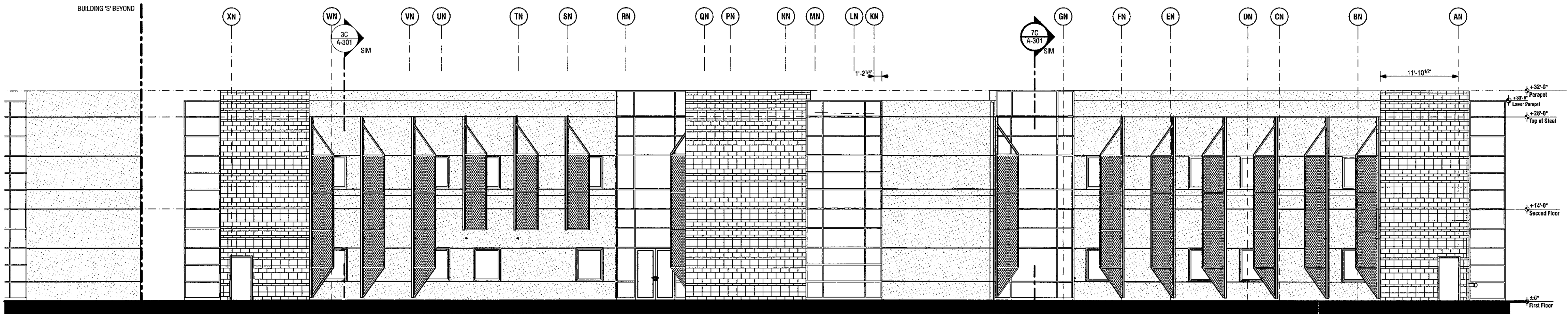
7C BLDG N NORTHEAST ELEVATION SCALE: 1/8" = 1'-0" 0 4 8 16'
