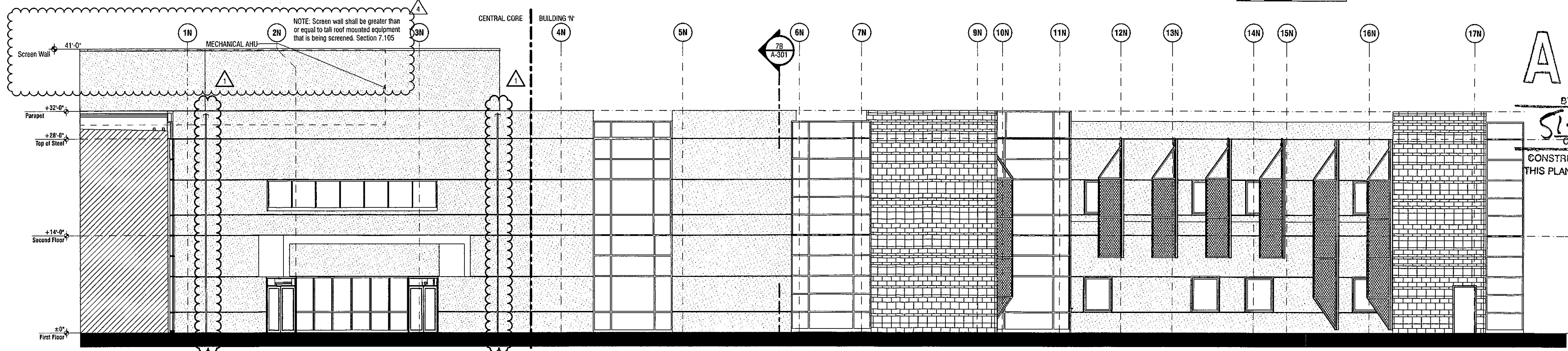
7D BLDG N SOUTHEAST ELEVATION SCALE: 1/8" = 1'-0" 0 4 8 16'
