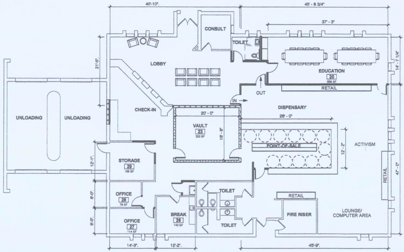
1 SPACE PLAN OPC 3/32" = 1'-0"
