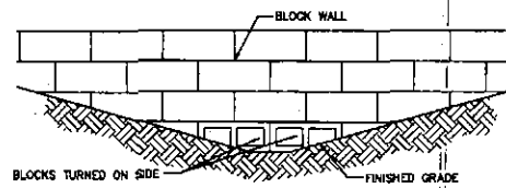
DRAINAGE BLOCKS DETAIL N.T.S.
