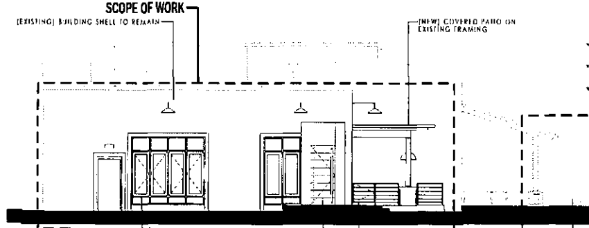
EAST ELEVATION SCALE: 3/16" = 1'-0"
