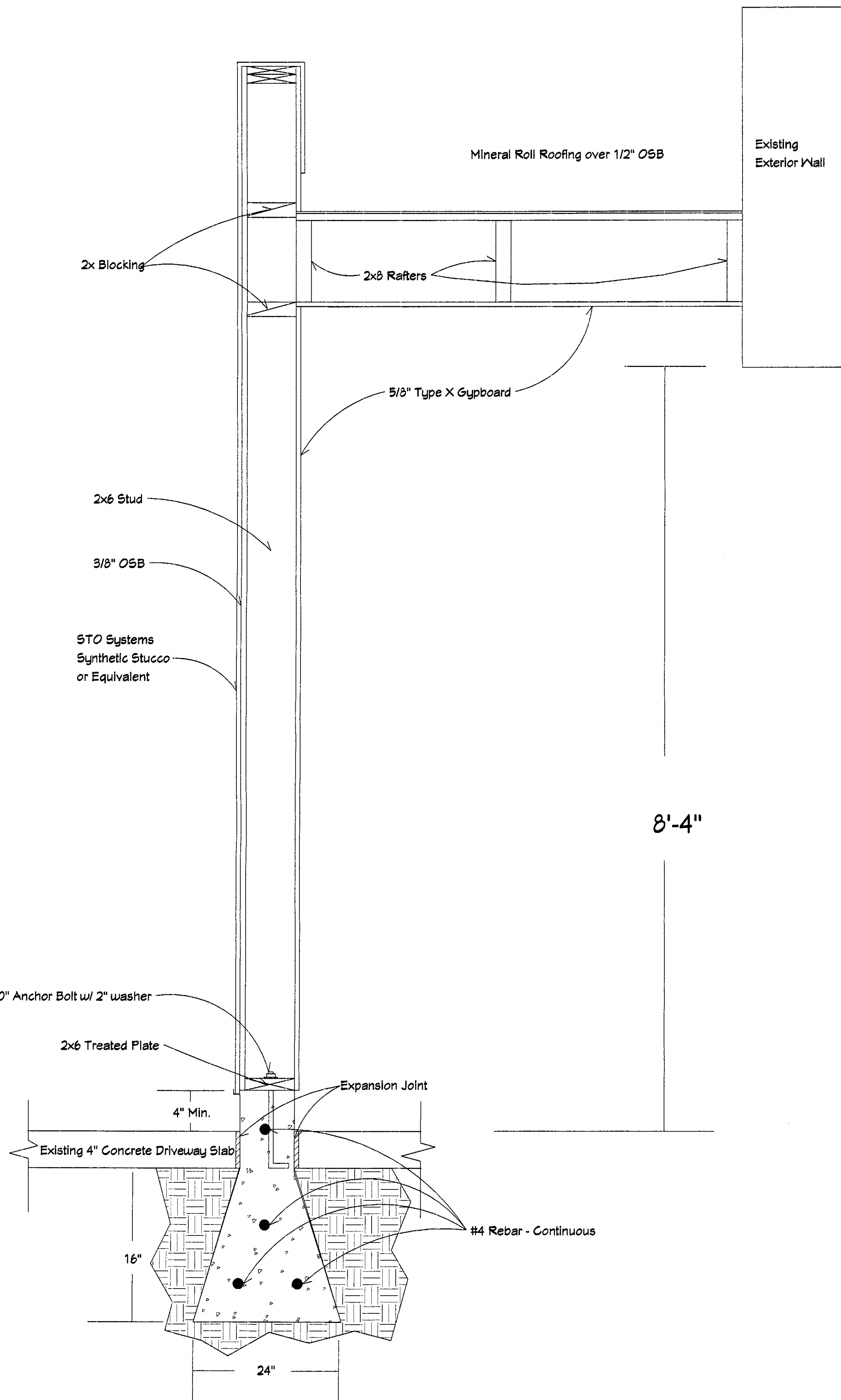
Cross Section Detail
