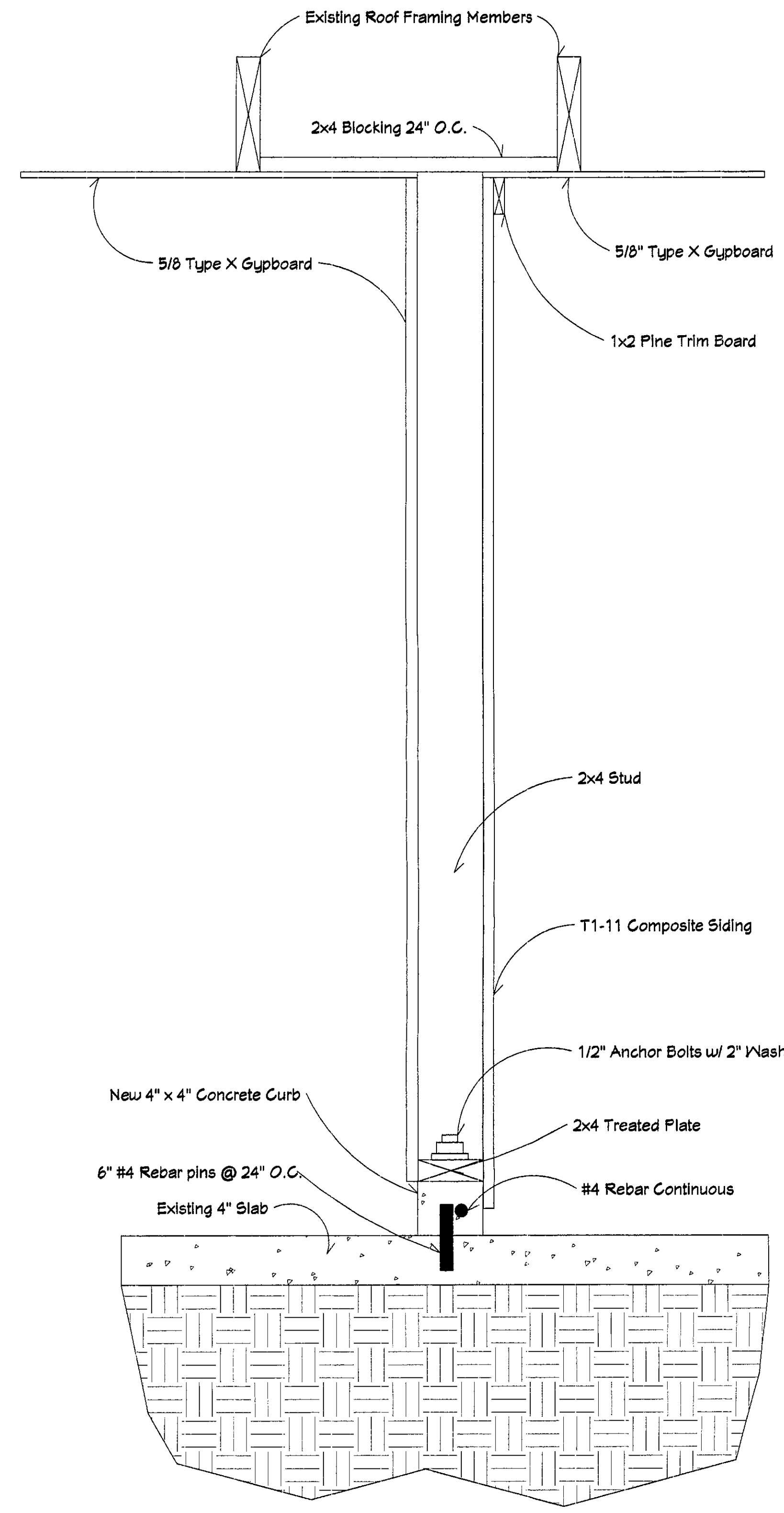
Cross Section Detail
