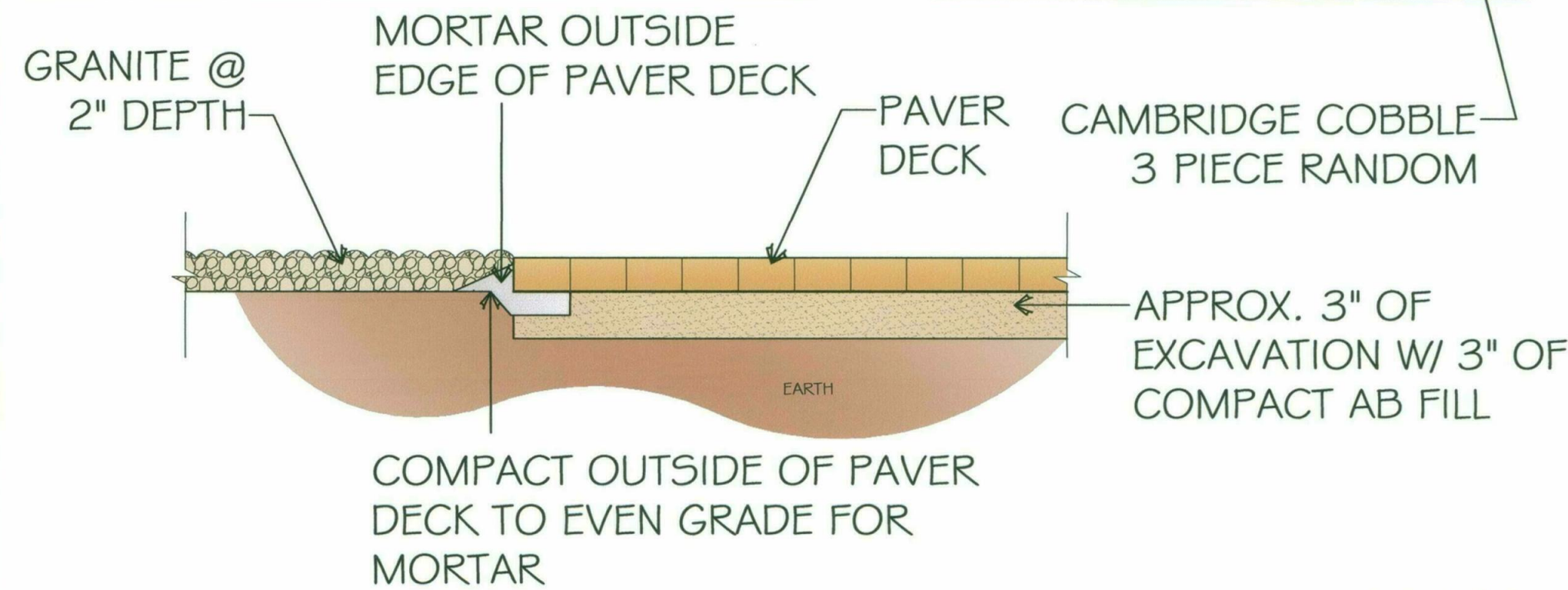
(F) PAVER DECK DETAIL
