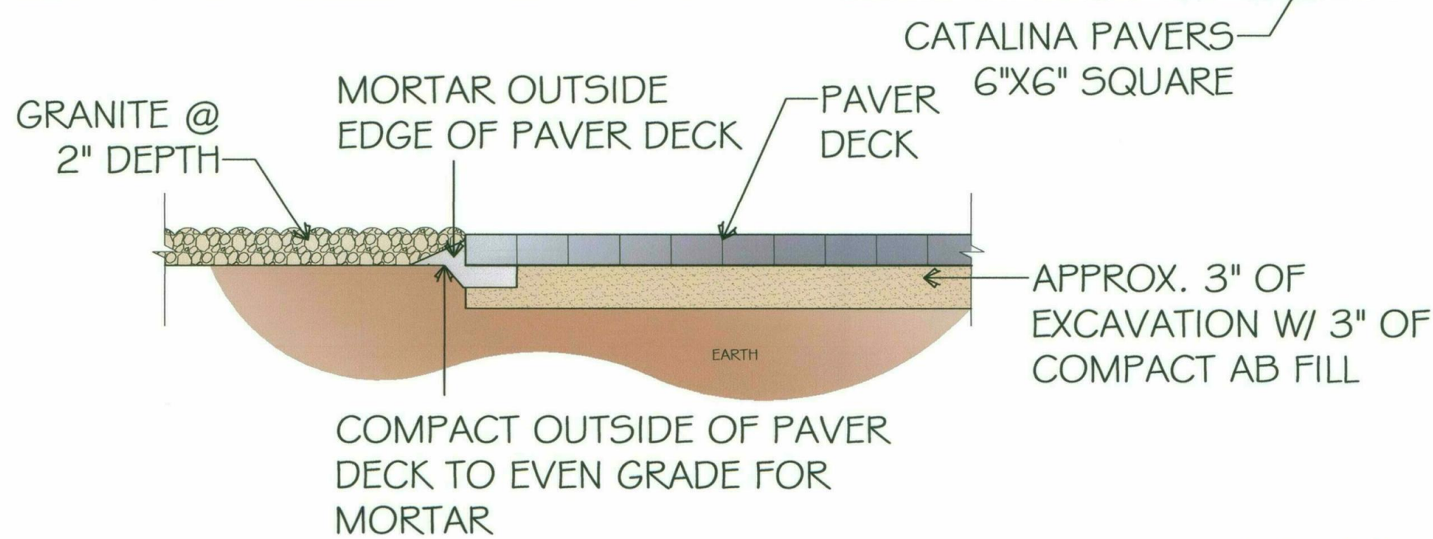
(E) PAVER DECK DETAIL
