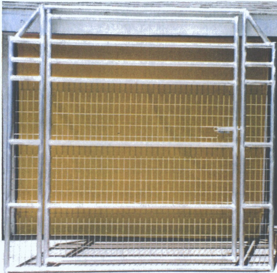
Main Entry/Exit Gate for Horses. 7 ft. Tall, 8 ft. Long. 1 7/8" pipe frame work, welded 360 degrees. Welded wire is 6 ft. tall, and welded to pipe framework. Gate opening is approximately 6 ft. wide by 8 ft. tall.
