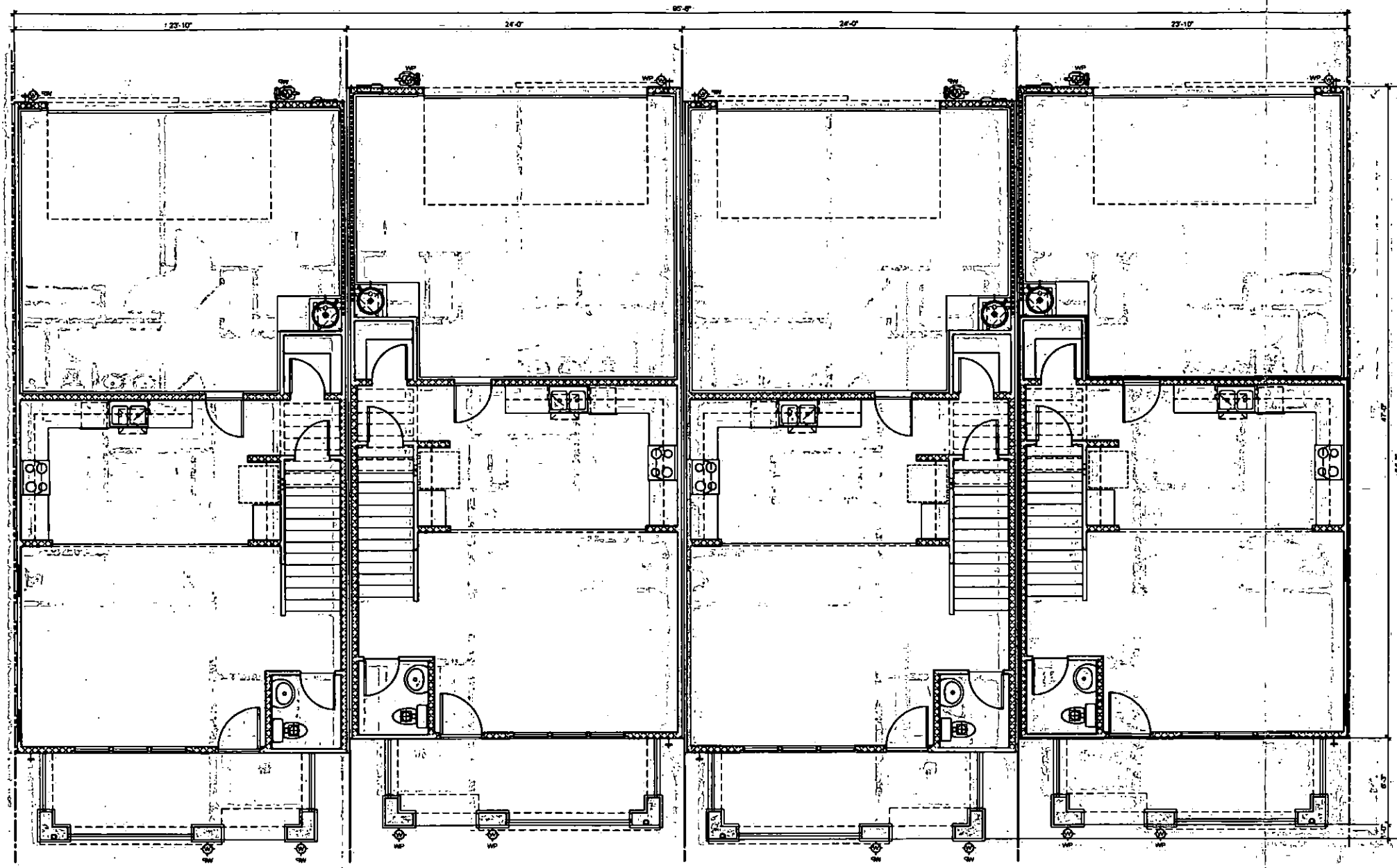
1st Floor Building Plan - 4 Plex 1/4" = 1'-0"
