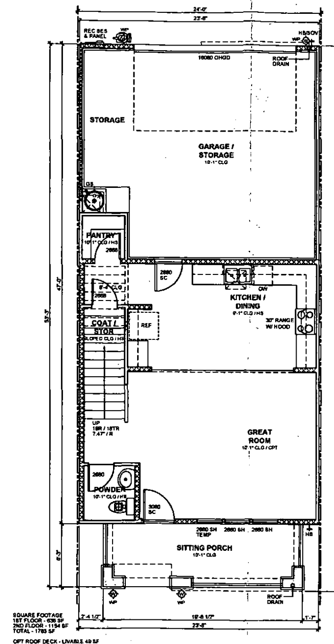
1st Floor Plan 1/4" = 1'-0"
