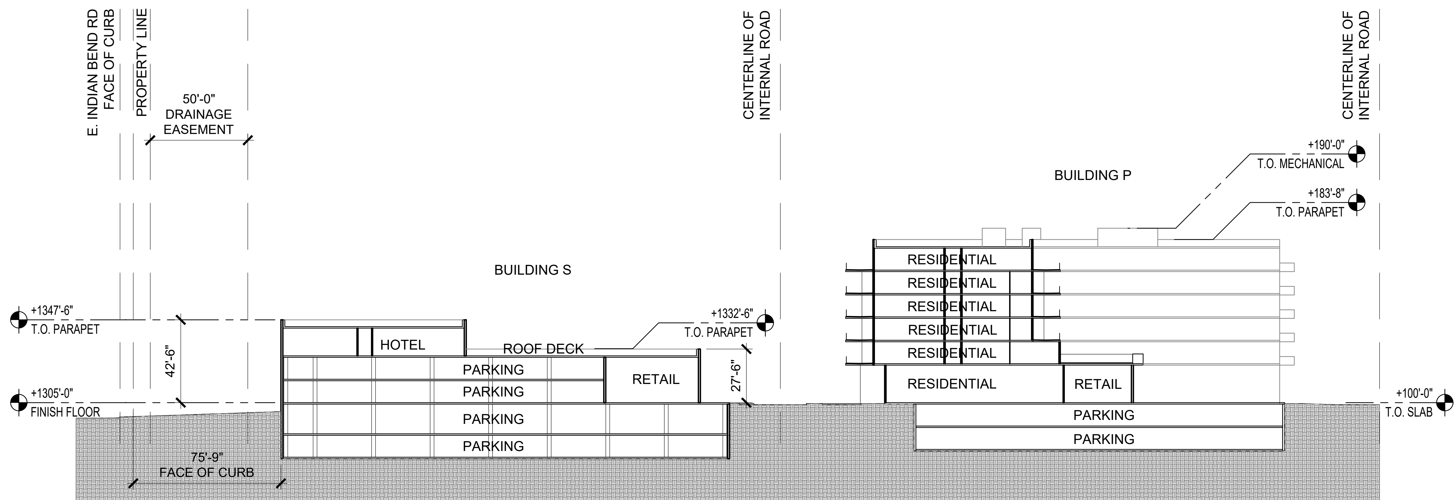
01 SITE SECTION - NORTH/SOUTH (LOOKING EAST) SCALE: 1"=30' REF:
