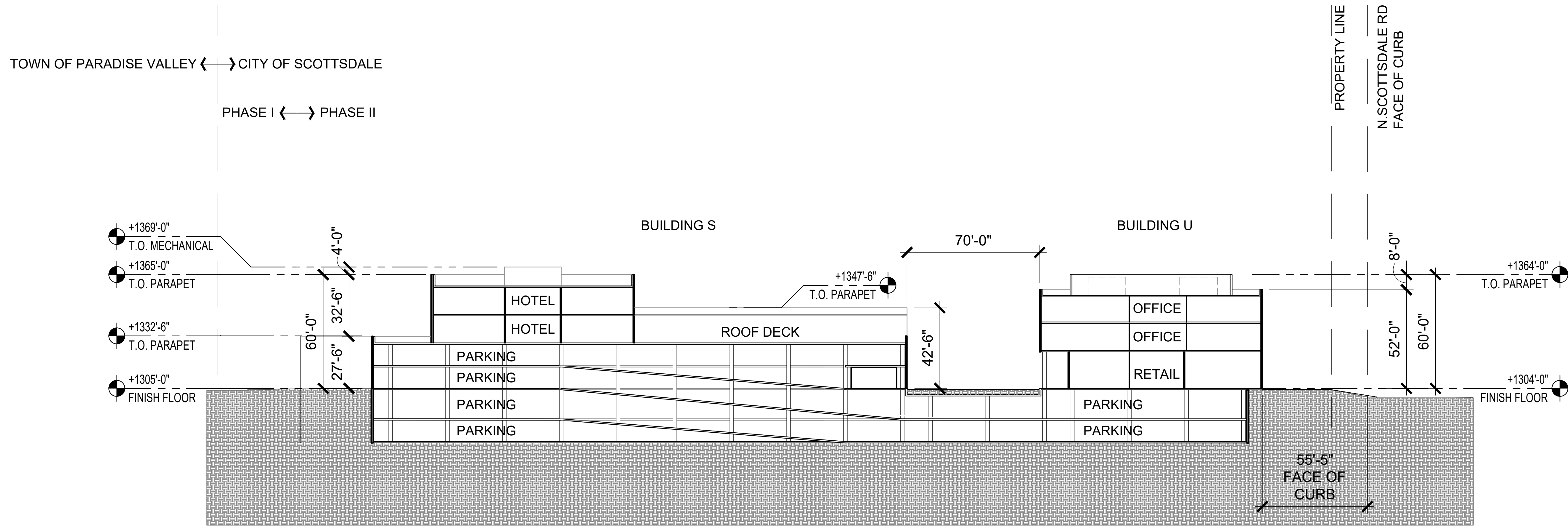
02 SITE SECTION - EAST/WEST (LOOKING NORTH) SCALE: 1"=30' REF:
