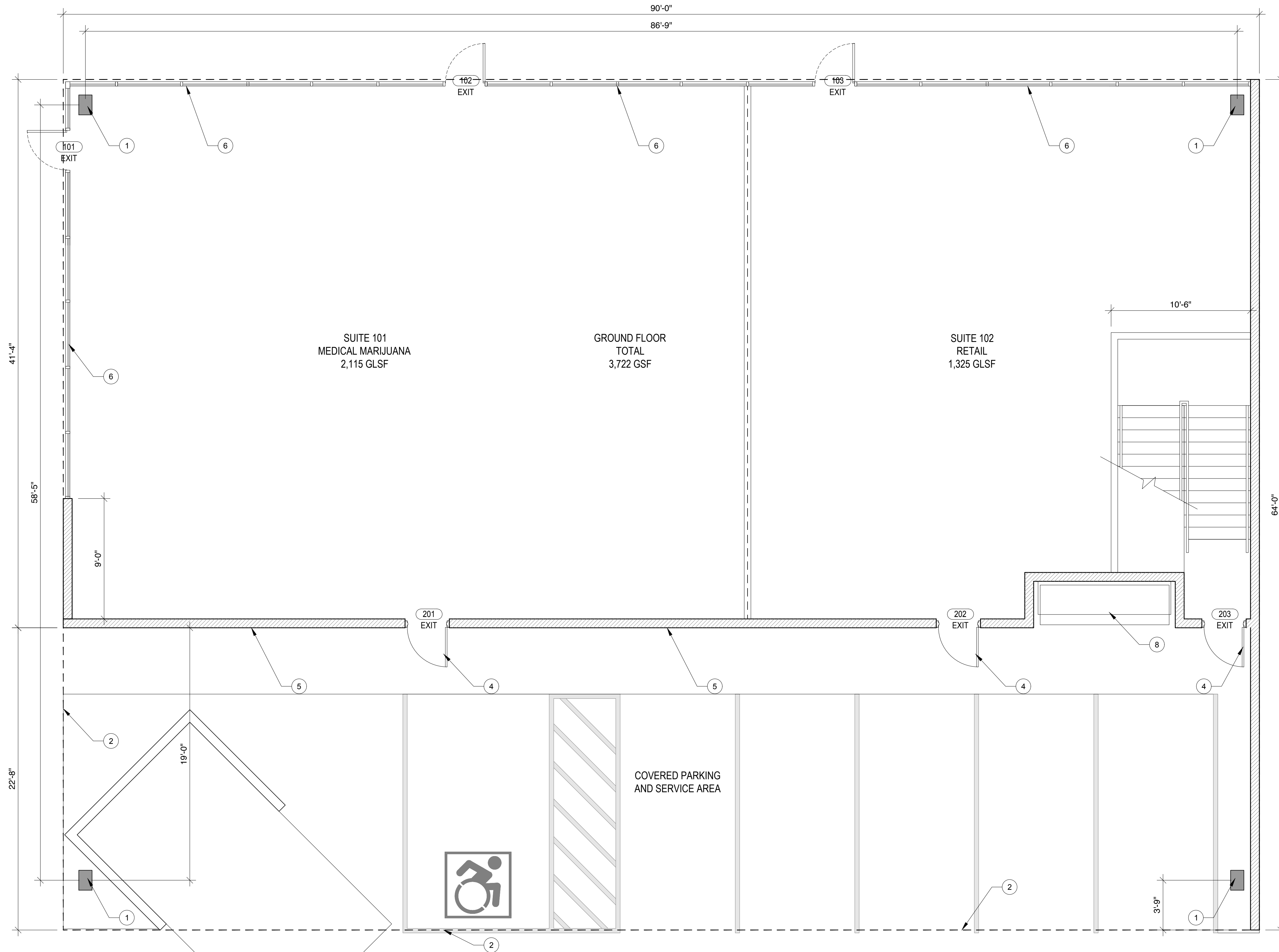
1 FLOOR PLAN - FIRST FLOOR 1/4" = 1'-0"
