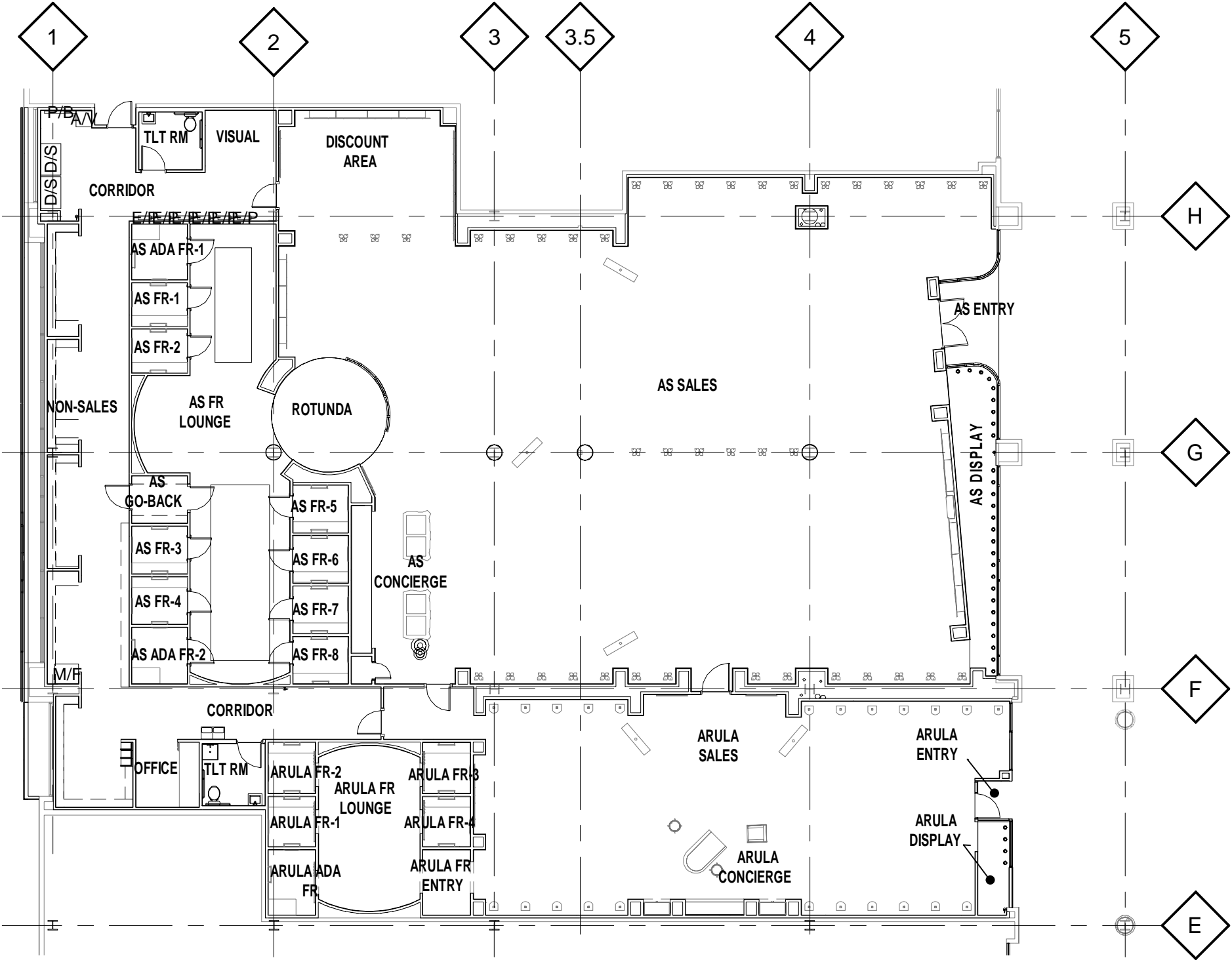
ALTAR'D STATE / ARULA FLOOR PLAN
