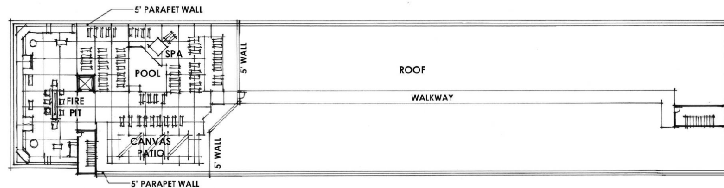
ROOF PLAN SCALE: 1/20"=1'-0"
