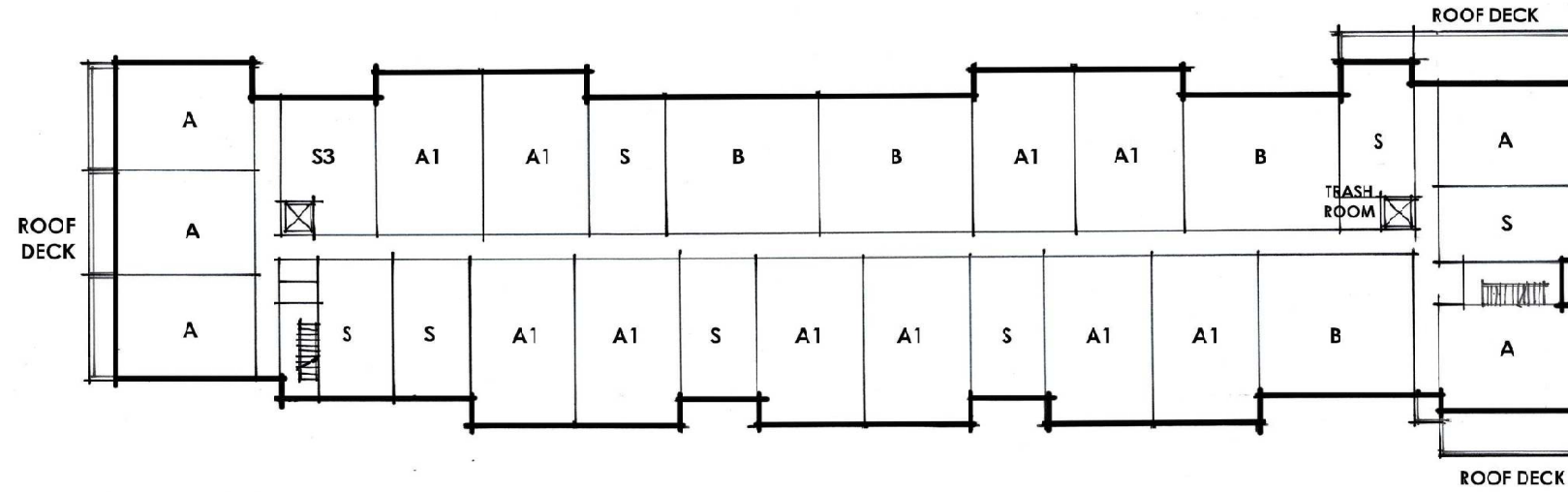
6TH FLOOR PLAN SCALE: 1/20"=1'-0"
