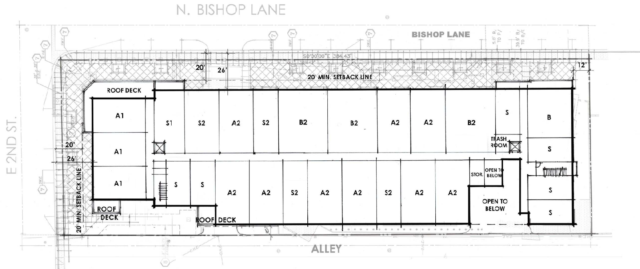
2ND FLOOR PLAN SCALE: 1/20"=1'-0"
