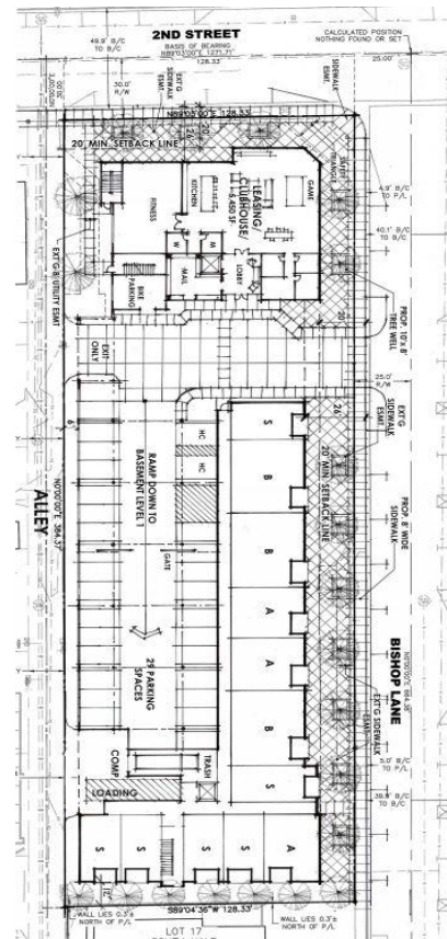
Figure 2 - Site Plan
