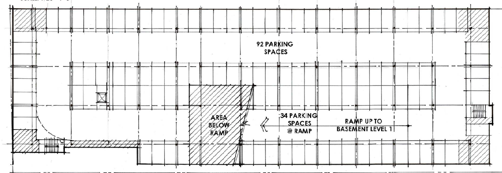
BASEMENT LEVEL 2 PLAN
