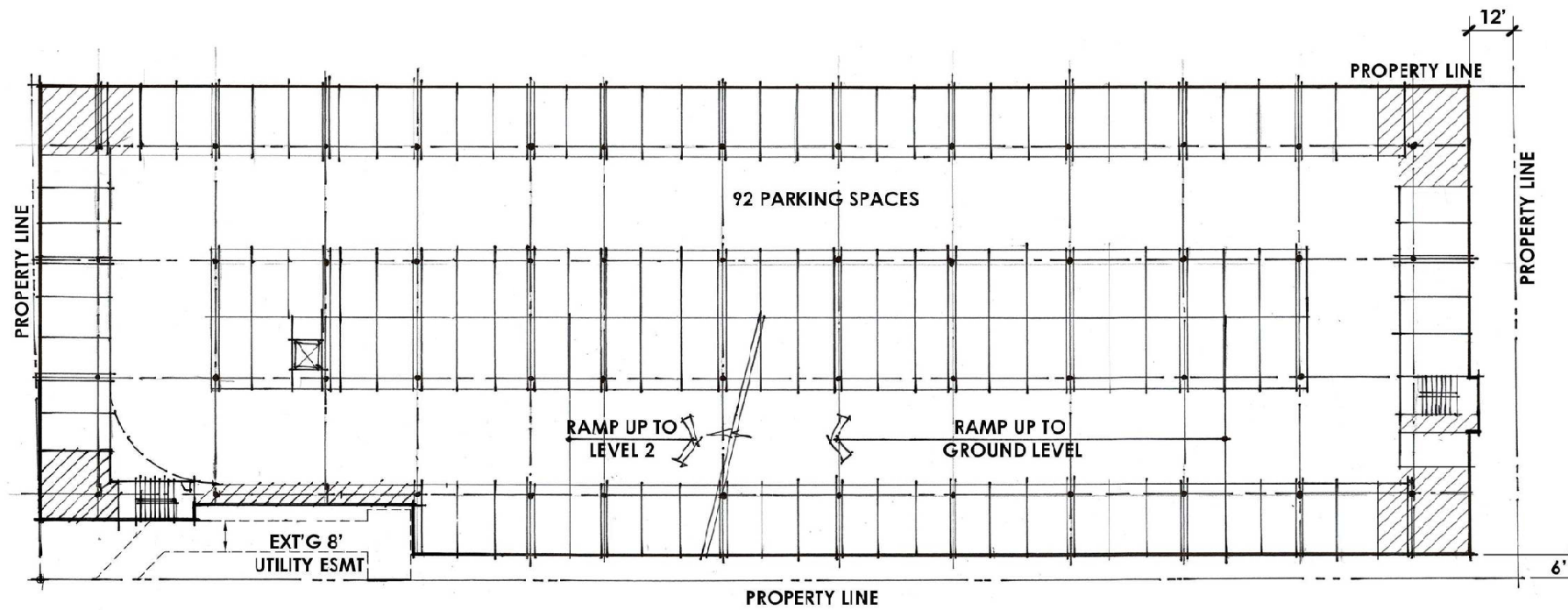
BASEMENT LEVEL 1 PLAN
