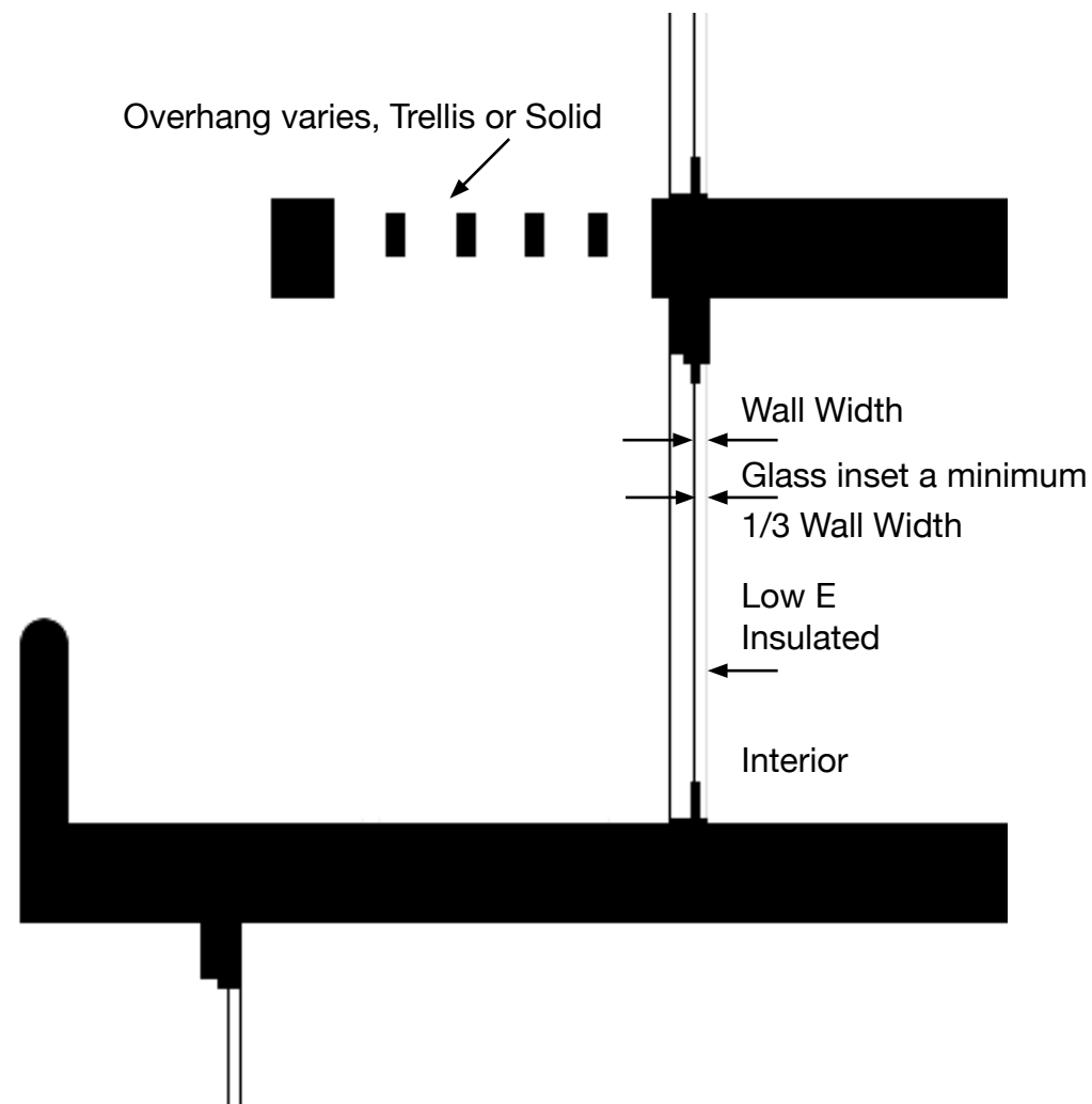
Typical Door or Window at Stepbacks
