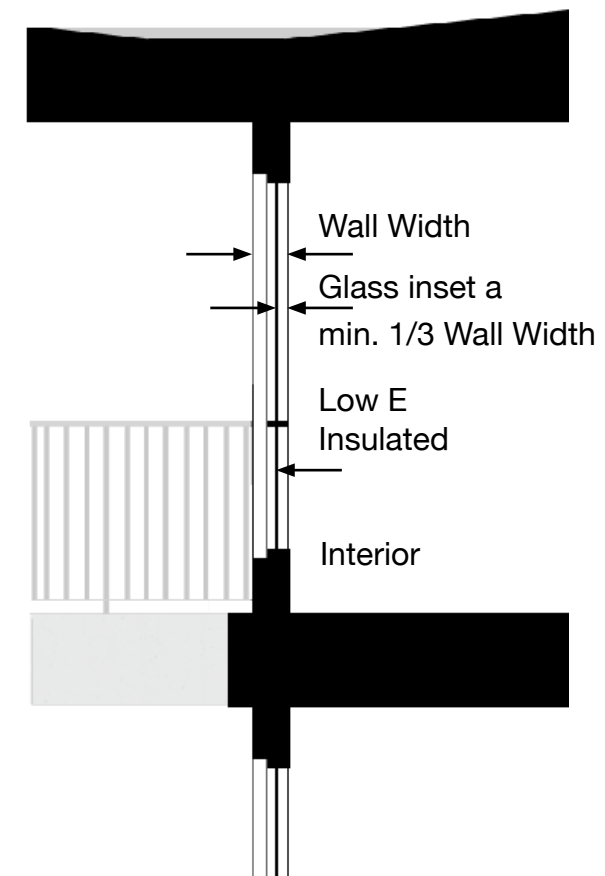
Typical Window at Roof
