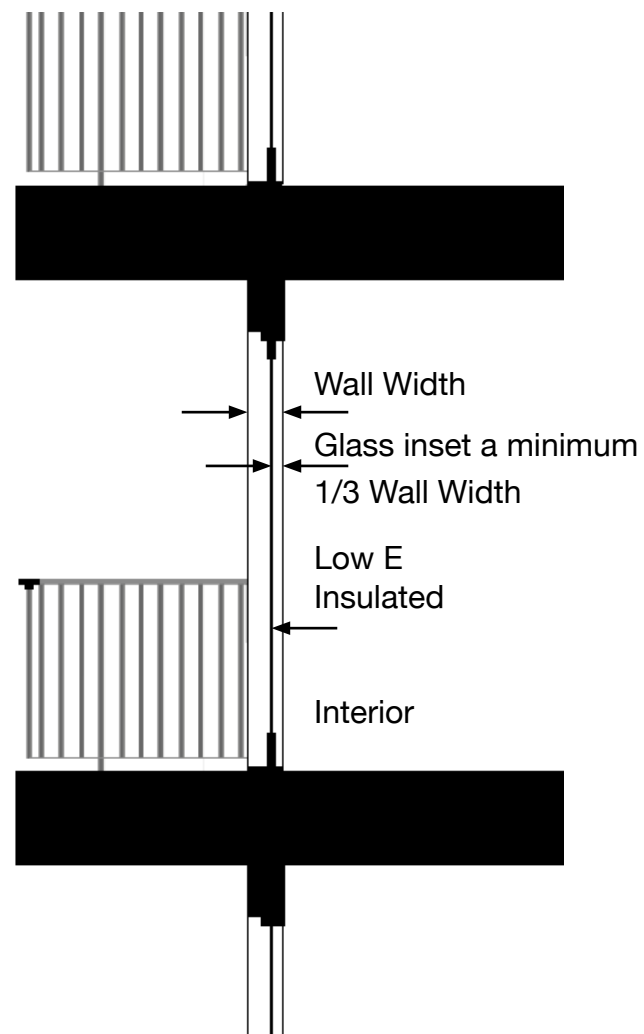
Typical Door at Balcony
