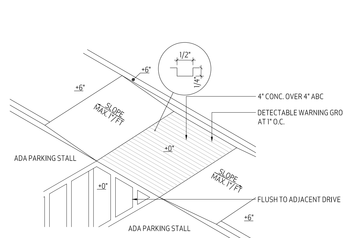
2 ACCESSIBLE PATH SCALE: 1/4"=1'-0"
