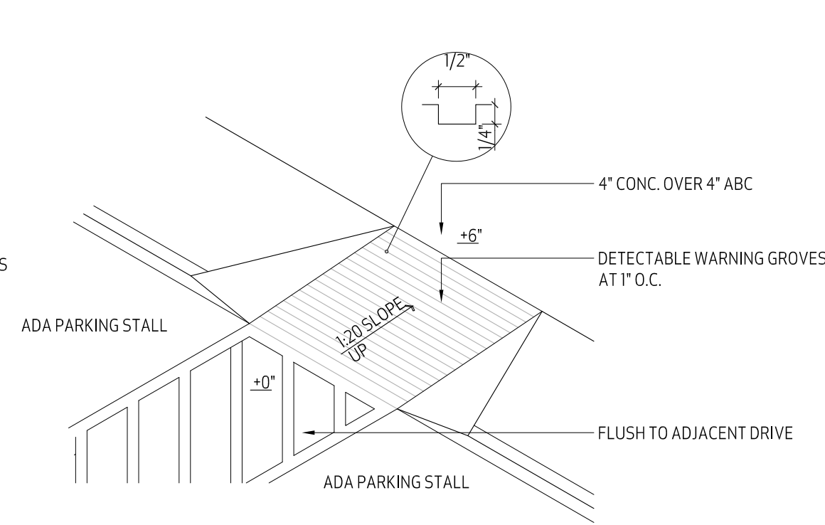
1 ACCESSIBLE PATH SCALE: 1/4"=1'-0"
