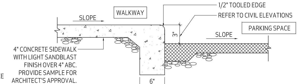
6B WALKWAY AT PARKING SCALE: 1/2"=1'-0"
