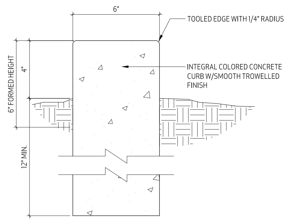
5 LANDSCAPING CURB SCALE: 3/4"=1'-0"
