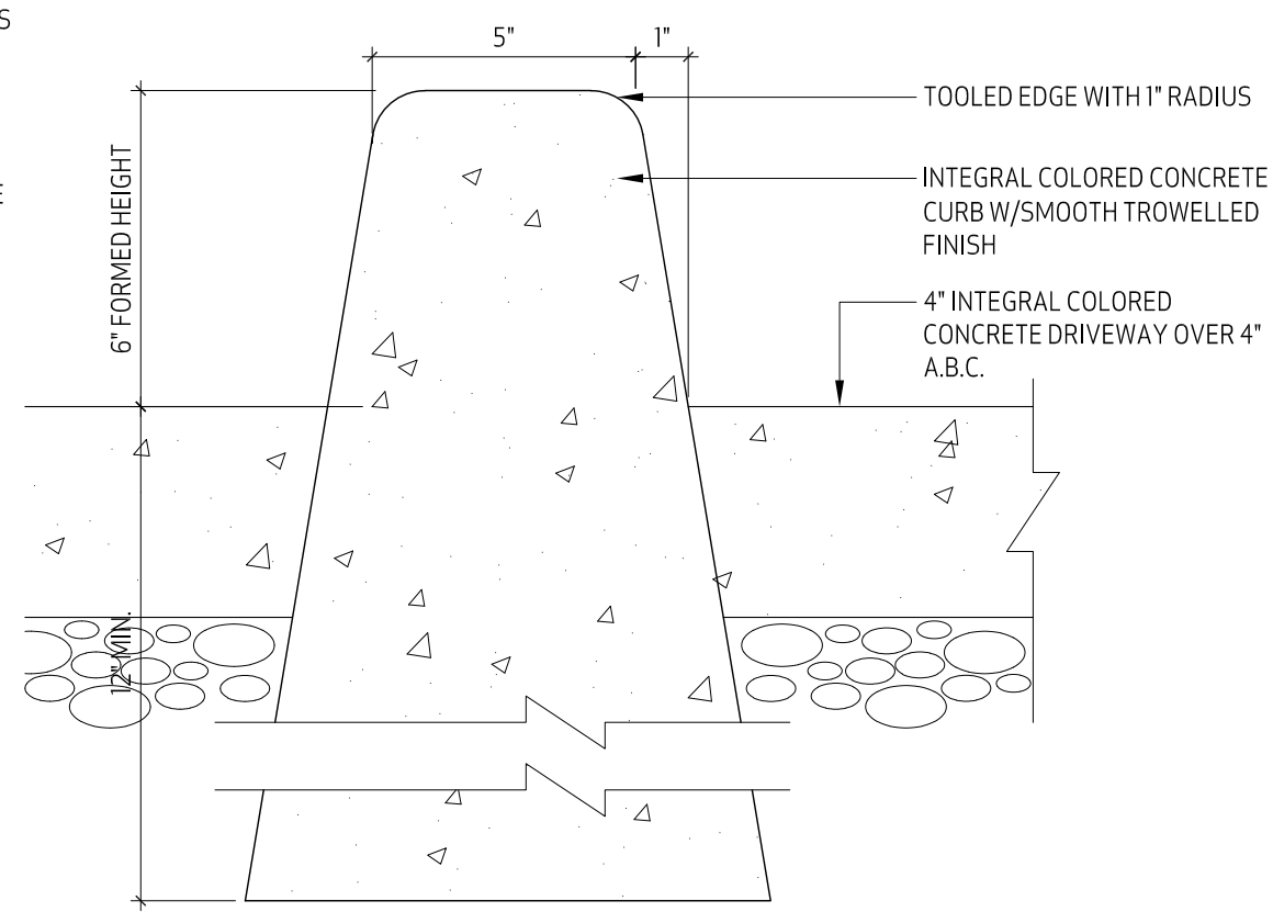
4 PARKING CURB SCALE: 3/4"=1'-0"
