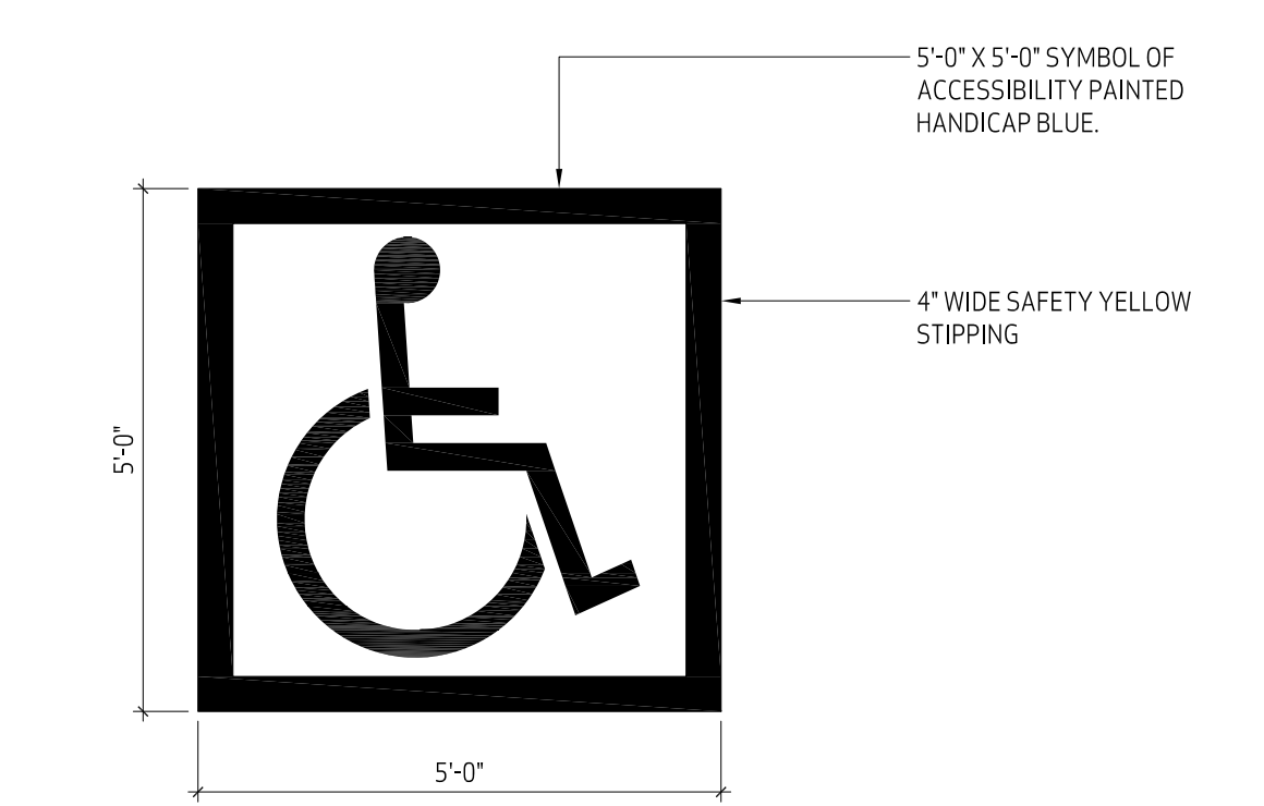
13 ACCESSIBLE PARKING SIGN SCALE: 1/2"=1'-0"
