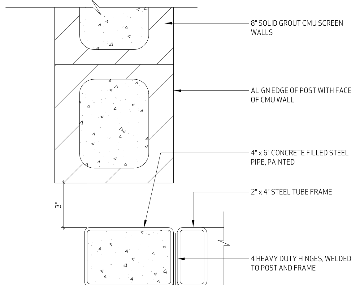
7 GATE POST SCALE: 3/4"=1'-0"
