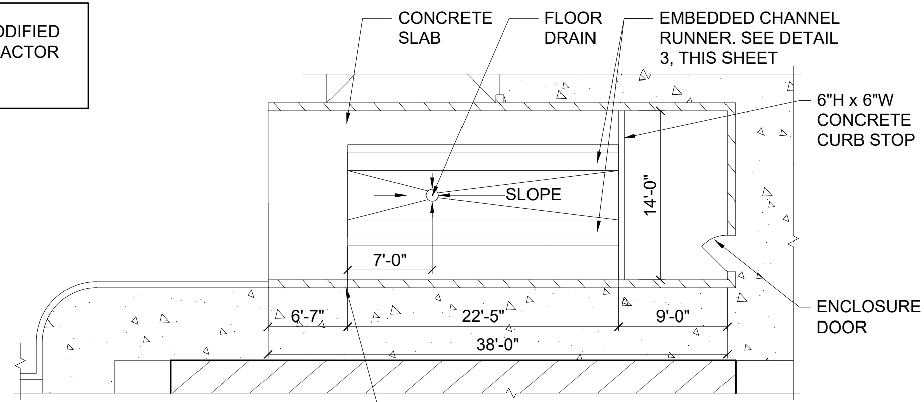
2 TRASH COMPACTOR PLAN scale: 1"= 40'
