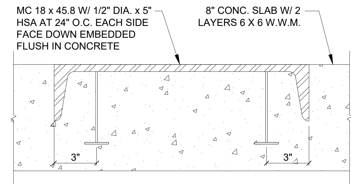
3 CHANNEL RUNNER INSERT scale: 3"= 1'-0"
