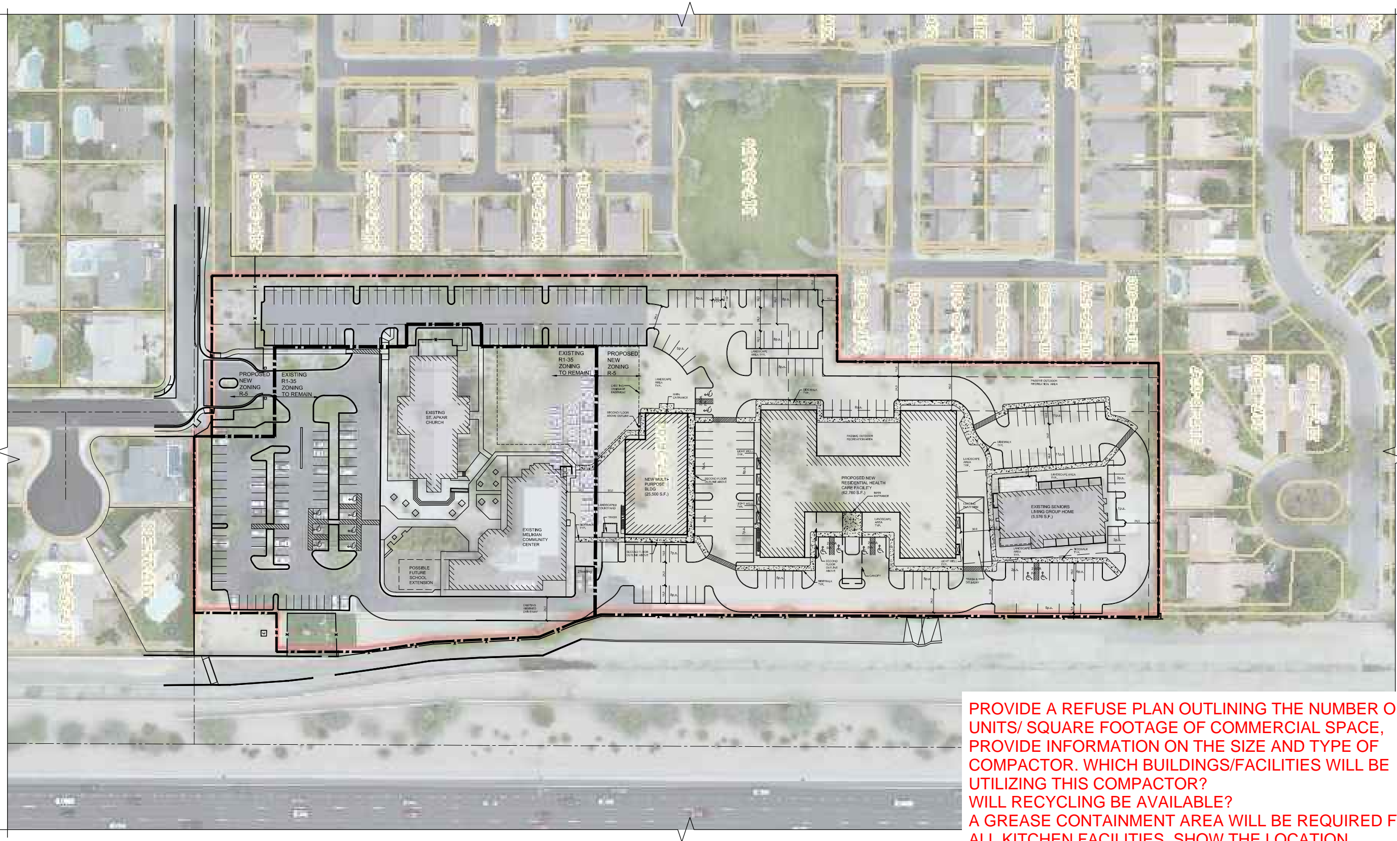
PROPOSED REZONING SITE PLAN SCALE: 1"=100'
