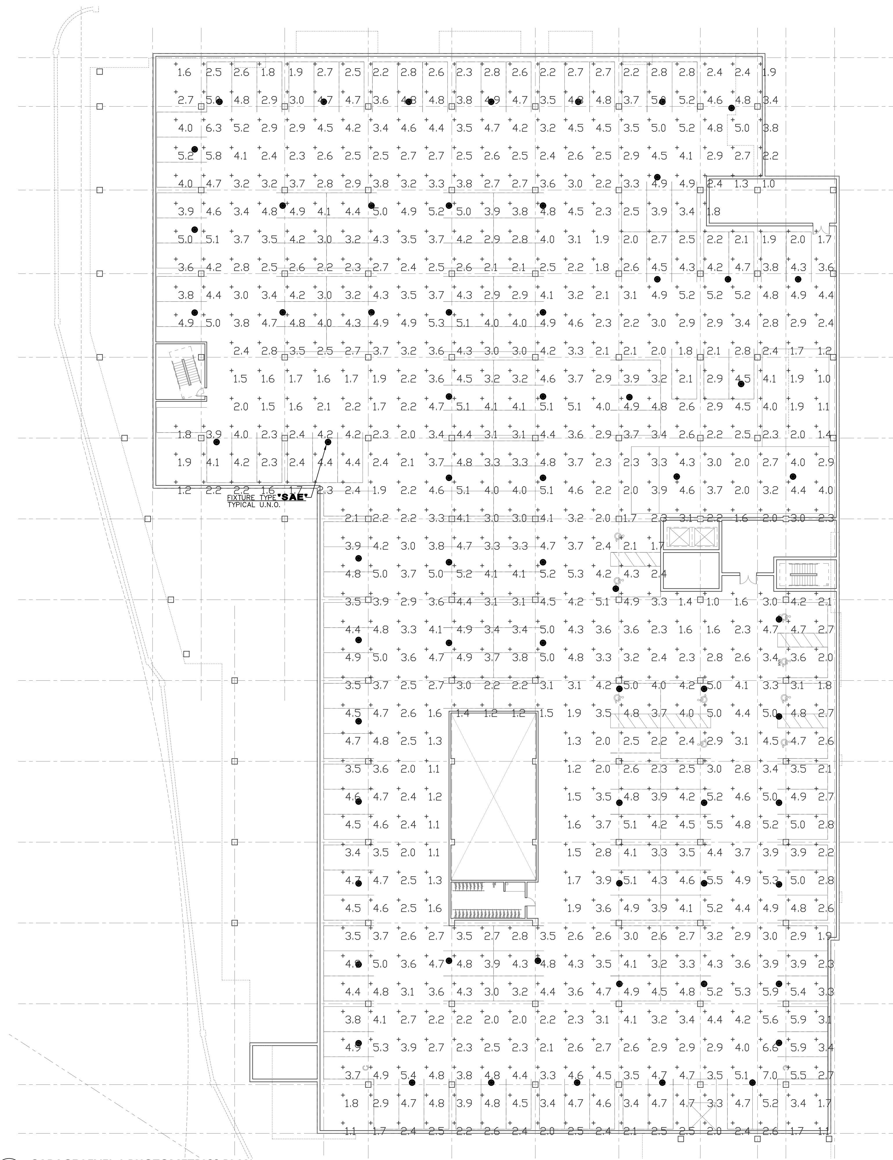
1 GARAGE LEVEL 1 PHOTOMETRICS PLAN 1" = 20' - 0"
