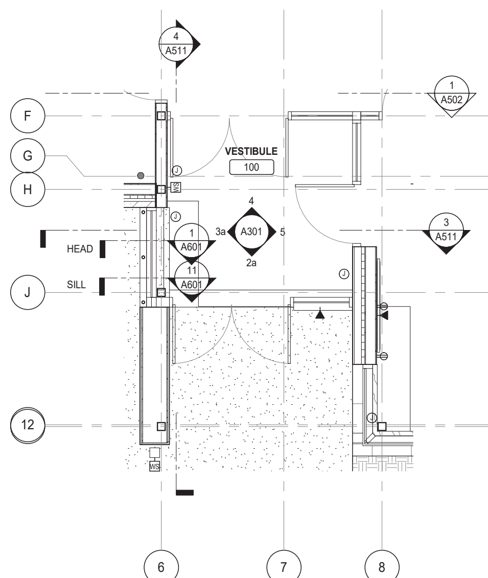
6 PARTIAL PLAN AT VESTIBULE 1/4" = 1'-0"
