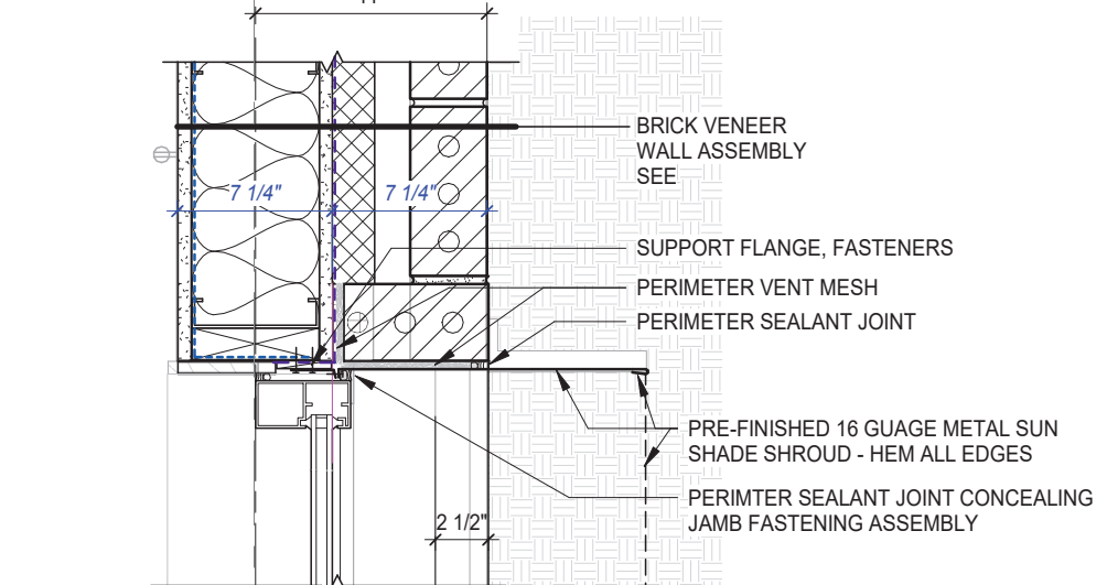
3B WINDOW JAMB AT BRICK CLADDING 1 1/2" = 1'-0"
