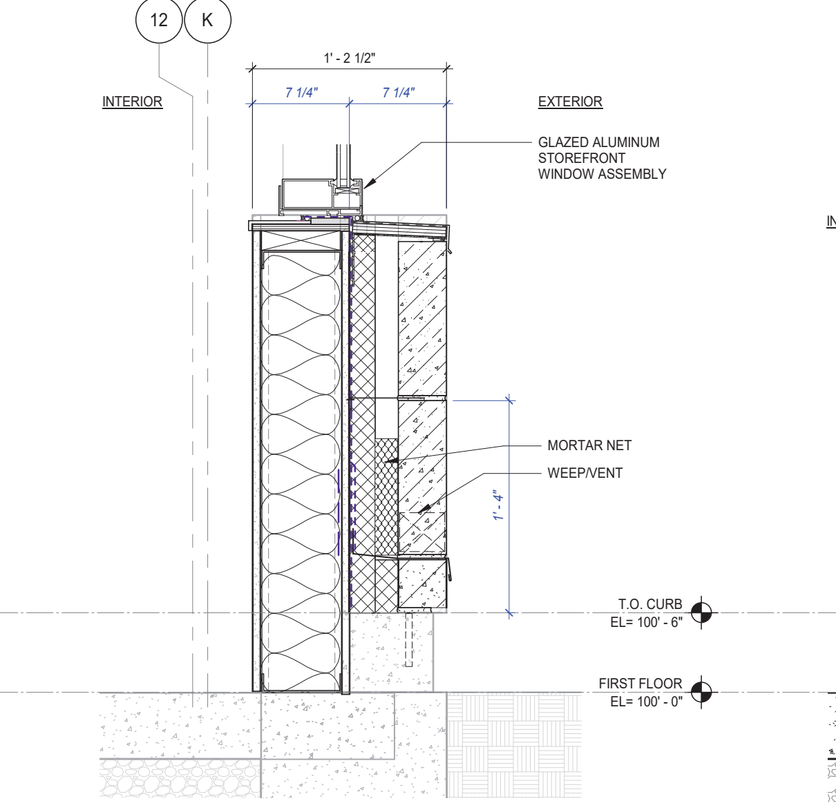
14 WINDOW SILL AT COMMUNITY ROOM 1 1/2" = 1'-0"
