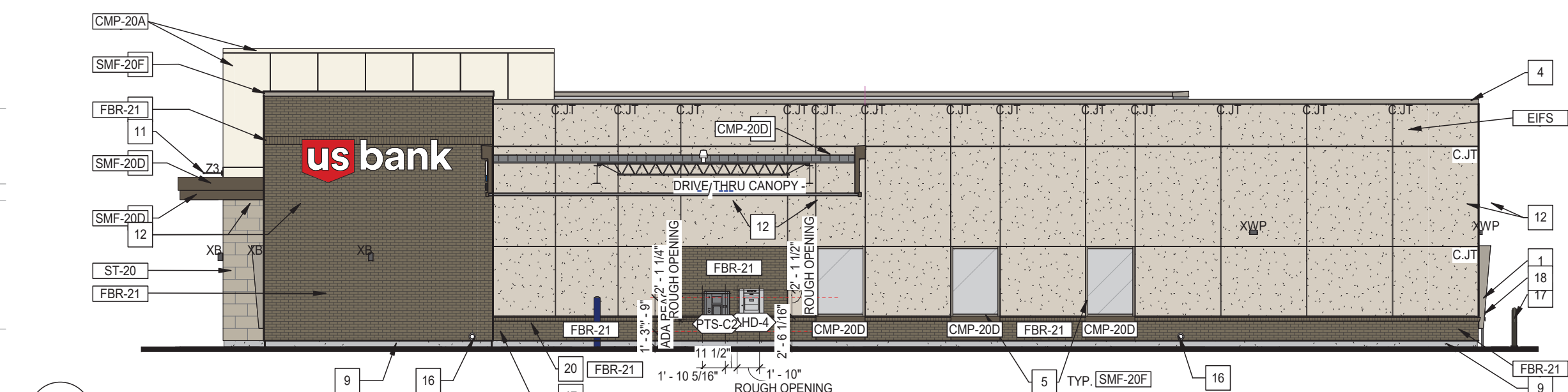
7 ELEVATION - NORTH Color 1/8" = 1'-0"
