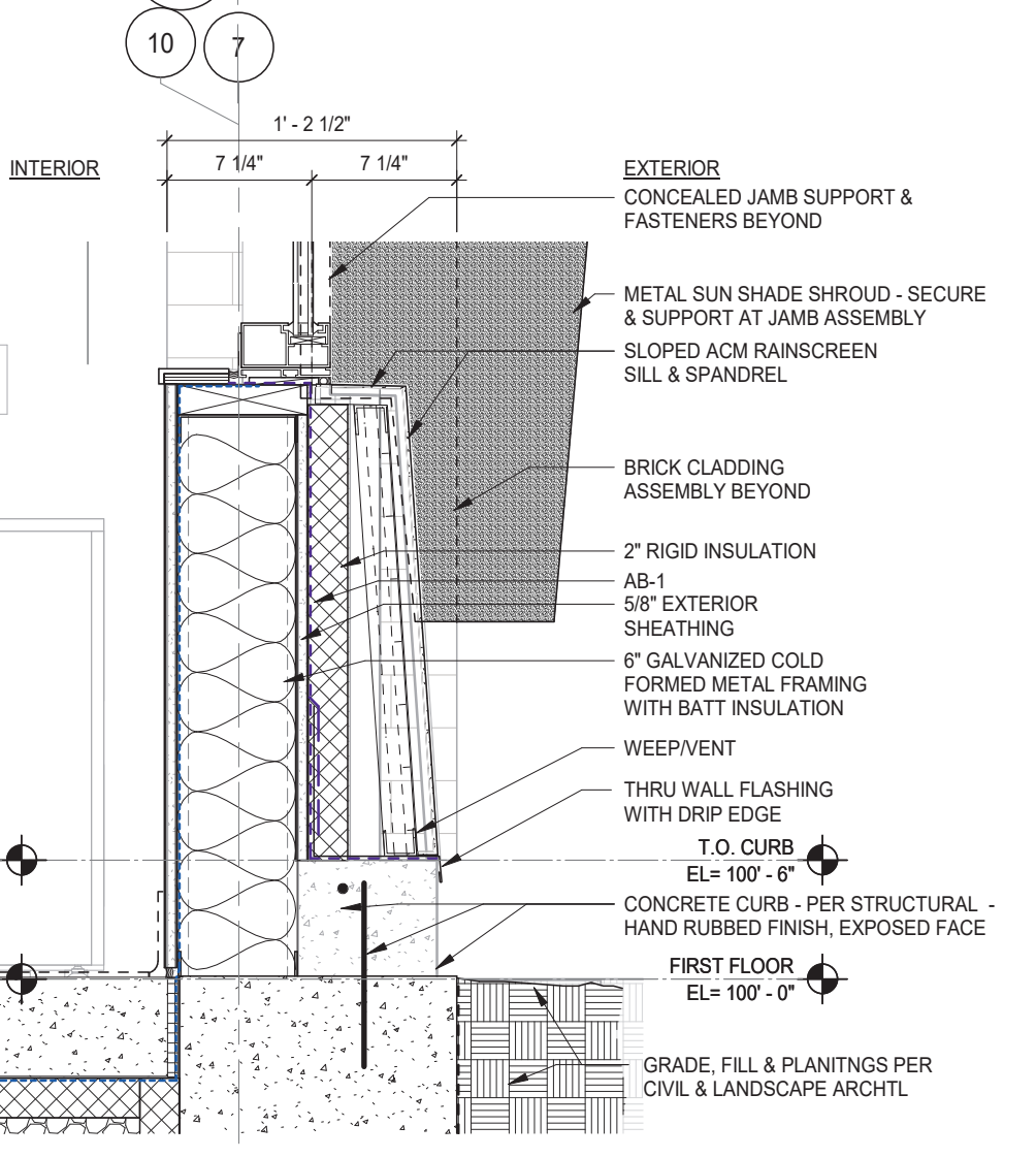
13 WINDOW SILL AT BRICK CLADDING & METAL SPANDREL 1 1/2" = 1'-0"
