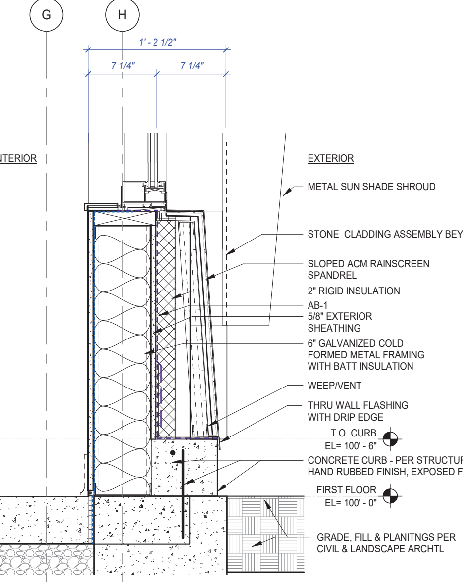
15 WINDOW SILL AT METAL SPANDREL 1 1/2" = 1'-0"
