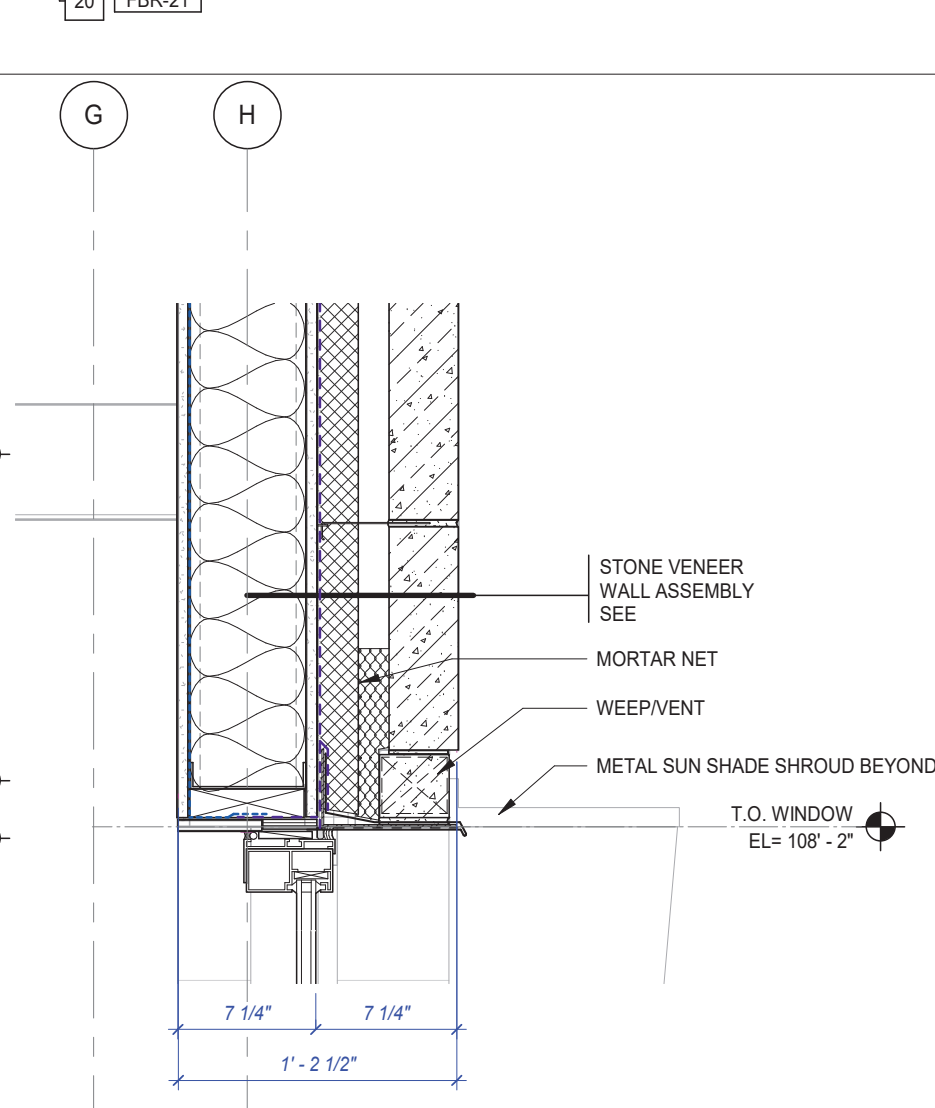
5 WINDOW HEAD AT STONE CLADDING 1 1/2" = 1'-0"
