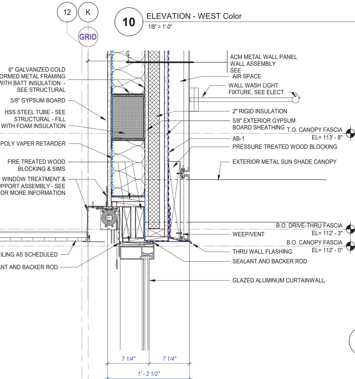
4 WINDOW HEAD AT METAL PANEL CLADDING 1 1/2" = 1'-0"
