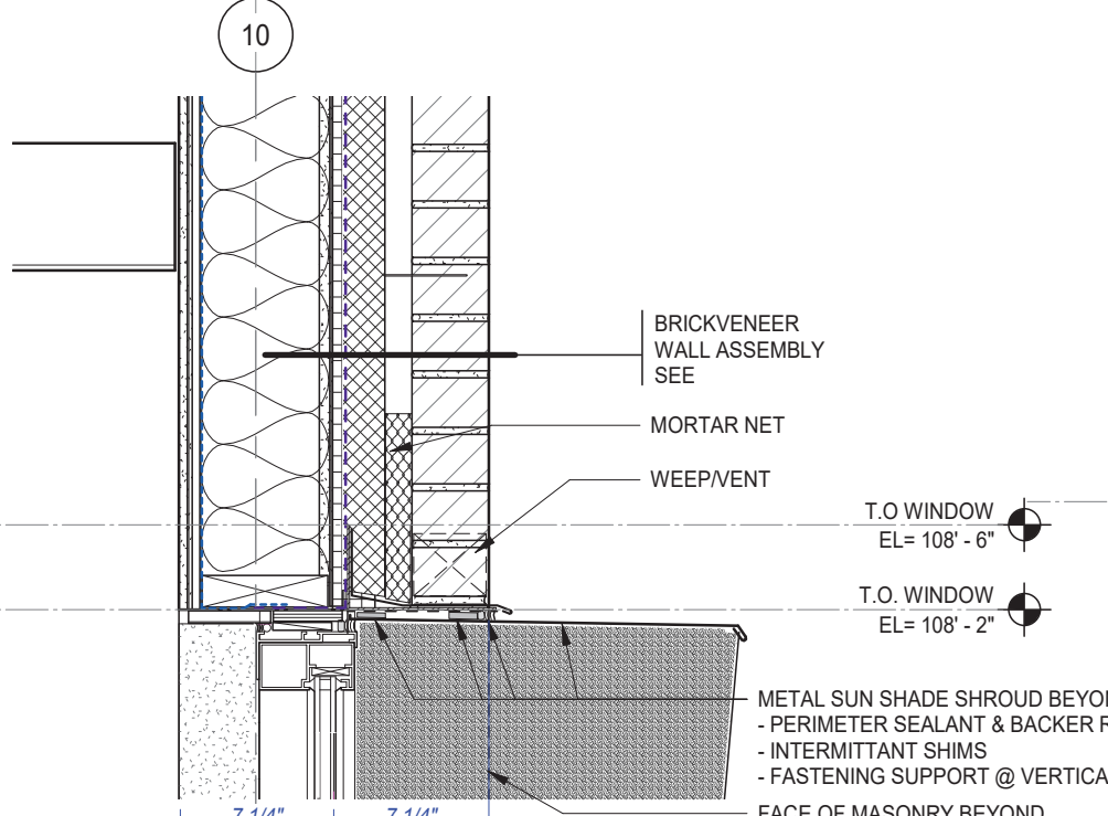
3A WINDOW HEAD AT BRICK CLADDING Rev 1 1 1/2" = 1'-0"
