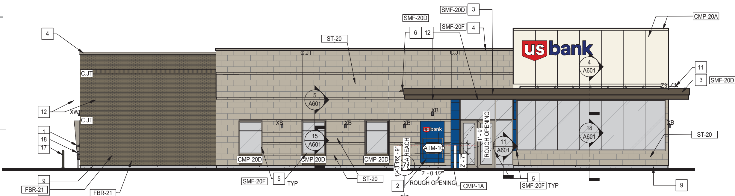
9 ELEVATION - SOUTH Color 1/8" = 1'-0"
