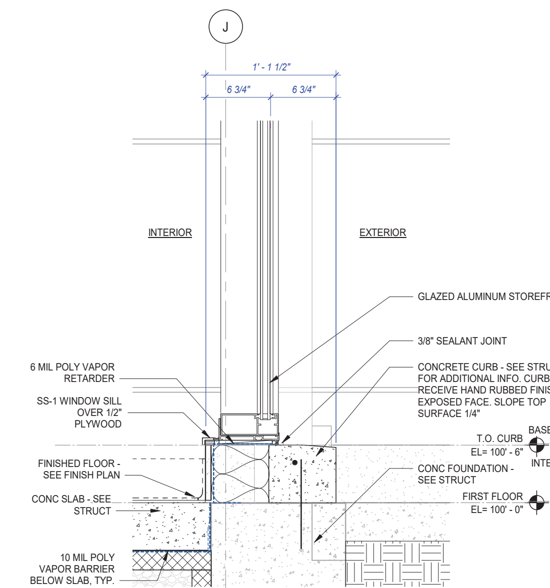
11 WINDOW SILL AT VESTIBULE 1 1/2" = 1'-0"
