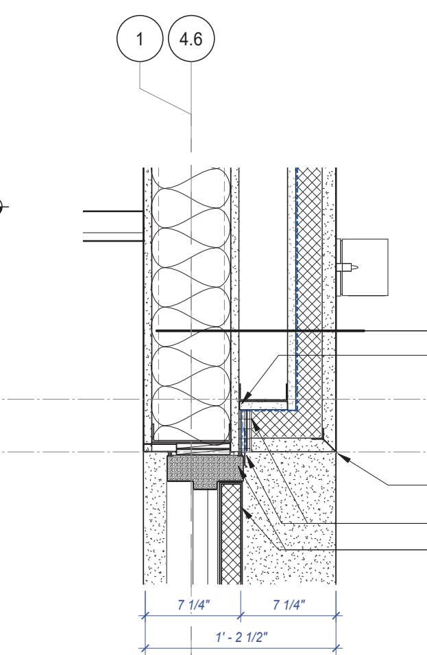
2 HOLLOW METAL DOOR HEAD AT BRICK 1 1/2" = 1'-0"
