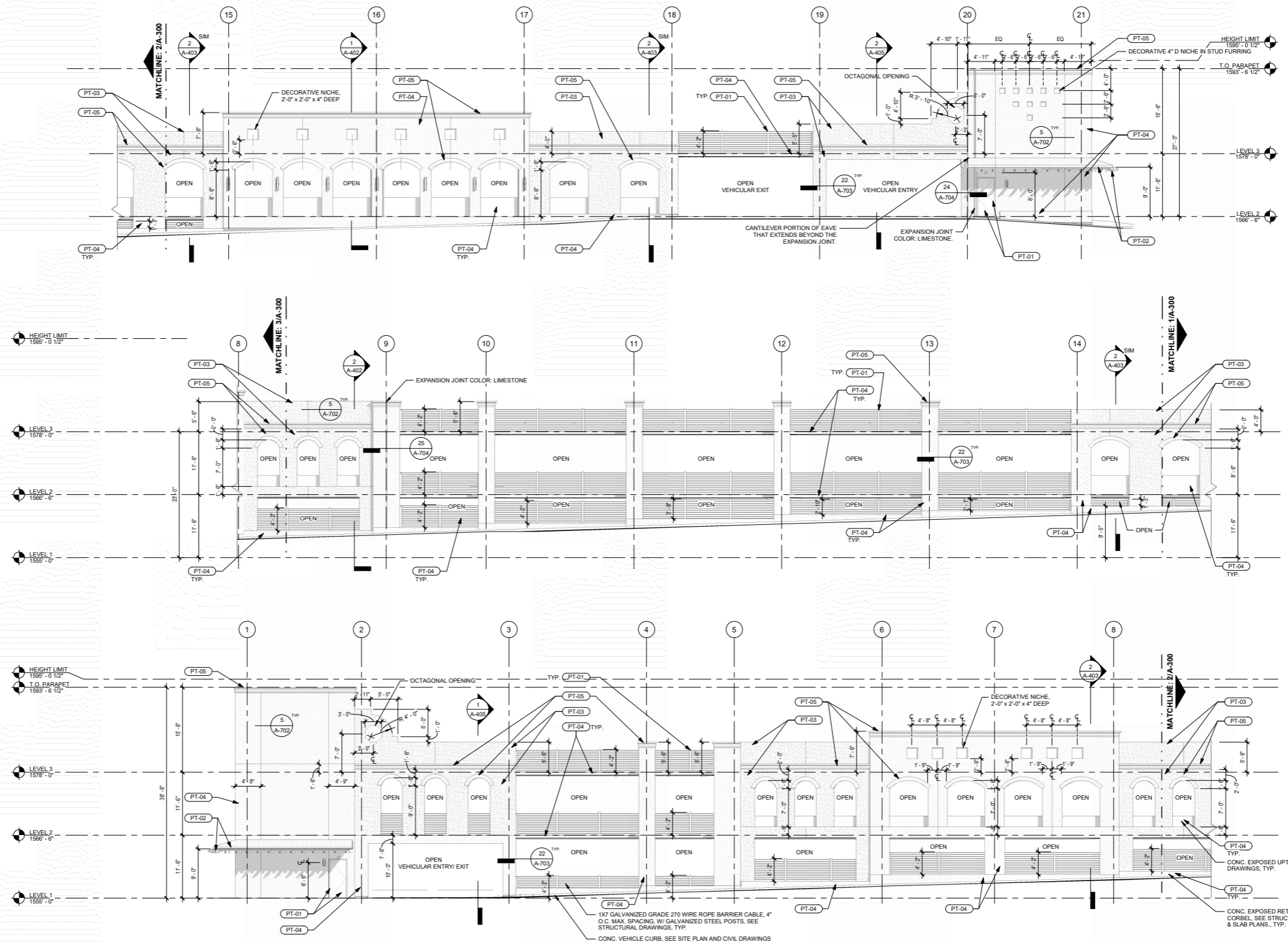
ELEVATION - EAST 1/8" = 1'-0" 1
