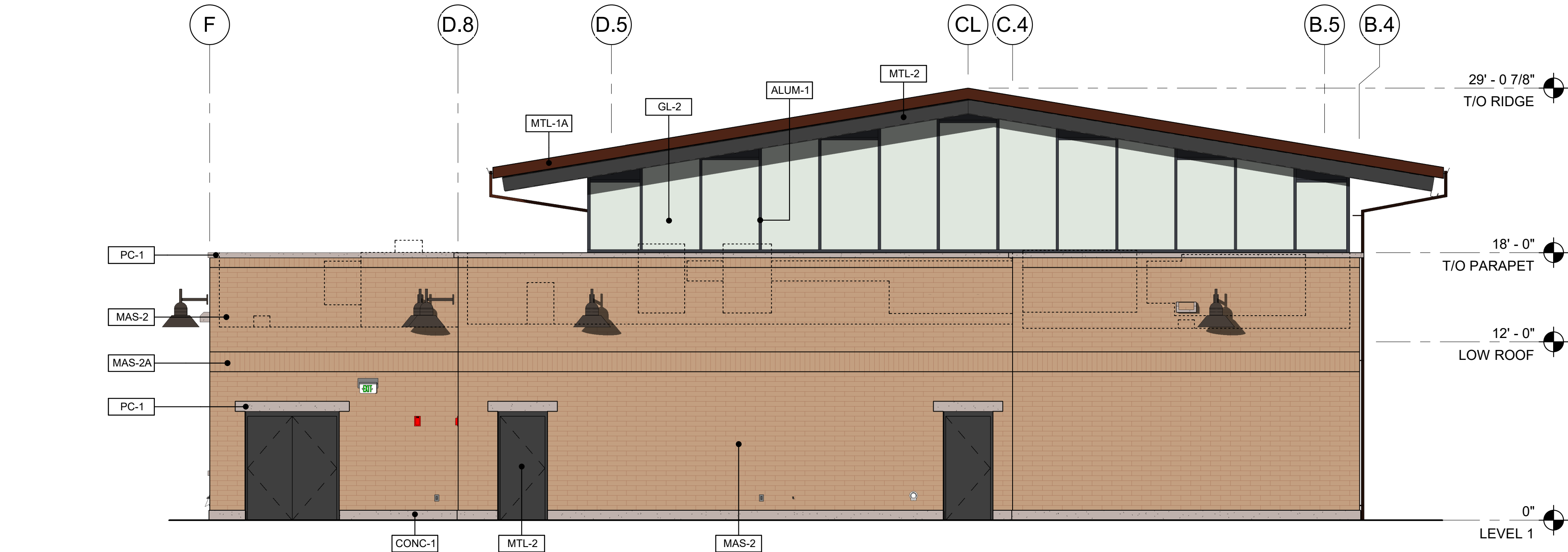
3 NORTH BUILDING COLOR ELEVATION 3/16" = 1'-0"
