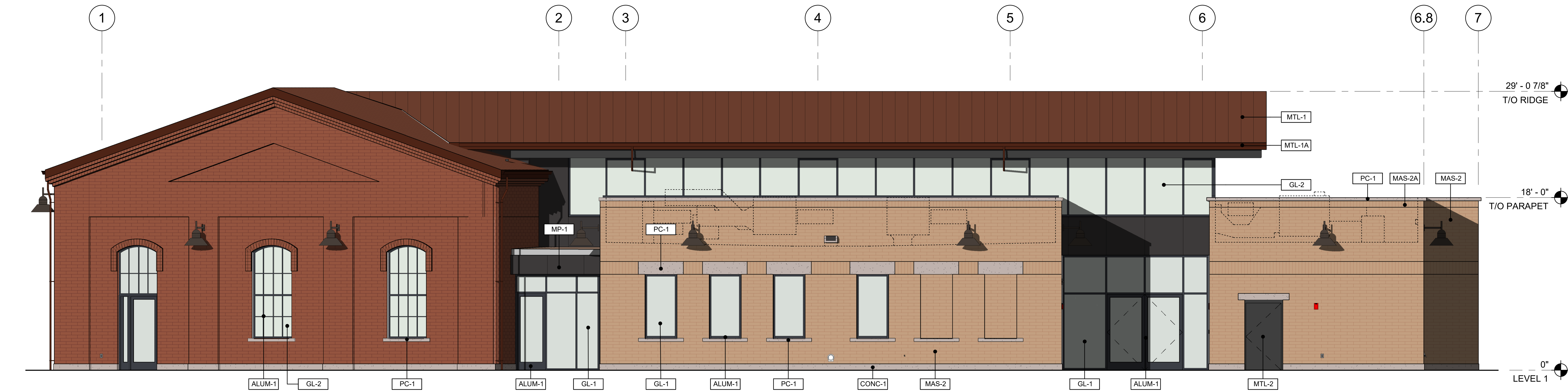
2 EAST BUILDING COLOR ELEVATION 3/16" = 1'-0"
