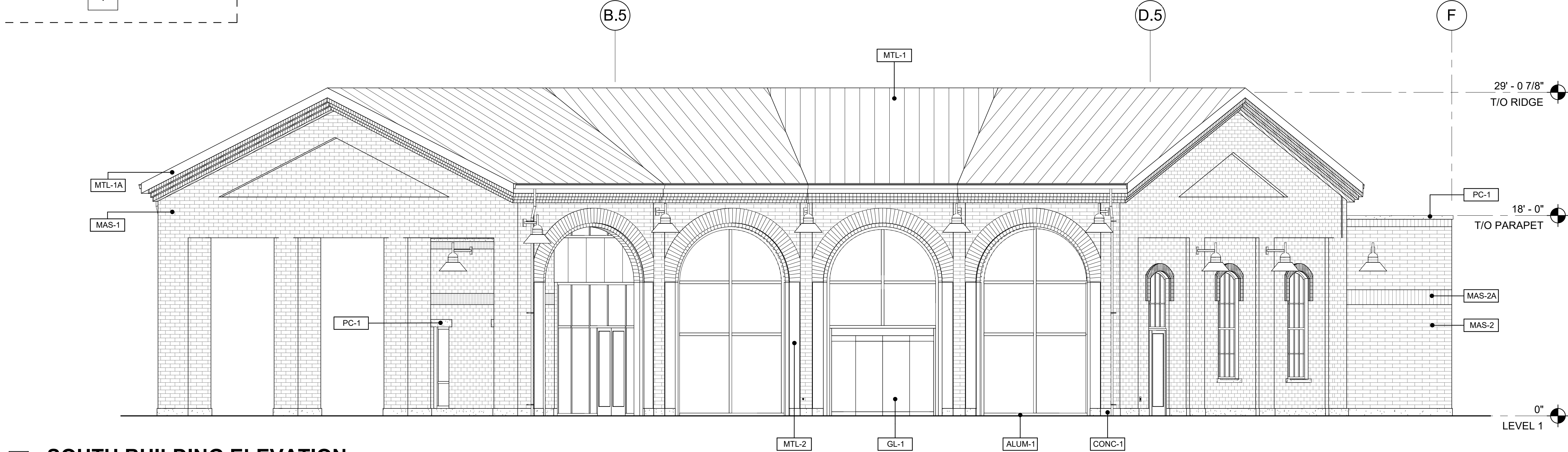
1 SOUTH BUILDING ELEVATION 3/16" = 1'-0"
