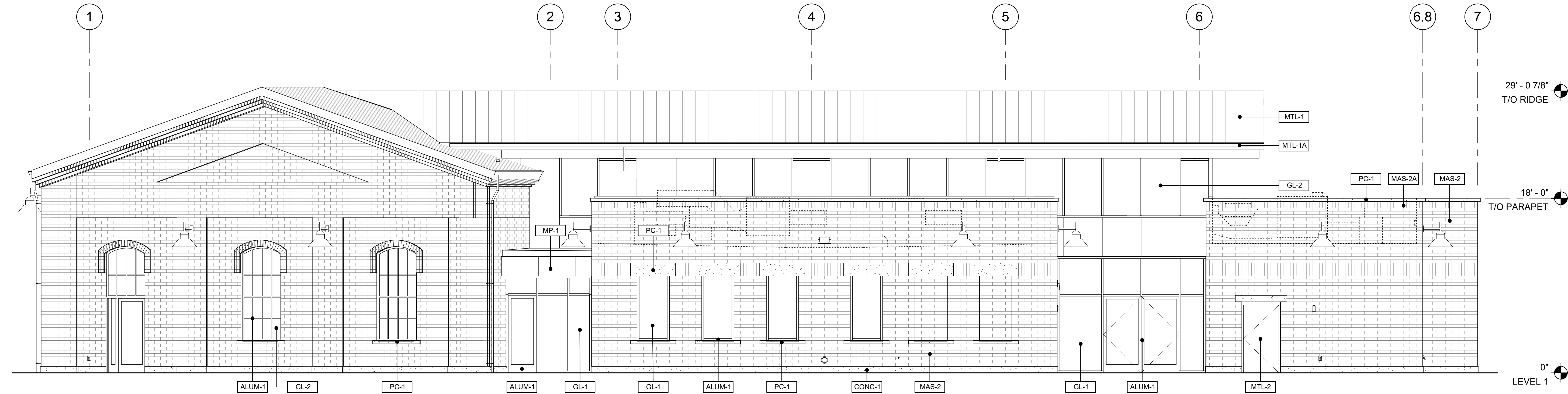
2 EAST BUILDING ELEVATION 3/16" = 1'-0"
