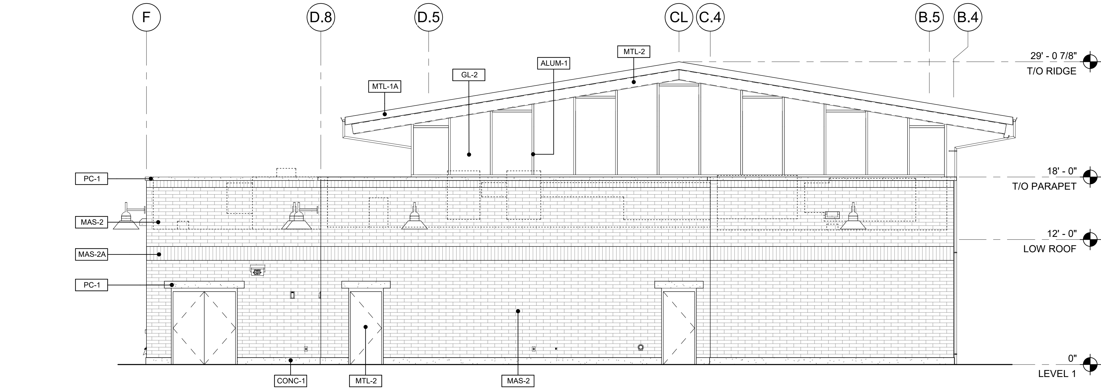
1 NORTH BUILDING ELEVATION 3/16" = 1'-0"
