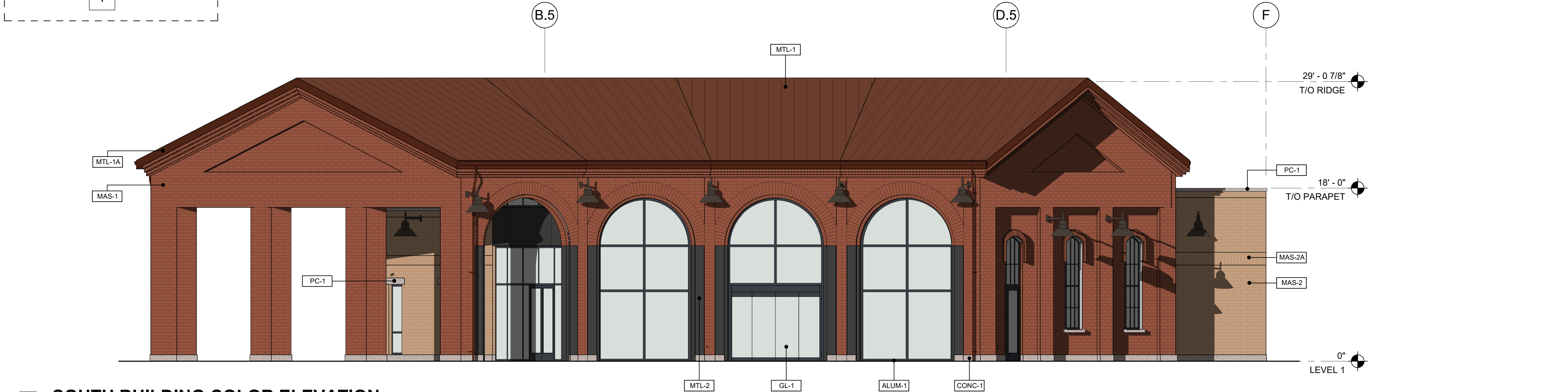
1 SOUTH BUILDING COLOR ELEVATION 3/16" = 1'-0"
