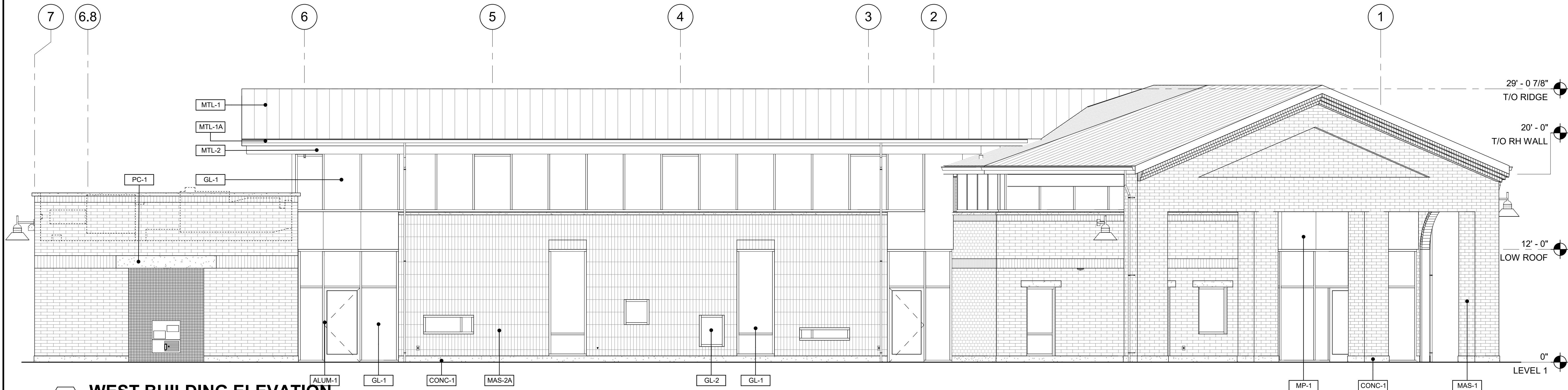
2 WEST BUILDING ELEVATION 3/16" = 1'-0"
