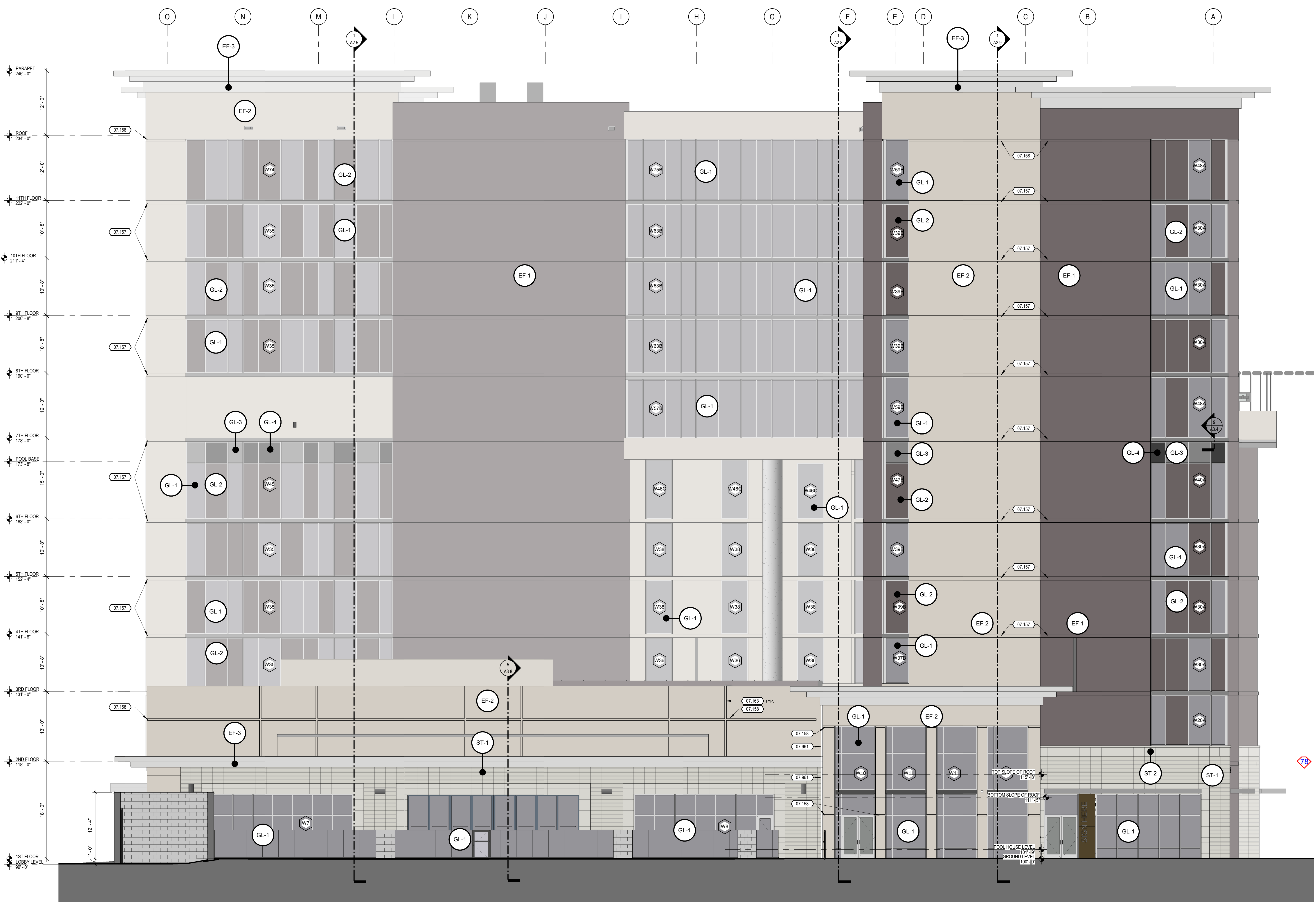
1 EAST ELEVATION 3/8" = 1'-0"
