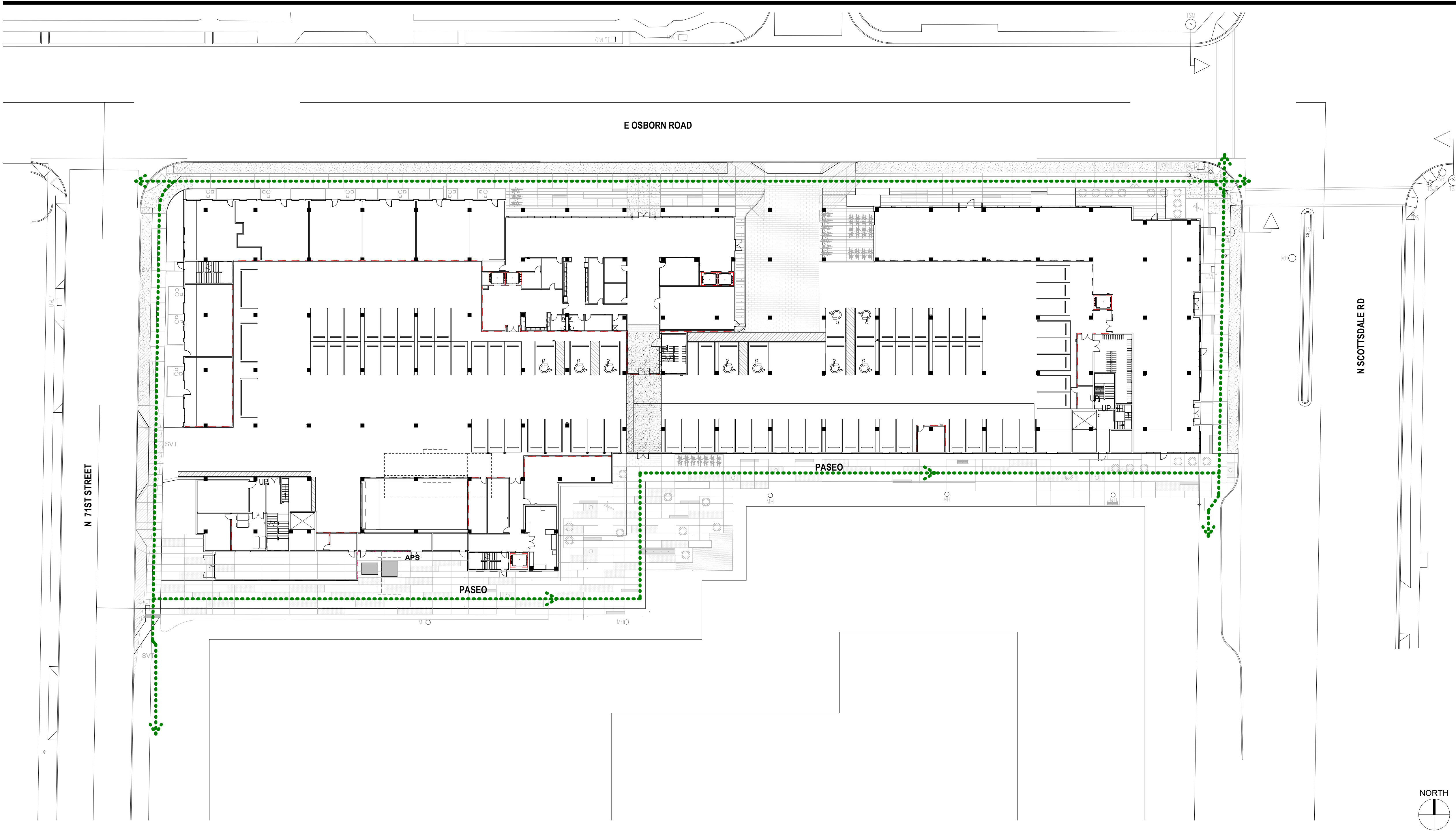
01 BIKEWAYS & TRAILS PLAN SCALE: 1" = 30'-0"
