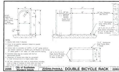
2285 City of Scottsdale Standard Details Double Bicycle Rack 2285
