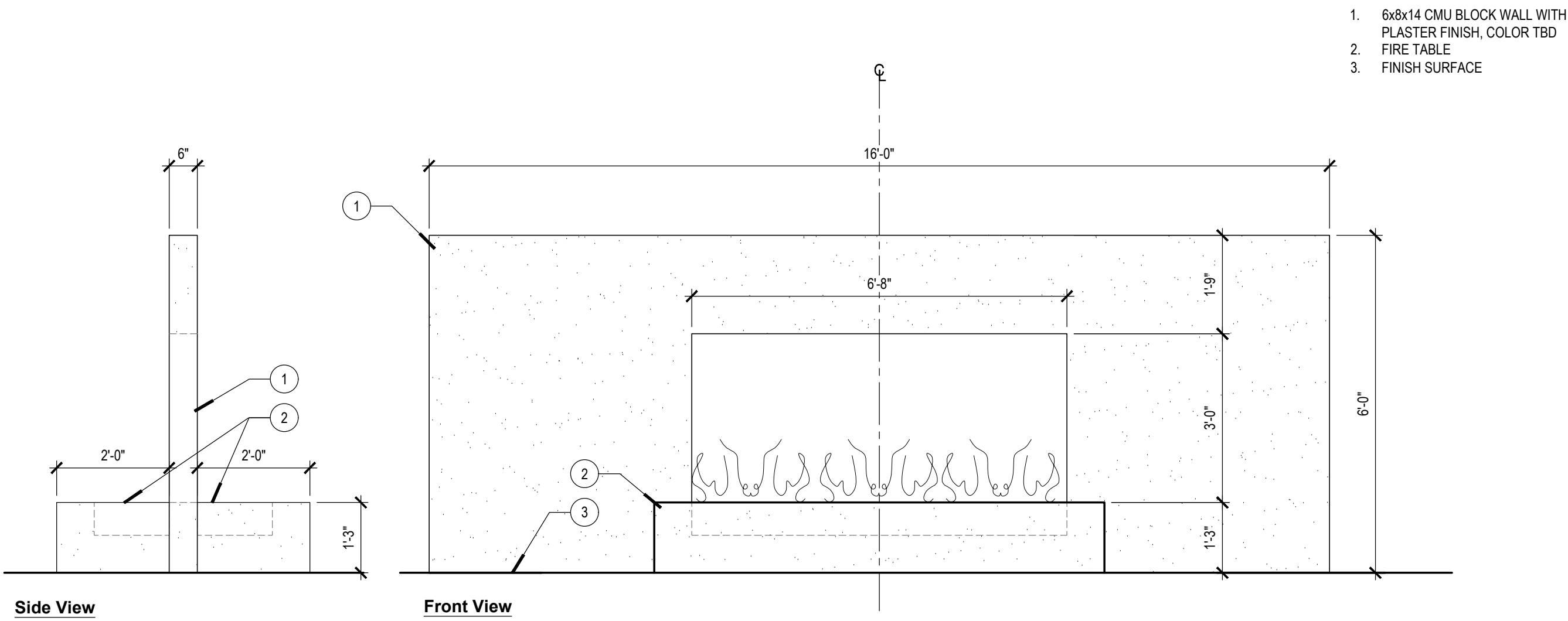
K Sunset Garden Wall - Elevation Scale: 1/2" = 1'-0"
