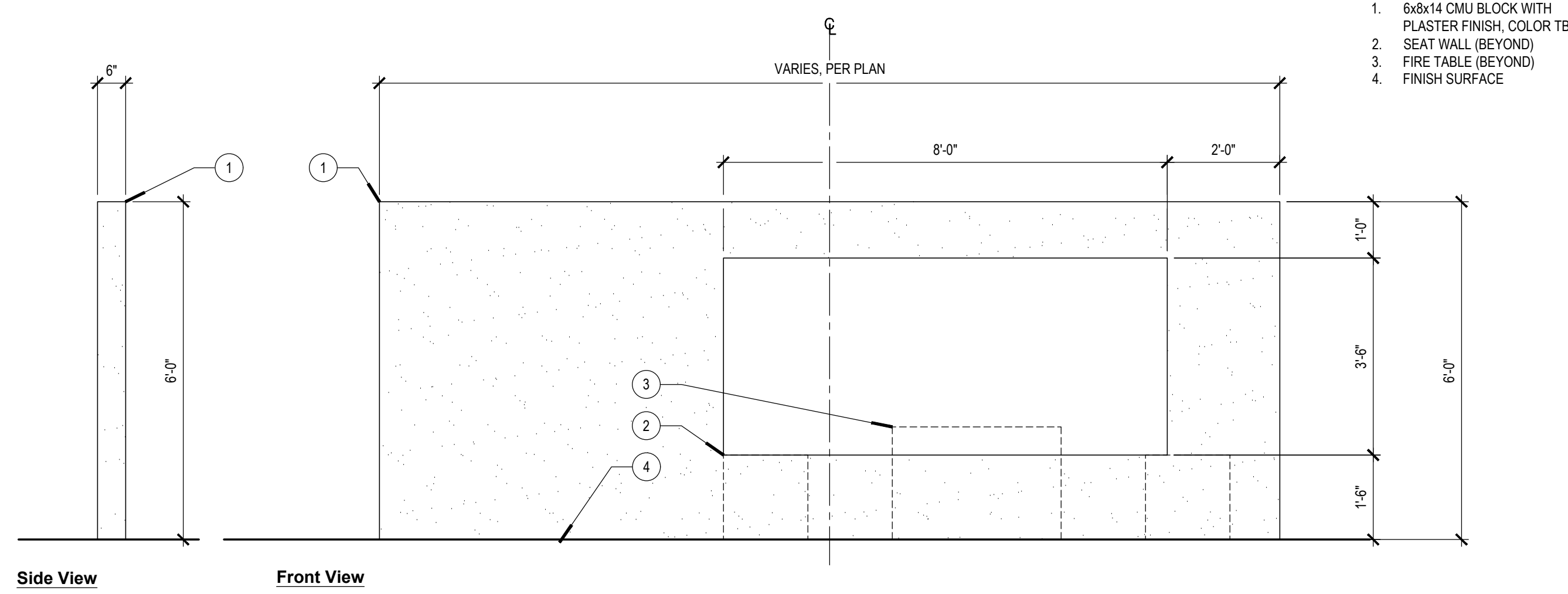
L Garden Room Wall - Elevation (Typical) Scale: 1/2" = 1'-0"
