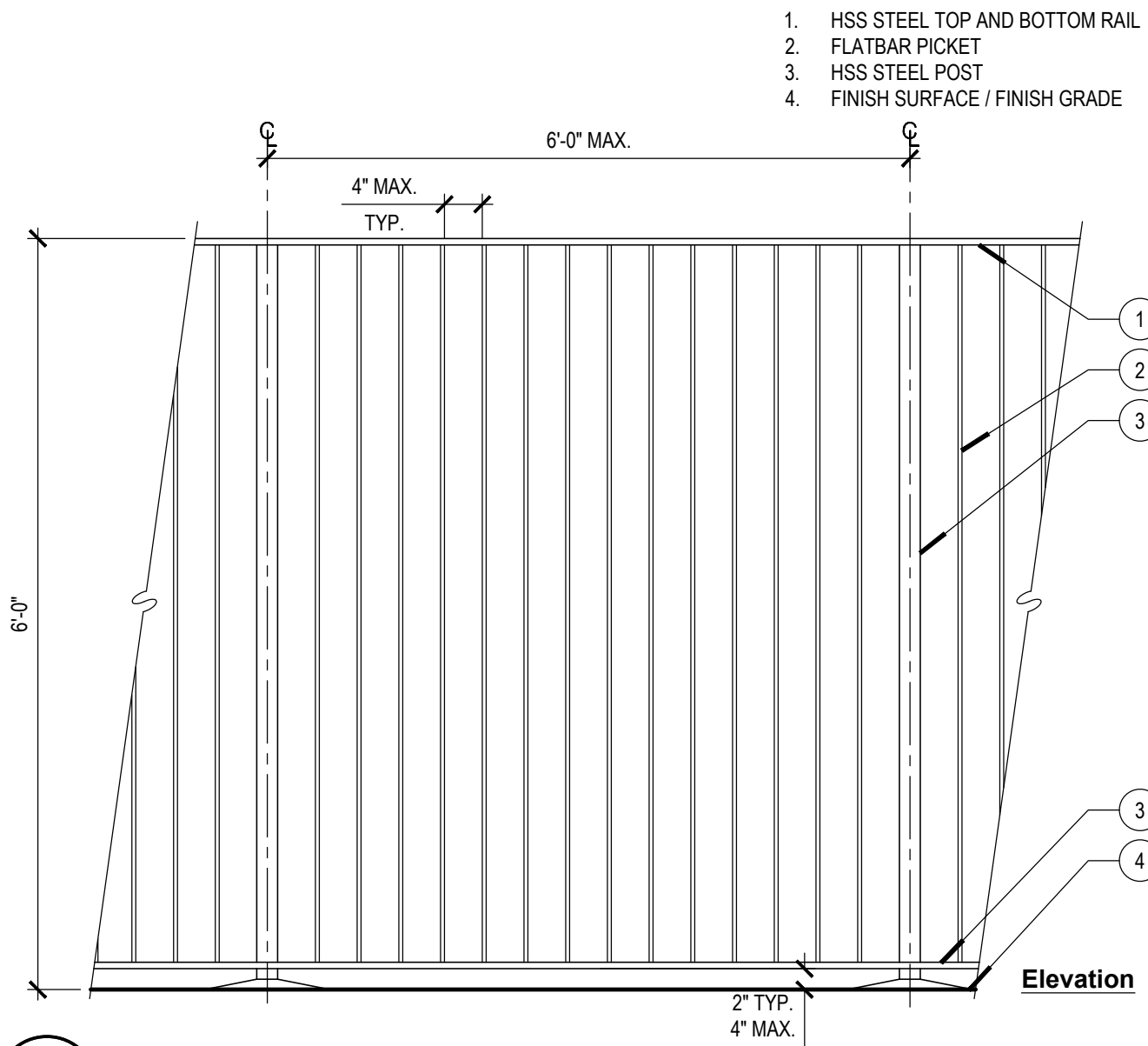
E Perimeter Fence - Tube Steel Scale: 3/4" = 1'-0"
