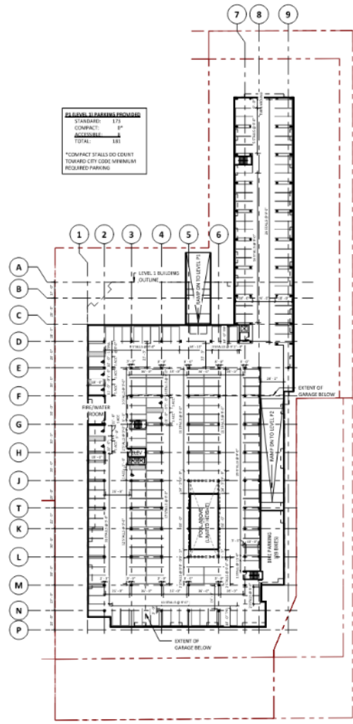
1 ZONING - LEVEL P1 PARKING PLAN 8.21.09 1" = 40' 0"
