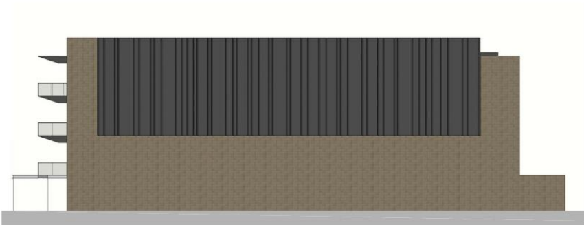
SOUTH ELEVATION SCALE 1/8" = 1'-0"
