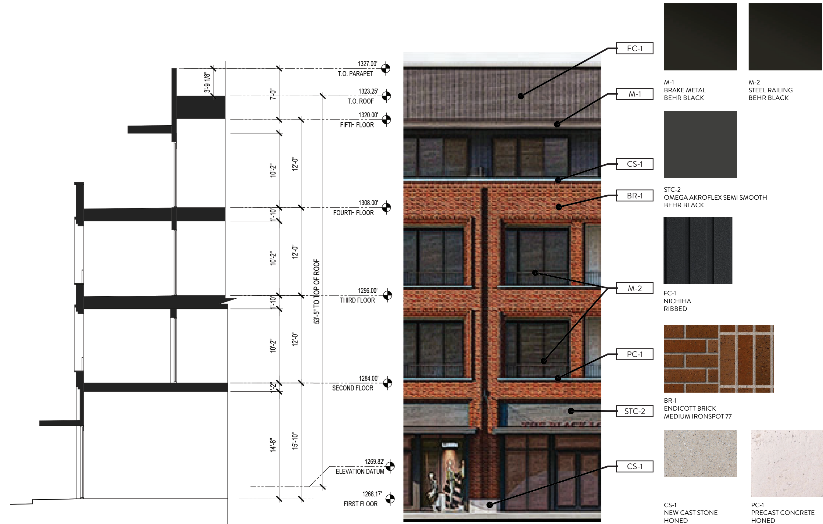
04 ENLARGEMENT D SCALE: 1/8"=1' 0 8' 16'
