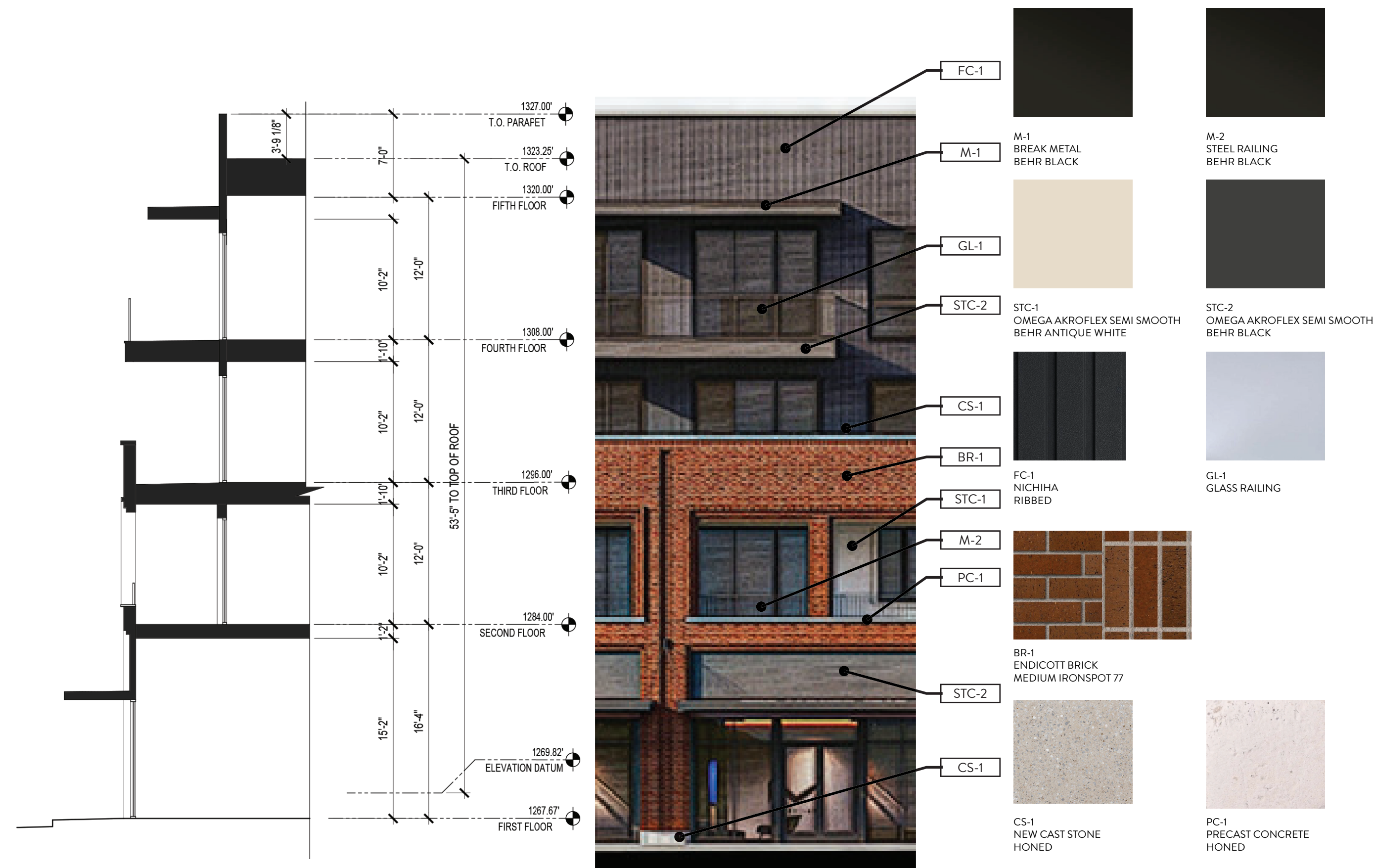
03 ENLARGEMENT C SCALE: 1/8"=1' 0 8' 16'
