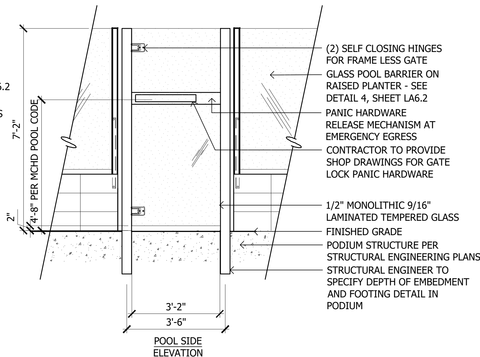
5 Glass Pool Barrier SCALE: 1/2"=1'-0"
