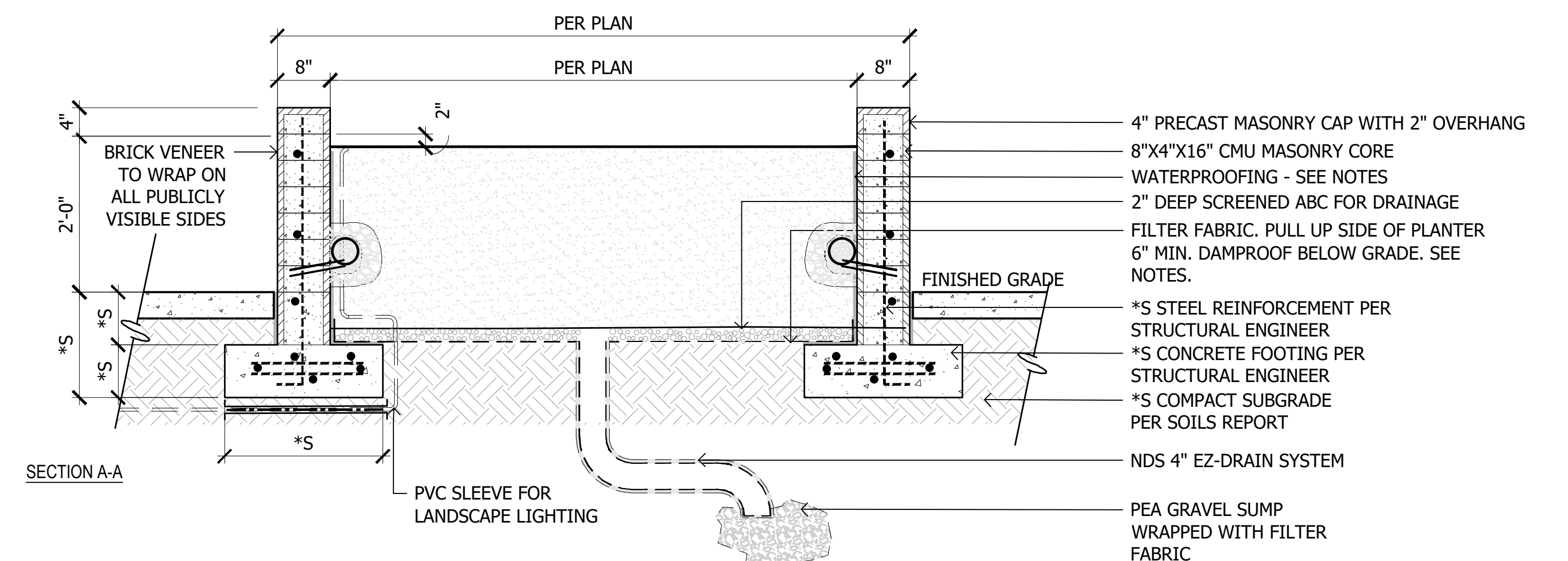
7 Raised Planter at Grade SCALE: 3/4"=1'-0"
