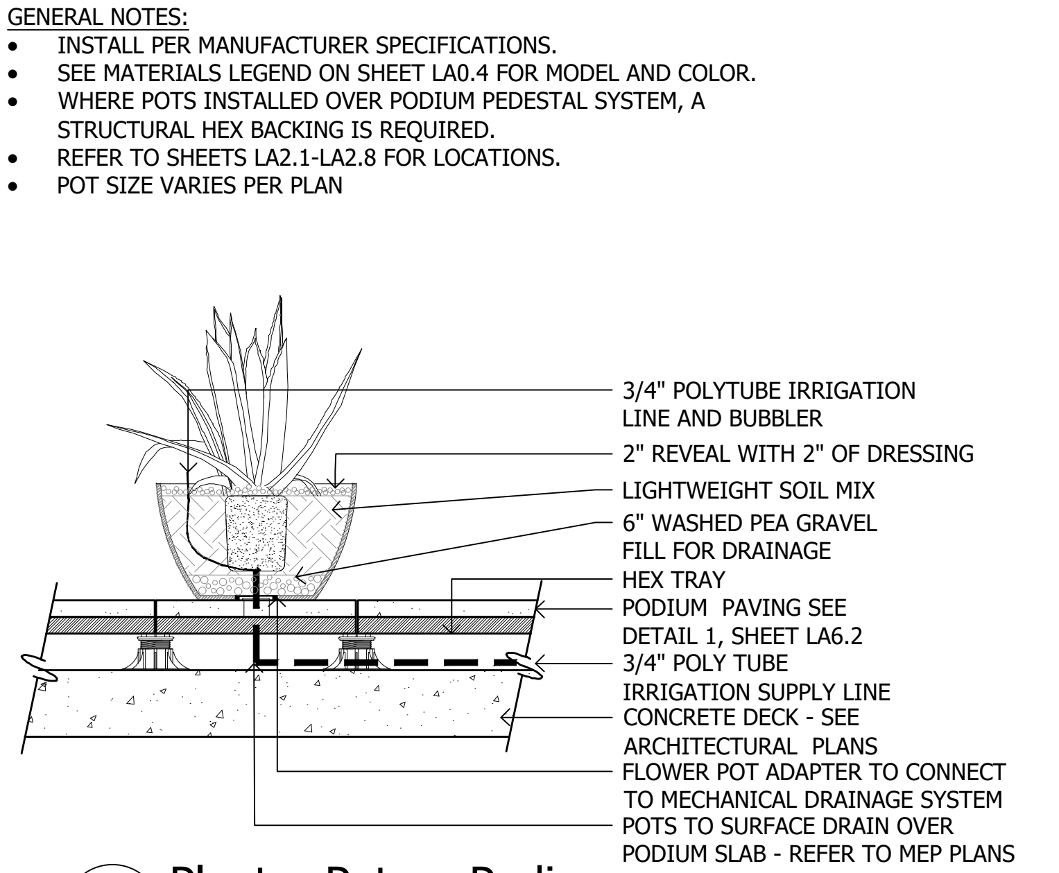
4 Planter Pot on Podium SCALE: 3/4"=1'-0"
