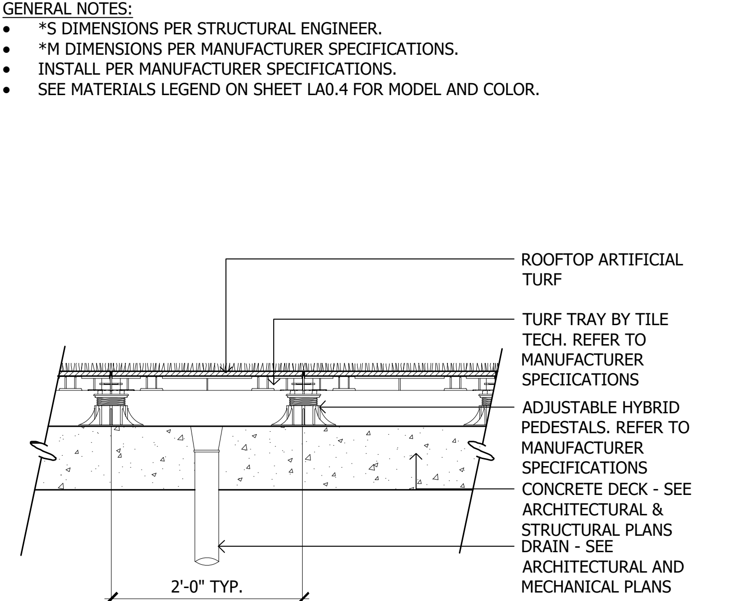
2 Podium Artificial Turf SCALE: 1"=1'-0"
