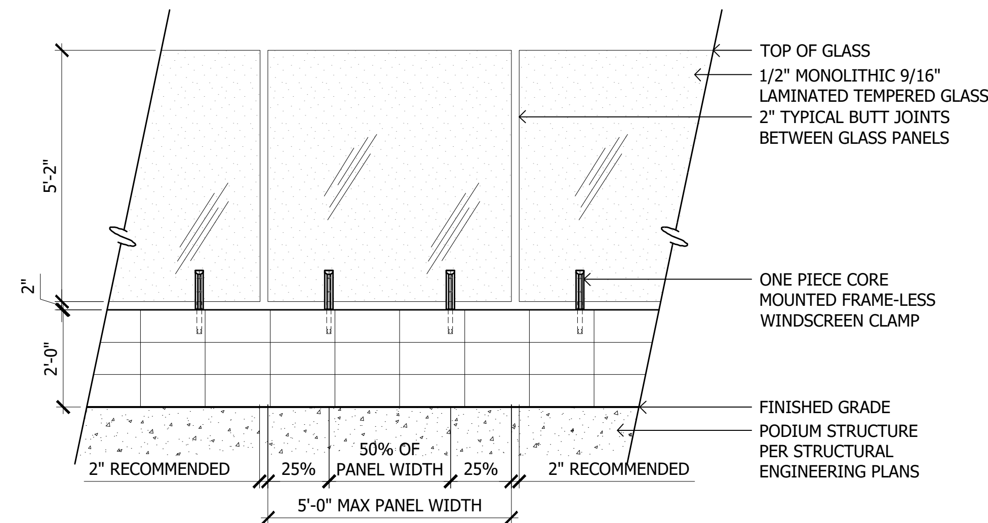
5 Glass Pool Barrier SCALE: 1/2"=1'-0"
