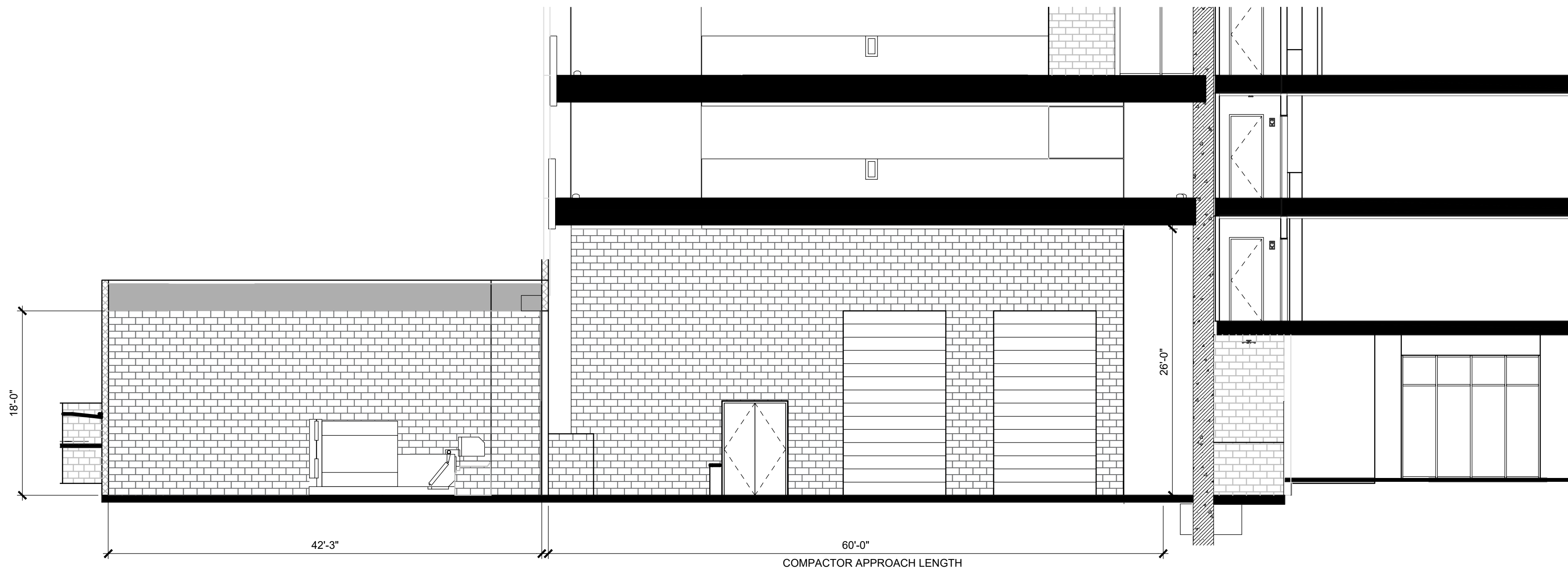
01 COMPACTOR / LOADING AREA E/W SECTION SCALE: 1/8" = 1'-0"
