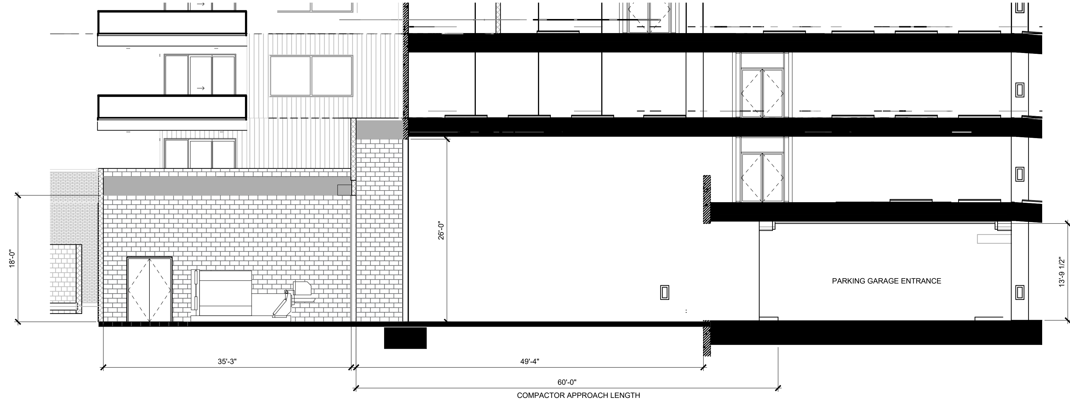
02 COMPACTOR / LOADING AREA N/S SECTION SCALE: 1/8" = 1'-0"
