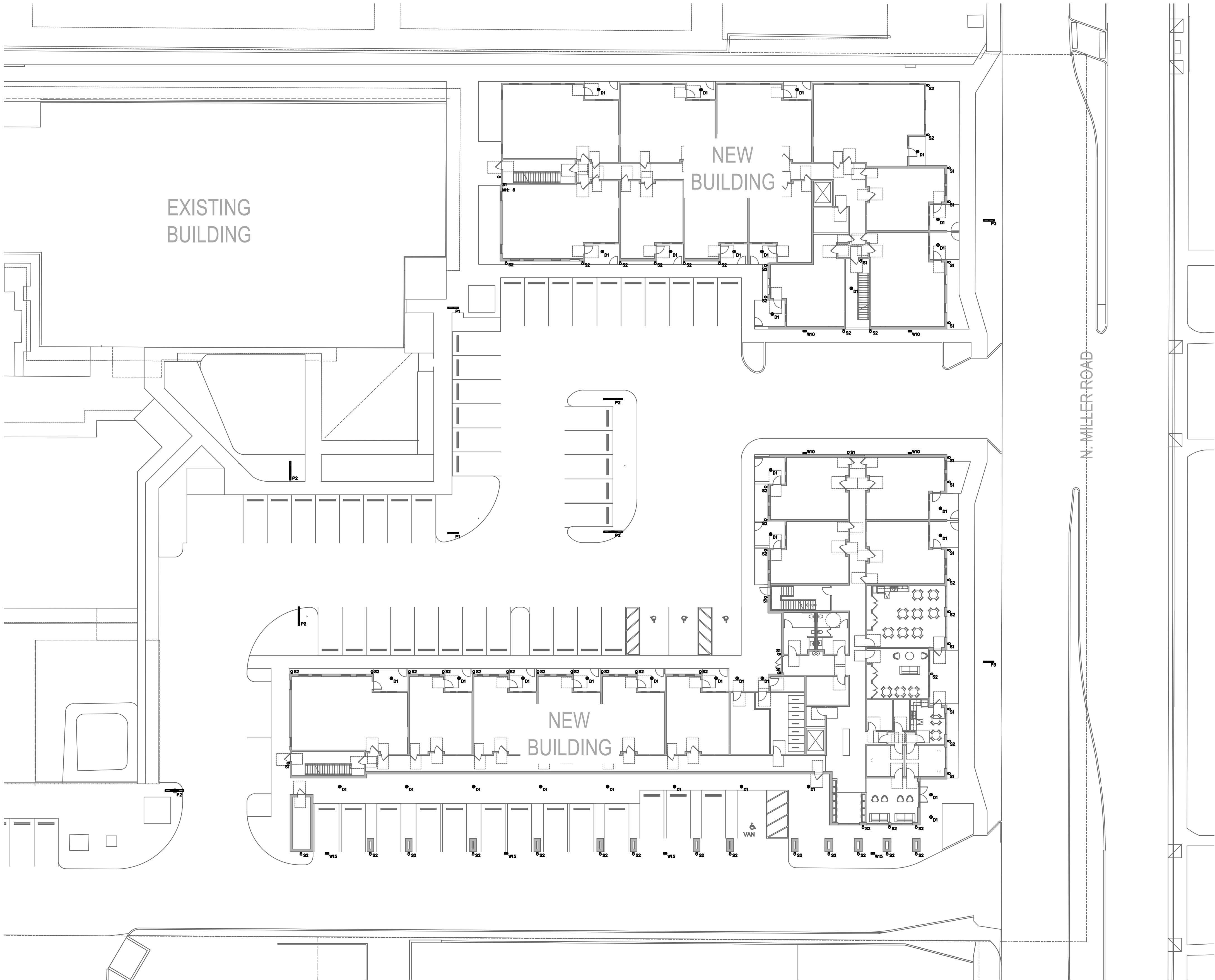
ELECTRICAL LIGHTING PLAN - OVERALL SITE
