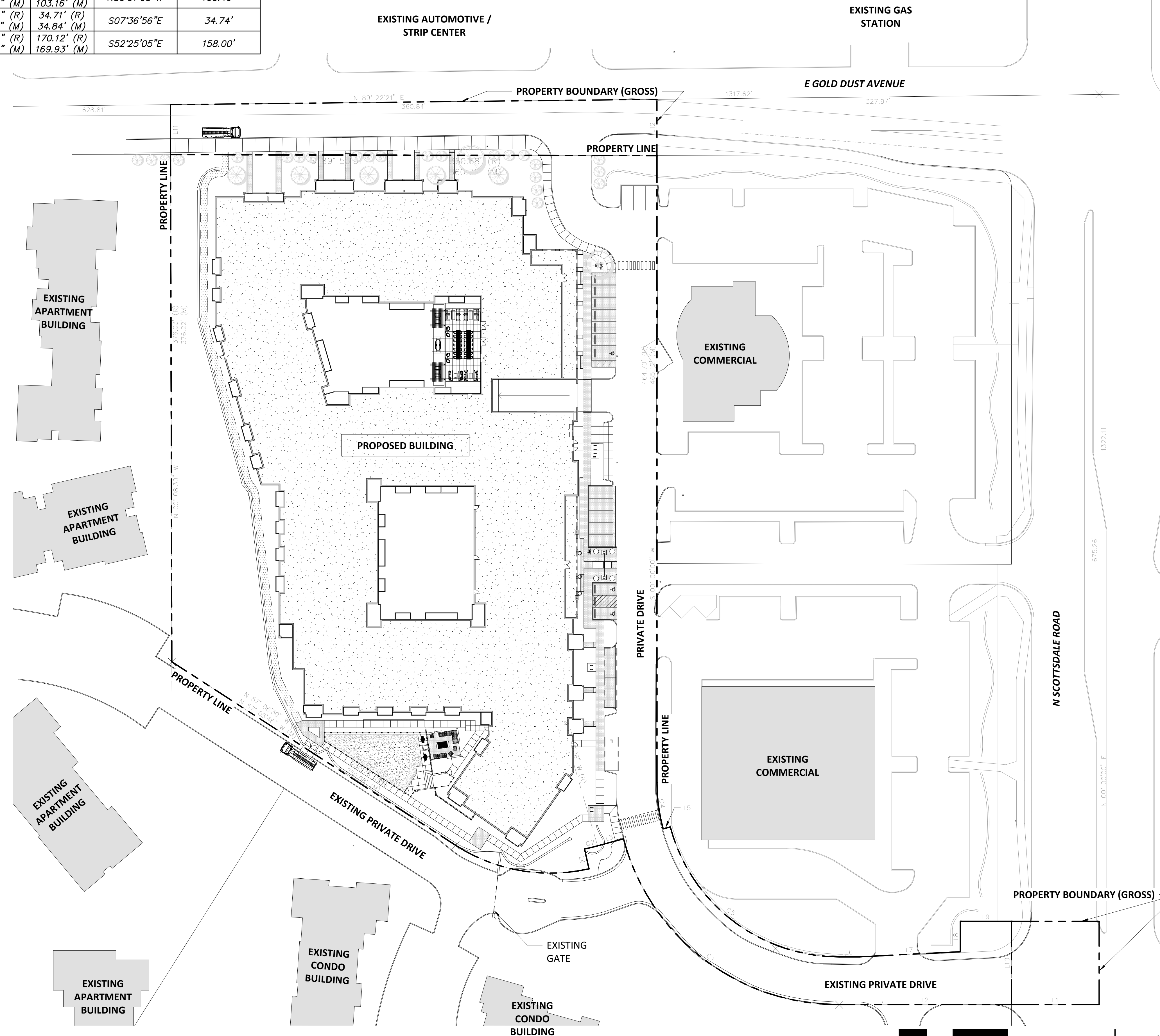
1 DIMENSIONED BOUNDARY PLAN A.d.1 1" = 40'-0"
