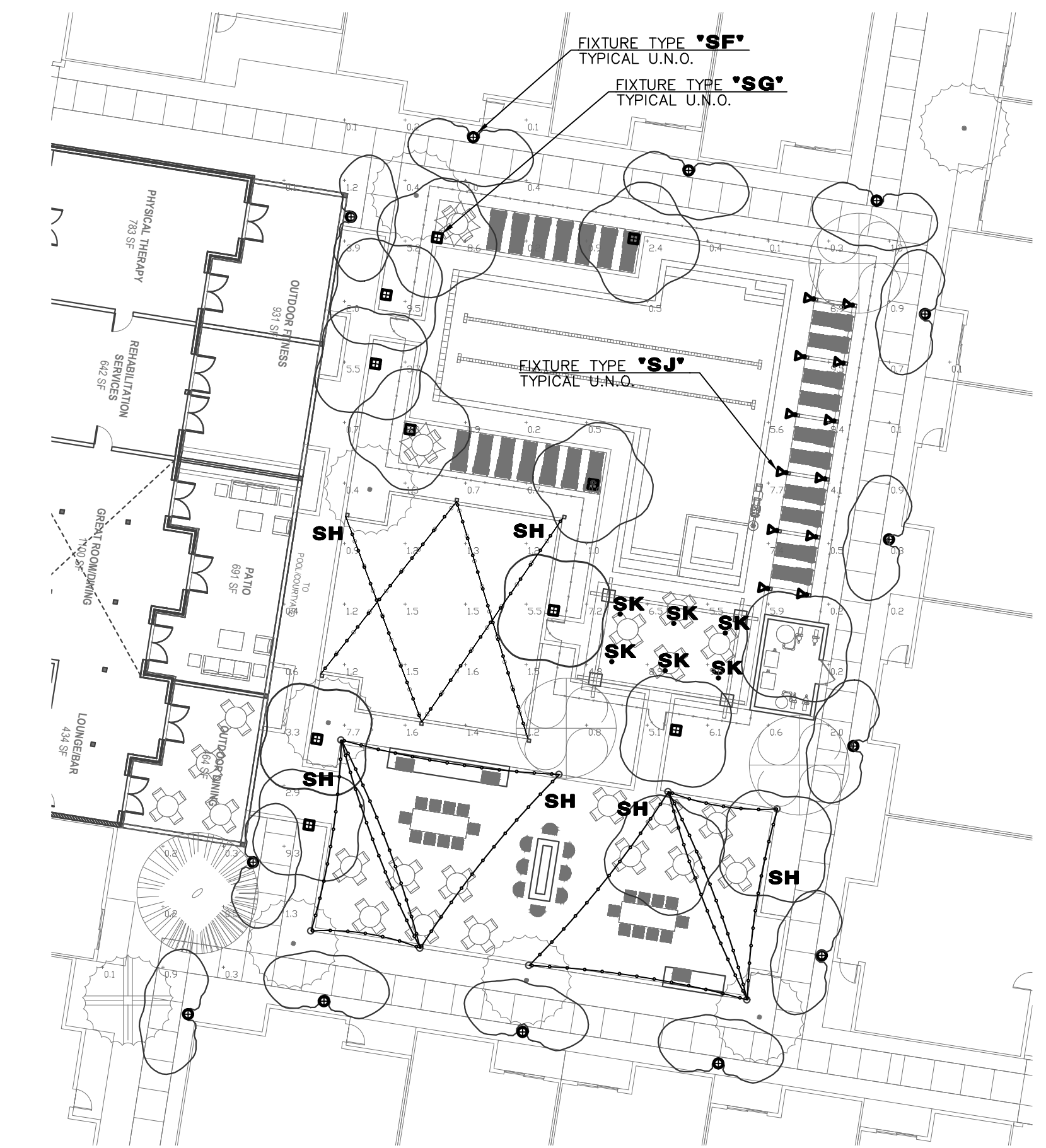
ENLARGED POOL AREA LIGHTING PLAN SCALE: 1" = 20'-0"
