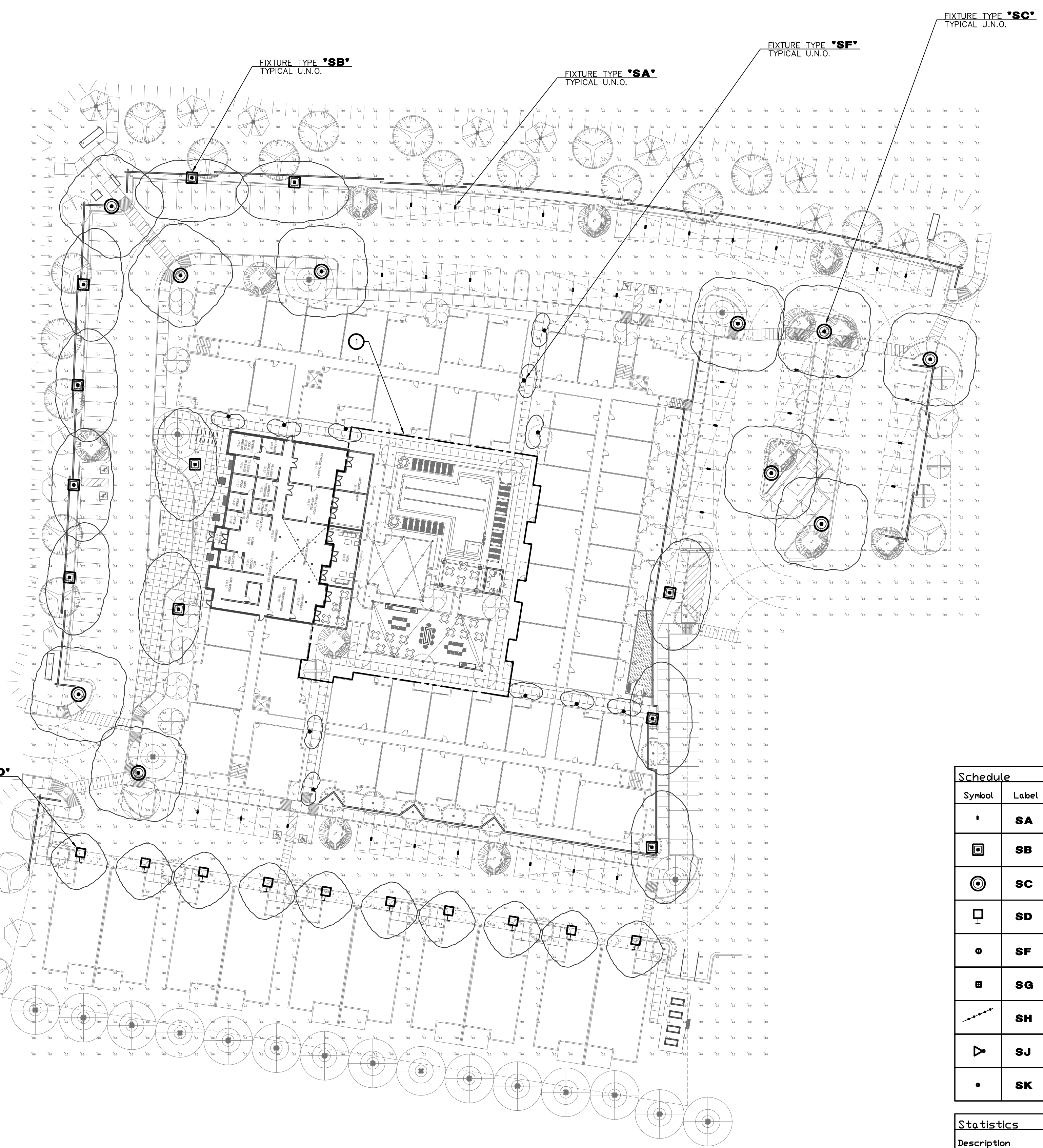
EXTERIOR LIGHTING SITE PLAN SCALE: 1" = 40'-0"
