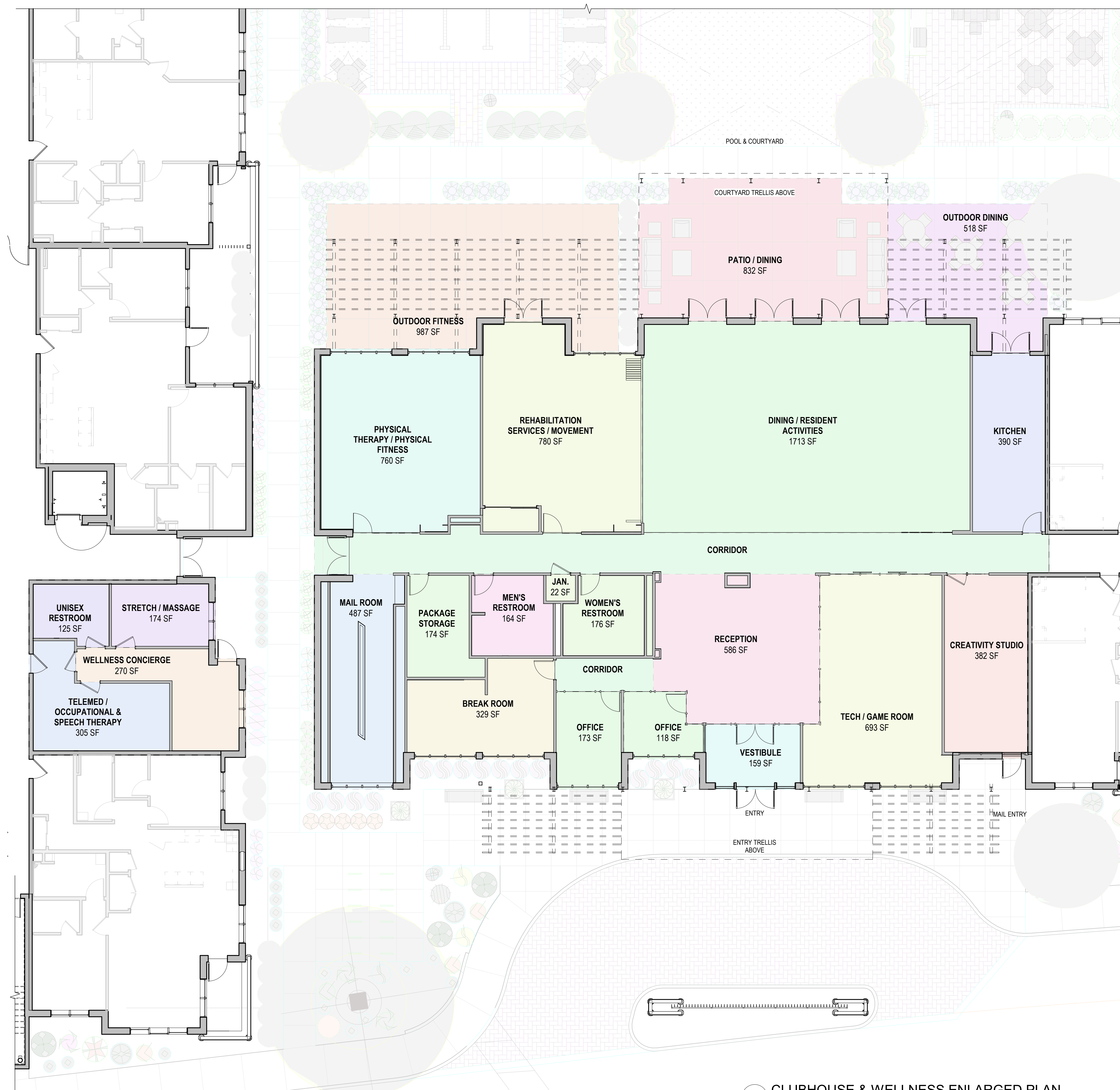
1 CLUBHOUSE & WELLNESS ENLARGED PLAN SCALE: 1/8" = 1'-0"
