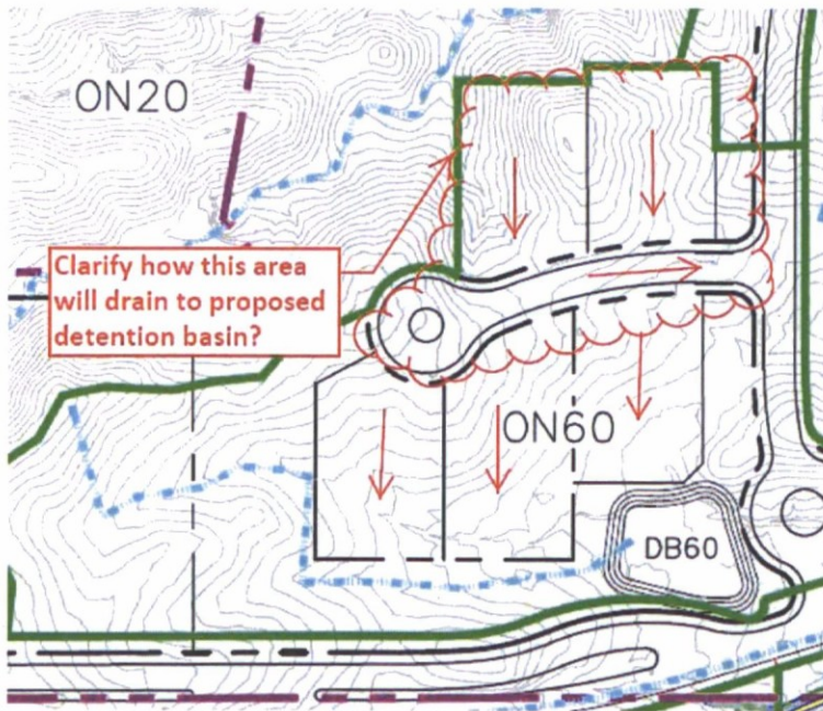
Figure 4. Proposed Drainage Condition.
