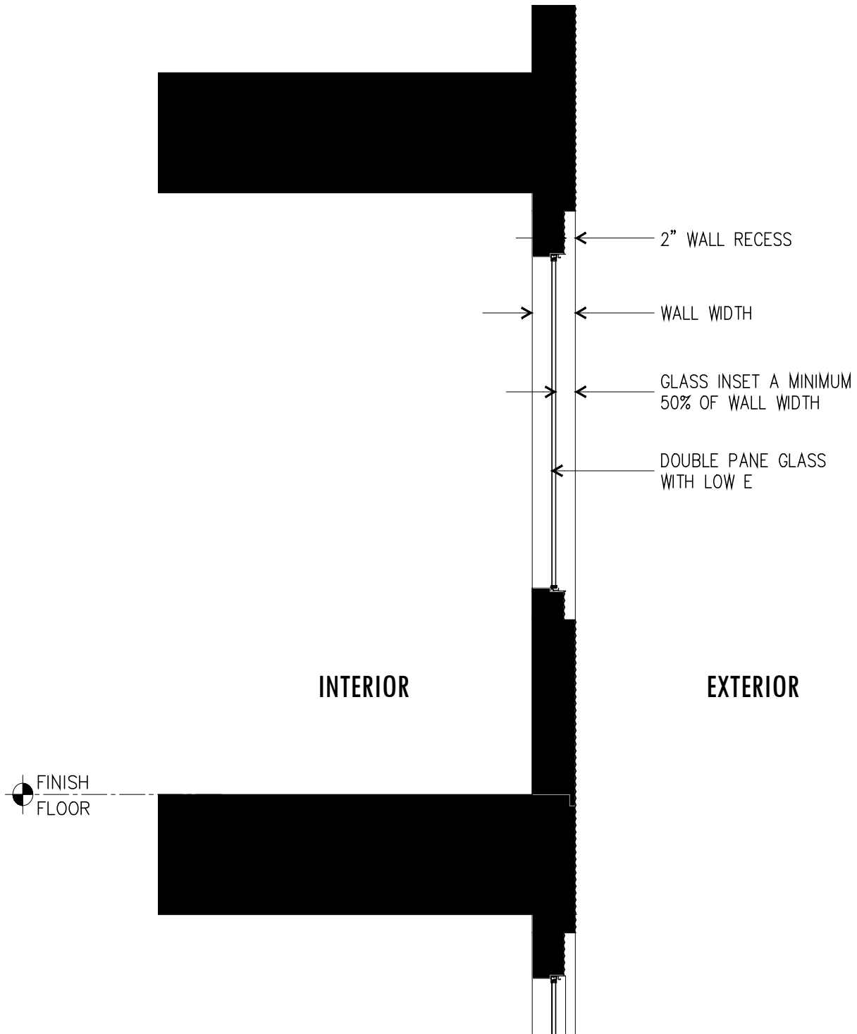
TYPICAL WINDOW RECESS
