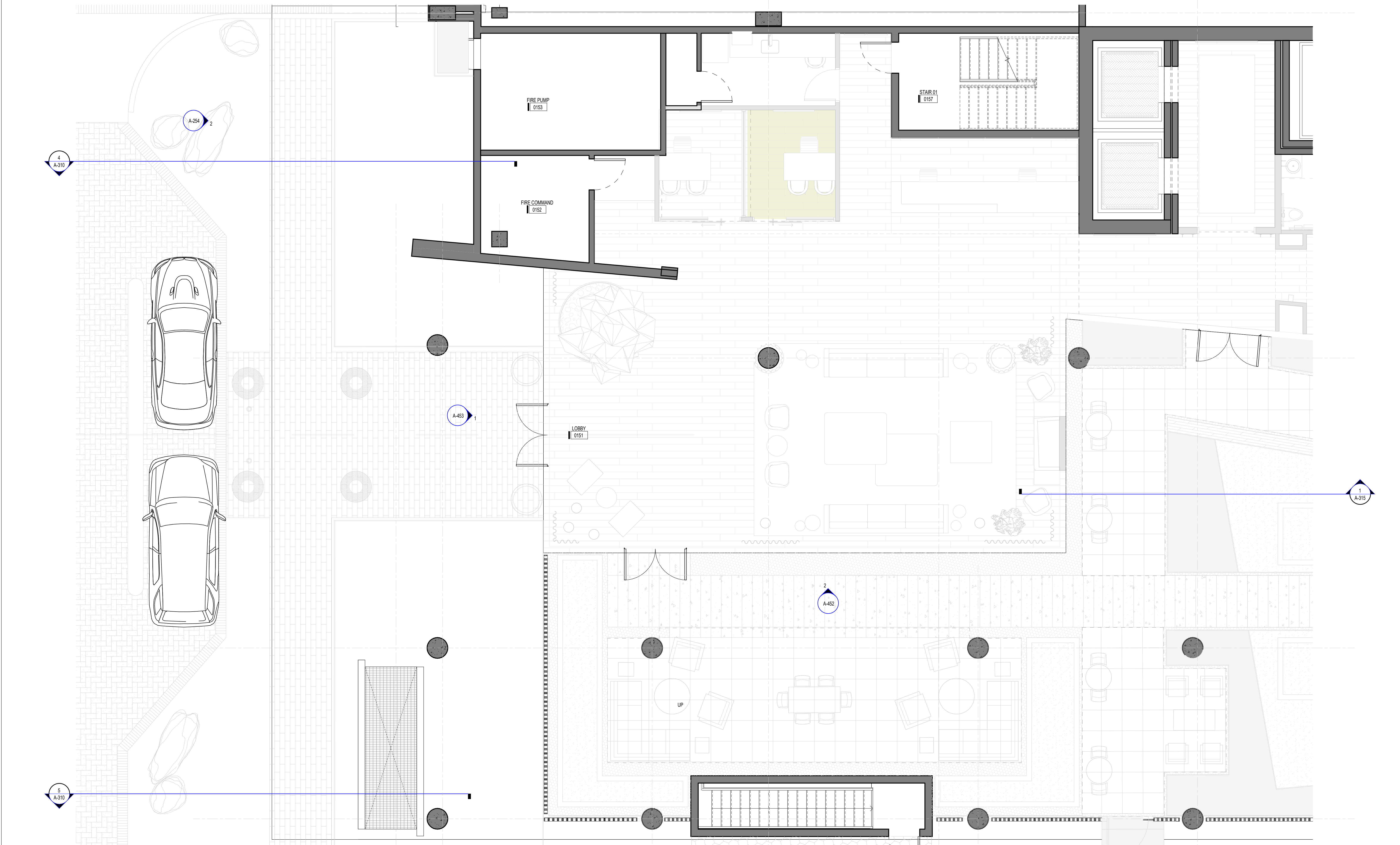
3 ENLARGED PLAN - LOBBY 1/4" = 1'-0"
