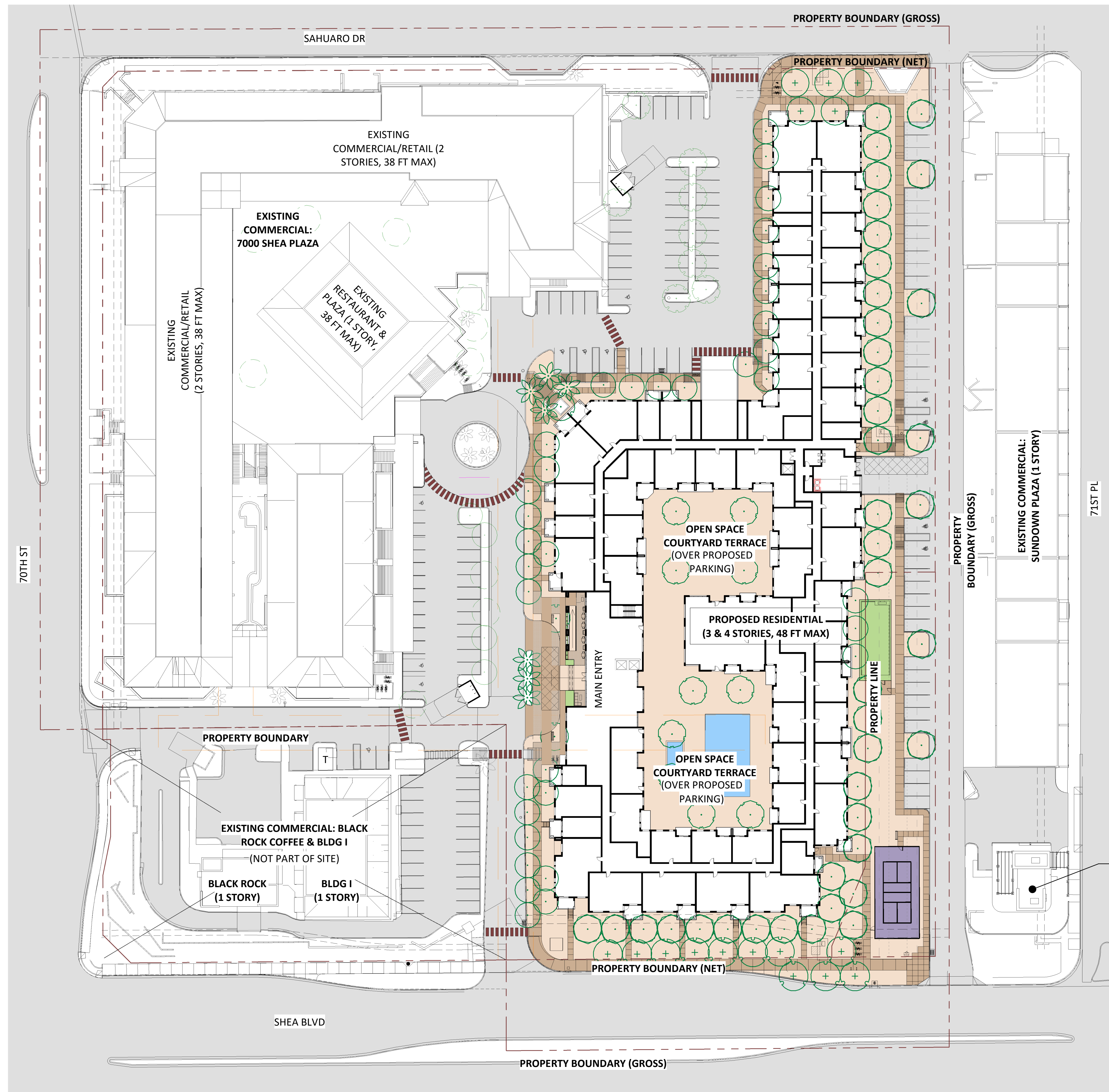
1 SITE PLAN A.21.fa 1" = 40'-0"
